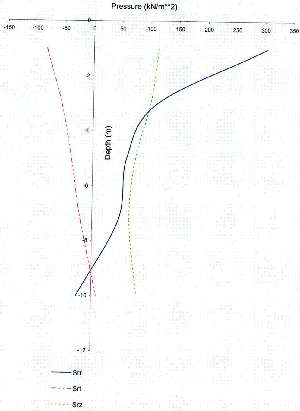
Figure 4.2.1-5 Vertical Distributions of Soil Pressure Computed from the 11.5 m DOB SASSI Model.
