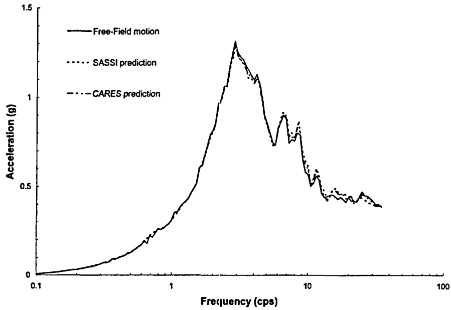
Figure 3.2.2-9 Comparison of Response Spectra for Soil Column C at the Basemat Center of Kinematic Model with 11.5 m Embedment.
