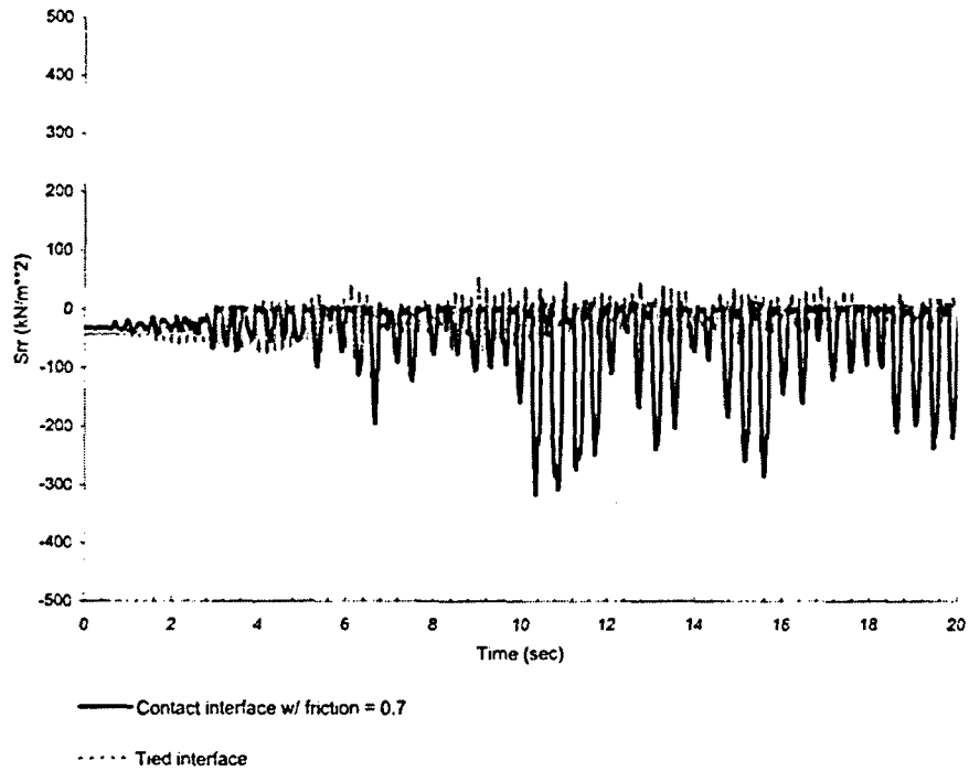
Figure 4.4.1-9 Comparison of Normal Pressure on the Head-on Soil Element near the Mid-height of Structural Wall Computed from the 11.5 m DOB Contact and Tied Interface Models.
