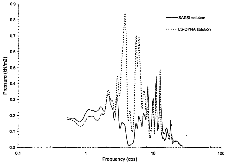
Figure 4.3.5-14 Fourier Spectra of Soil Pressure Computed at the Head-on Soil Element near Mid-Height Embedded Wall for the 46 m DOB LD-DYNA model.
