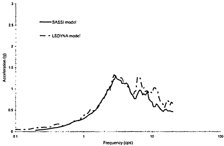
Figure 4.3.5-5 Comparison of Response Spectra at the Roof for the 46 m Embedment.
