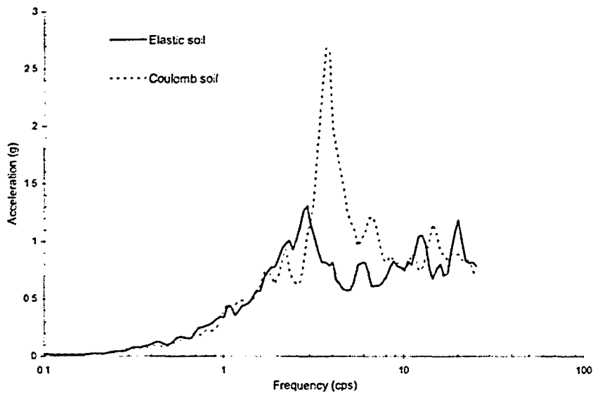
Figure 4.5-5 Effect of Soil Material Models on the Contact Interface LS-DYNA Response Spectra (5% Damping) at Structural Base with Butterworth Low-Pass High Cut Filter ( f_{cutoff} = 20 Hz).
