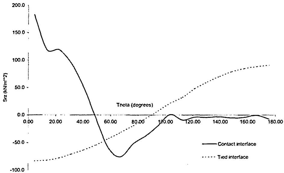
Figure 4.4.1-10 Comparison of Circumferential Distributions of Vertical Shear Computed from the 11.5 m DOB Contact and Tied Interface Models at Respective Mid-Height Peak S_r Times.
