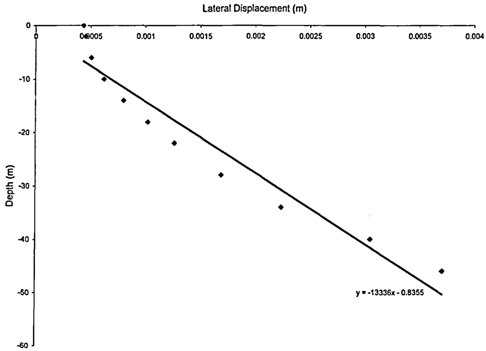
Figure 4.2.4-6 Lateral Wall Displacements Computed from the 46 m DOB SASSI Model.
