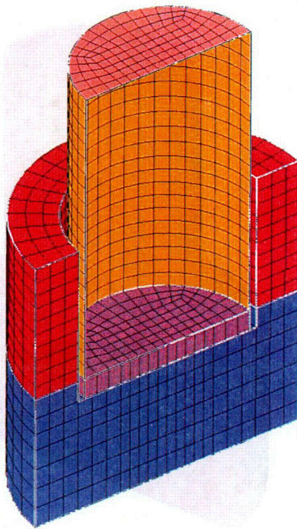
Figure 4.1.2-3 LS-DYNA Model for the 23 m Embedment.
