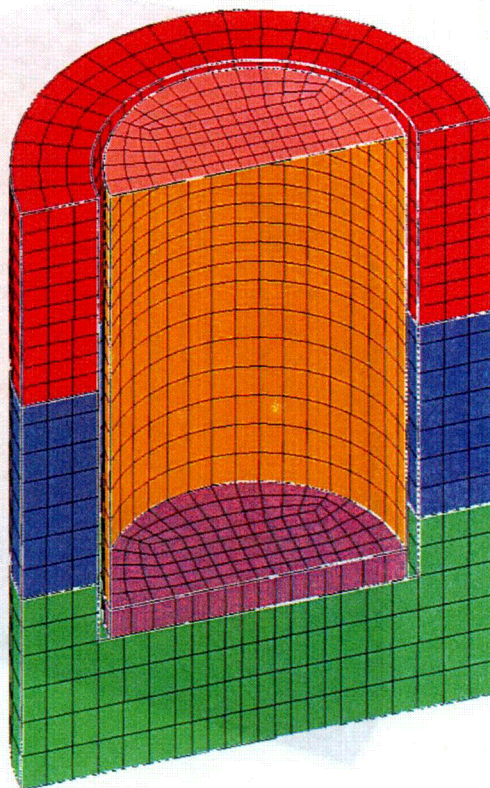
Figure 4.1.2-8 Zoom-in View of the Structure and Surrounding Soil in LS-DYNA Model for the 46 m Embedment.
