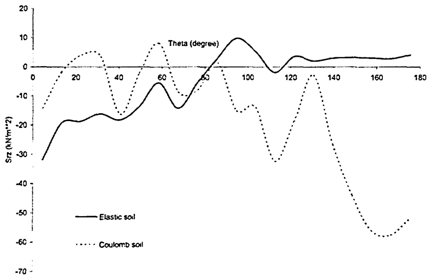
Figure 4.5-17 Effect of Soil Material Models on Circumferential Distribution of Vertical Shear Computed from the 23 m DOB Contact Interface LS-DYNA Model at Respective Mid-Height Peak S_{r\theta} Times.
