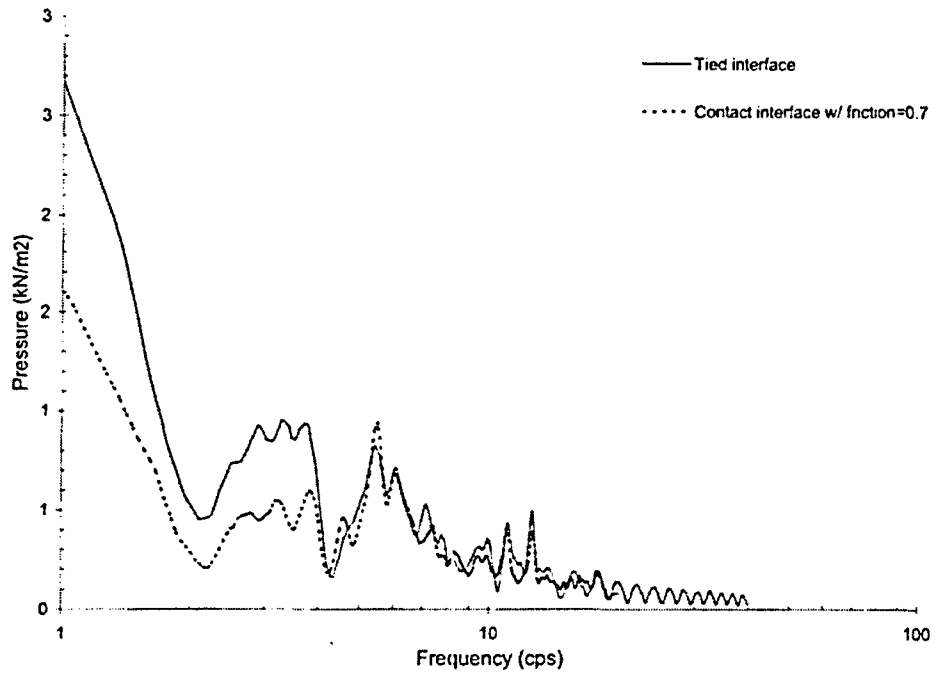
Figure 4.4.5-4 Smoothed Fourier Spectra of Soil Pressure in the Head-on Soil Element near the Mid-Height Wall Section for DOB = 46 m.
