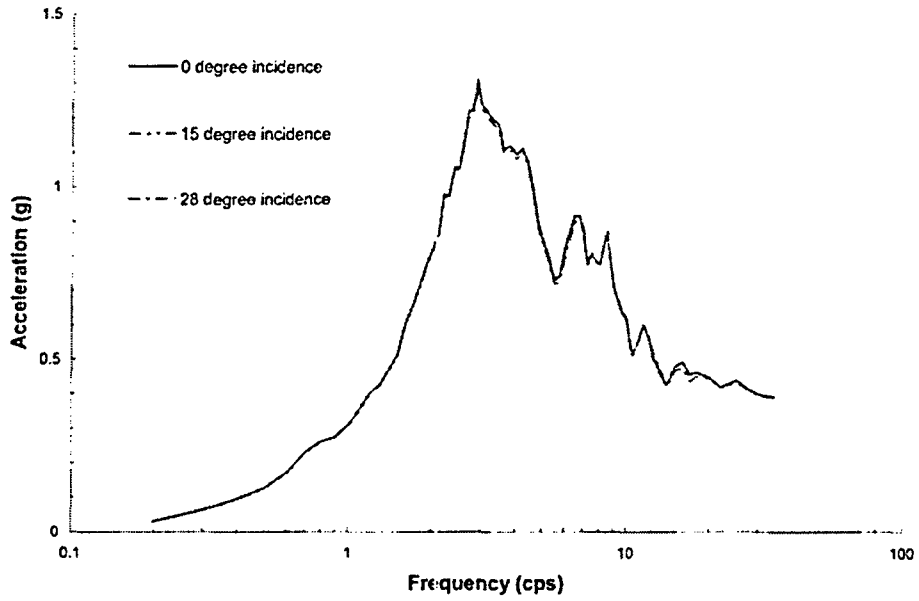
Figure 3.2.1-33 Translational Spectra for Soil Column C at the Basemat Center of SASSI Kinematic Model with 11.5 m Embedment for Various Incident SV-Waves.
