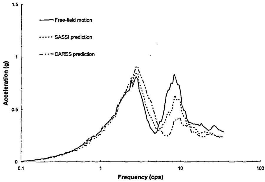
Figure 3.2.2-15 Comparison of Response Spectra for Soil Column C at the Basemat Center of Kinematic Model with 46 m Embedment.
