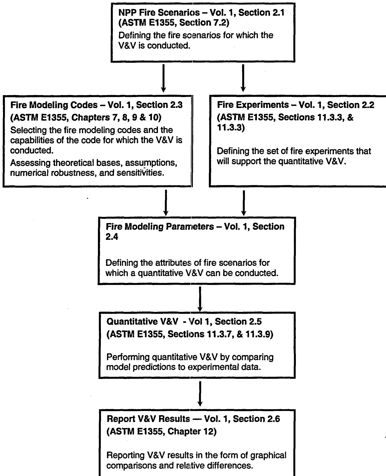
Figure 2-1: Overview of the Approach for V&V Study of Selected Fire Models for Nuclear Power Plant Application
