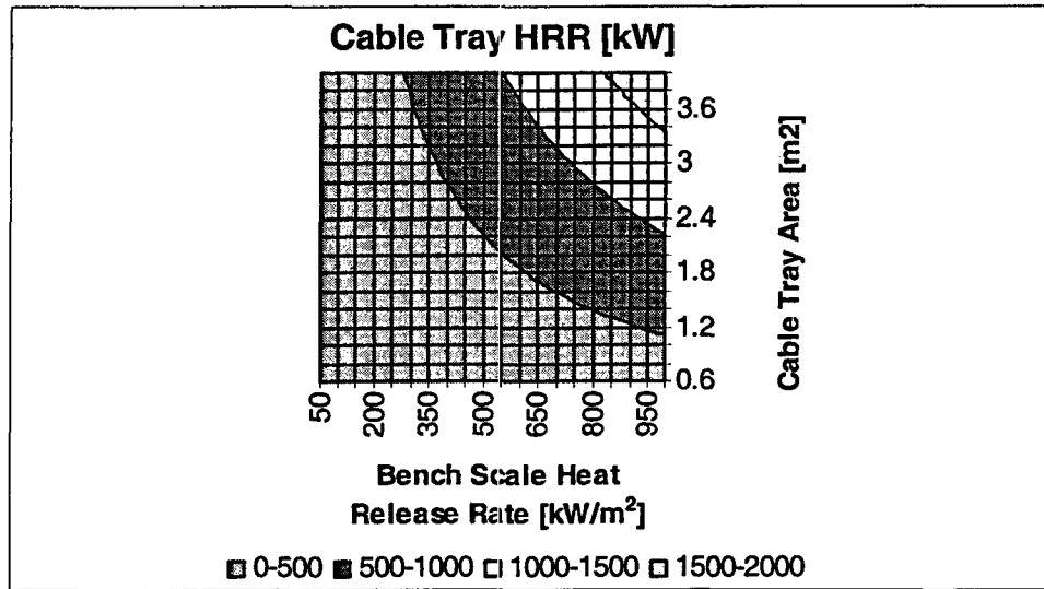
Figure 5-12: Sensitivity Analysis for the Model Used To Predict the Heat Release Rate from Cable Tray Fires
