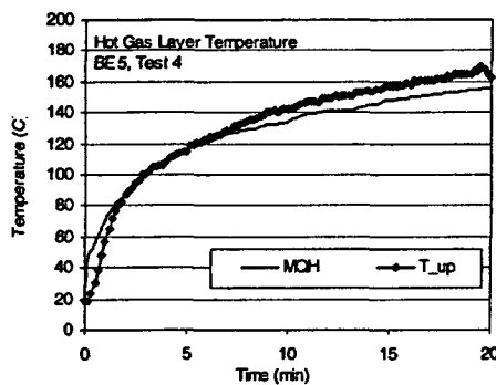
Figure A-8: Hot Gas Layer (HGL) Temperature and Height, ICFMP BE #5, Test 4.
