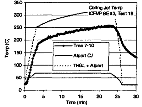
Figure A-13: Near-ceiling gas (ceiling jet) temperatures, ICFMP BE #3, open door tests
