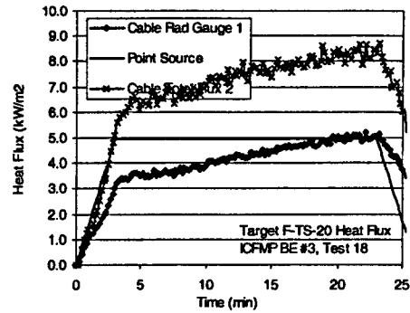
Figure A-29: Radiative heat flux to cable F
