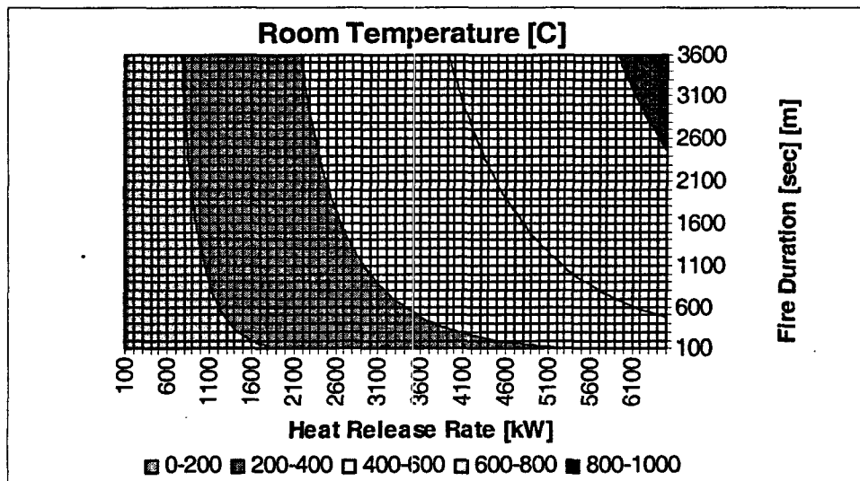
Figure 5-9: Sensitivity Analysis for the FPA Model for Room Temperature
