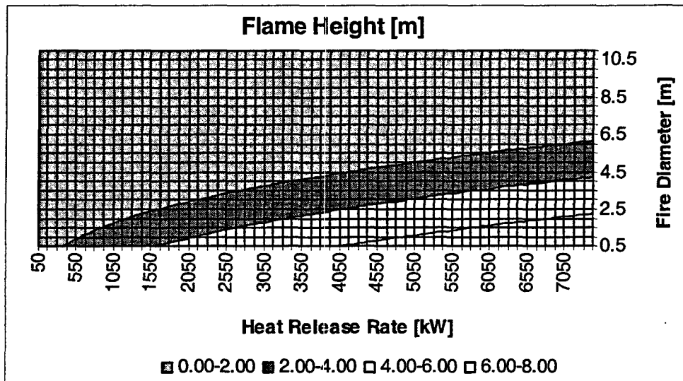
Figure 5-2: Sensitivity Analysis for Heskestad's Model for Flame Height
