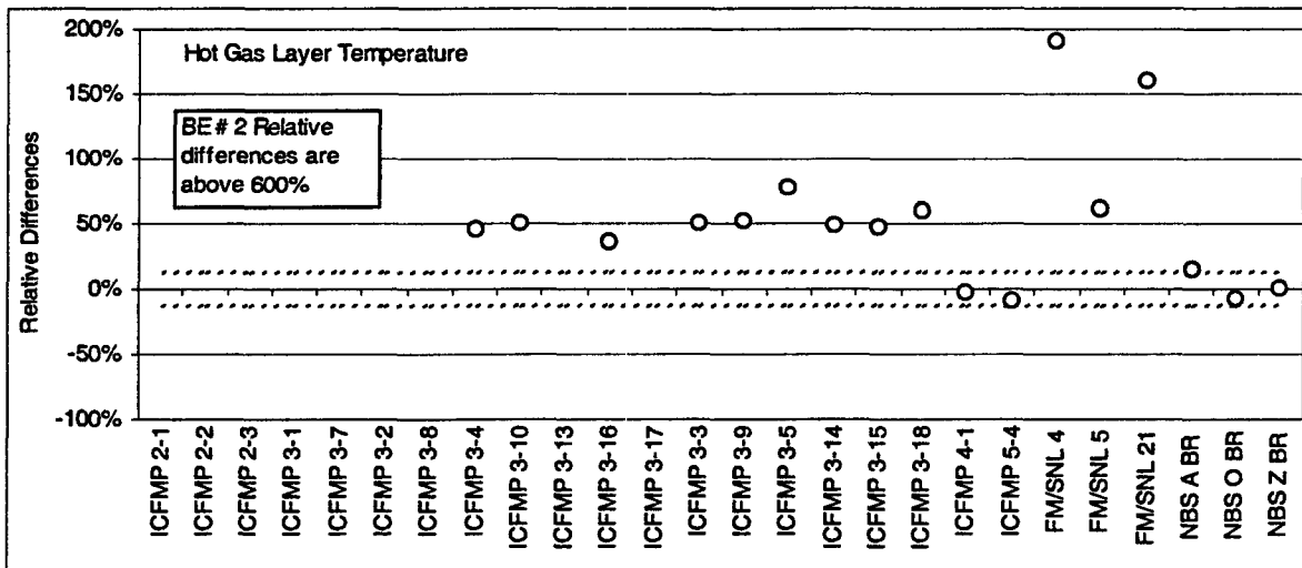
Figure 6-1: Scatter plot of relative differences for hot gas layer temperature for ICFMP BE #2, 3, 4, 5, and the selected FM/SNL and NBS Tests
