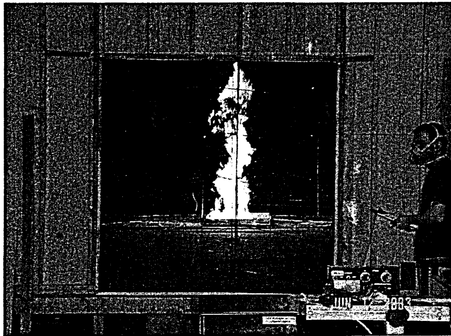
Figure A-21: Photograph and simulation of ICFMP BE #3, Test 3, as seen through the 2 m by 2 m doorway. Photo courtesy of Francisco Joglar, SAIC.
