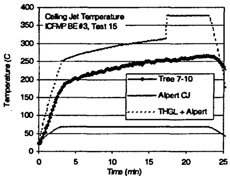
Figure A-13: Near-ceiling gas (ceiling jet) temperatures, ICFMP BE #3, open door tests
