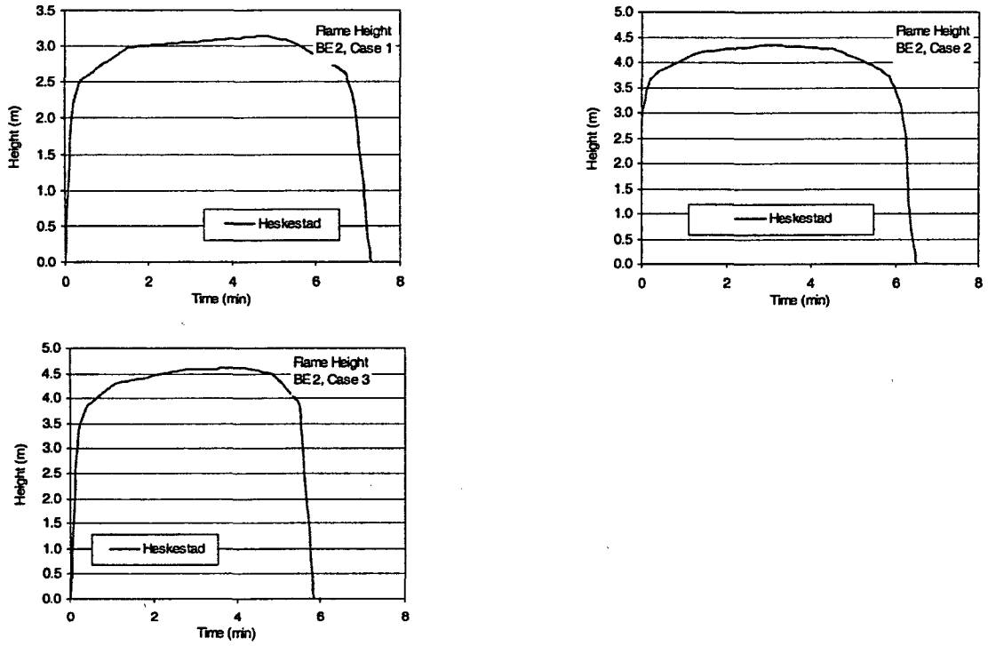
Figure A-19: Flame heights for ICFMP BE # 2
