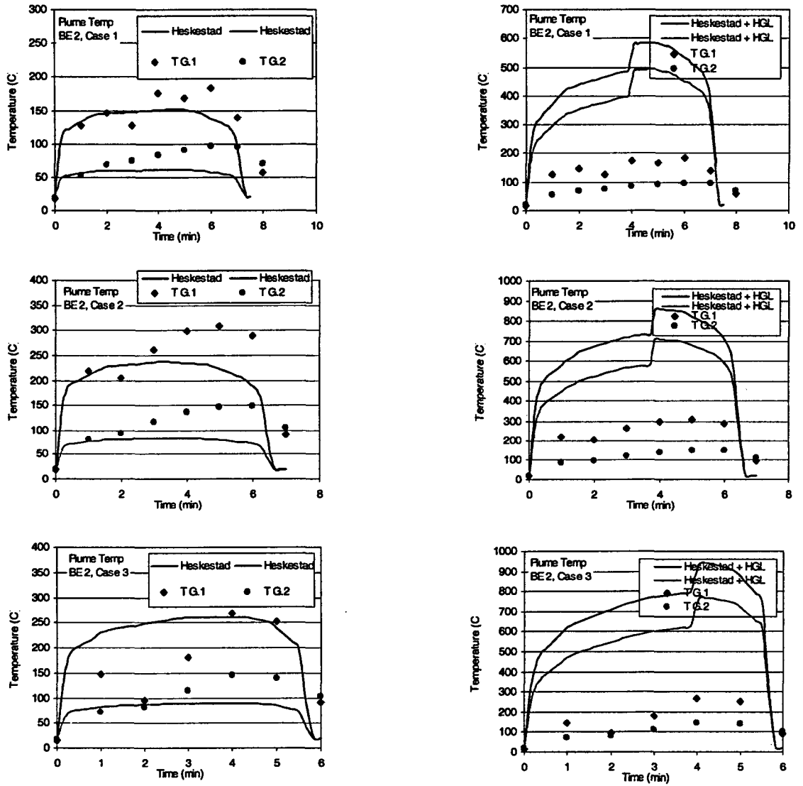
Figure A-16: Near-celling gas temperatures, FM/SNL Series, Sectors 1 and 3 compared with Heskestad's plume temperature correlation.
