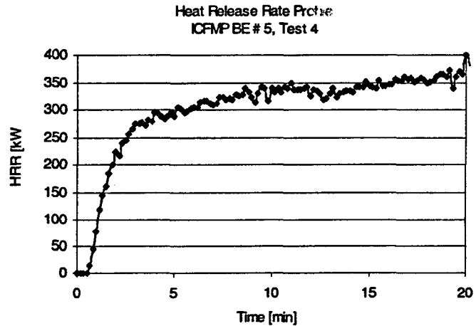
Figure A-7: Heat release rate profile for ICFMP BE #5.
