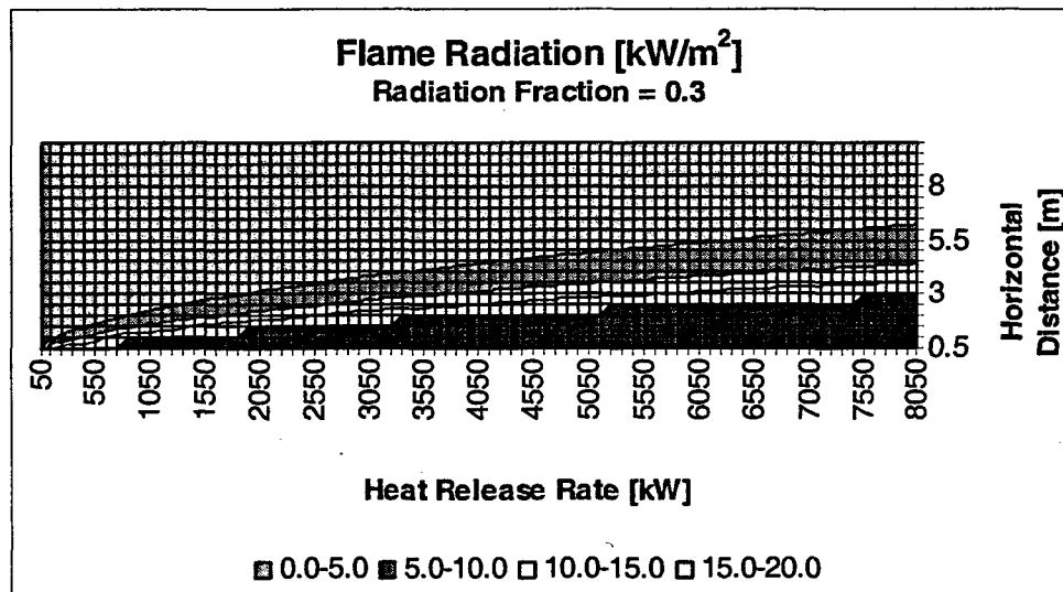
Figure 5-1: Sensitivity Analysis for the Point Source Radiation Model
