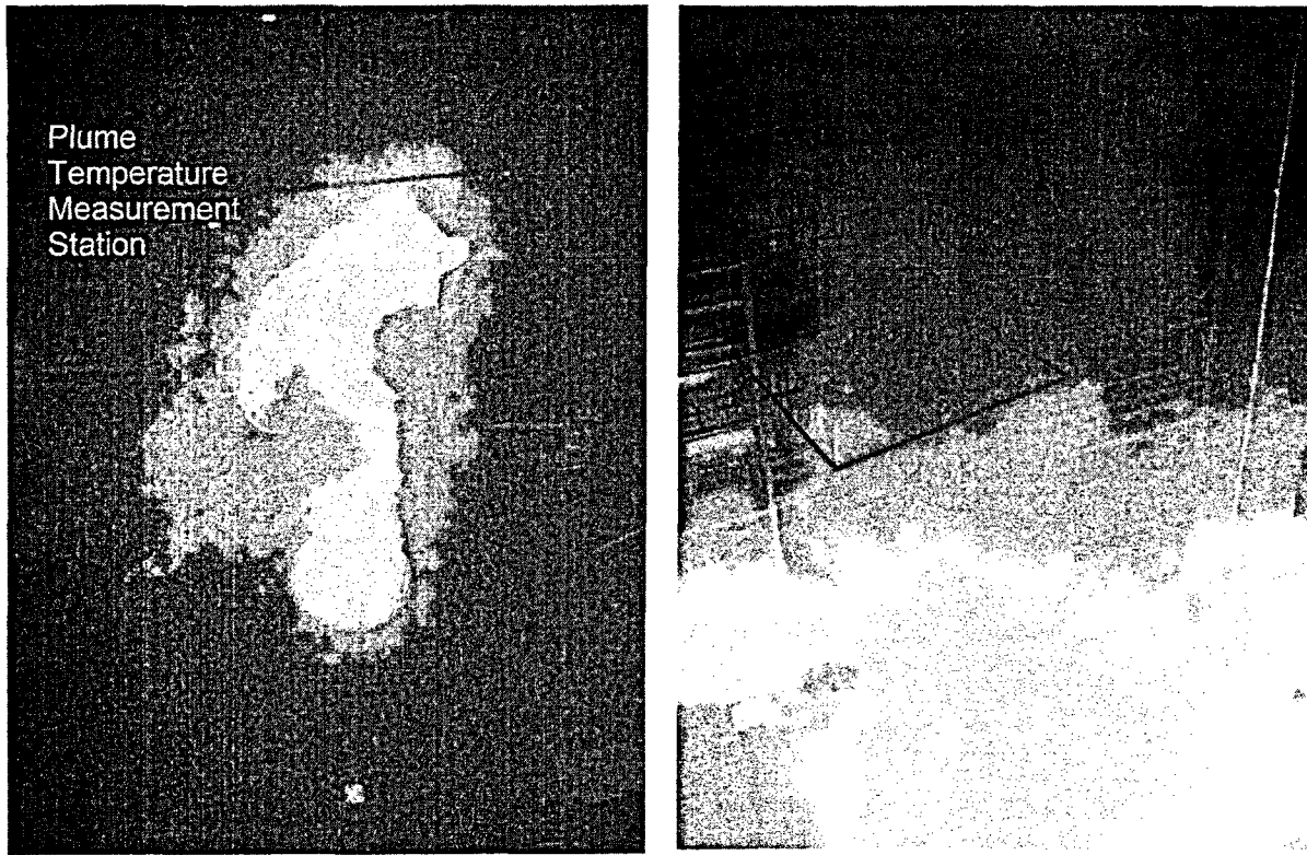
Figure A-15: Fire plumes in ICFMP BE #2. Courtesy Simo Hostikka, VTT Building and Transport, Espoo, Finland.
