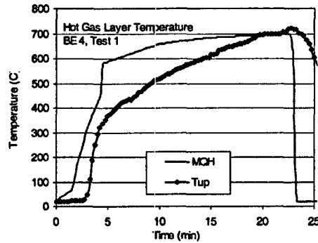
Figure A-6: Hot Gas Layer (HGL) Temperature and Height, ICFMP BE #4, Test 1.
