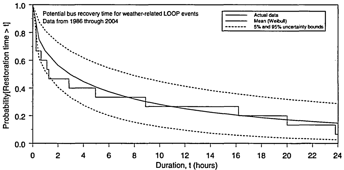
Figure C-4. Weibull fit for weather-related LOOP durations.
