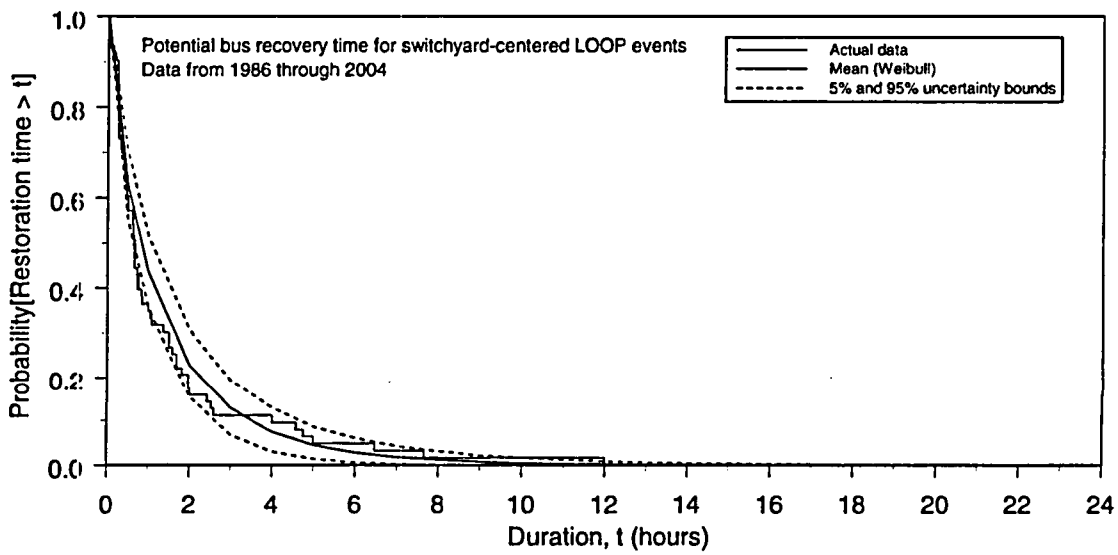
Figure C-2. Weibull fit for switchyard-centered LOOP durations.
