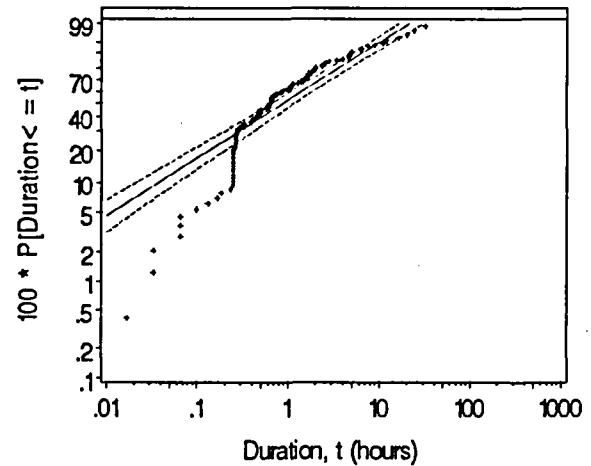
Figure B-2. Weibull fit for overall LOOP data.
