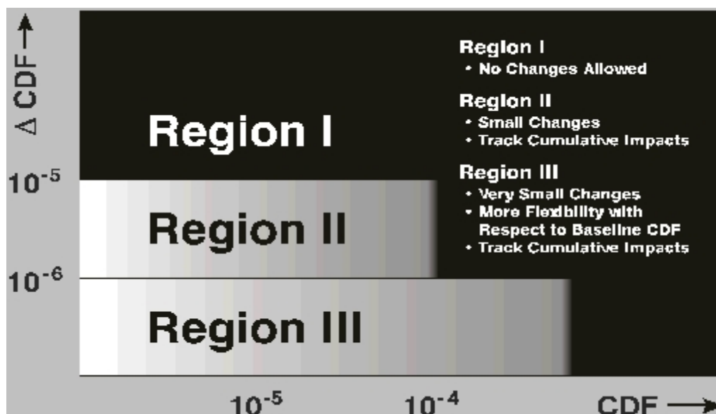
Figure 5-2 – \Delta CDF Acceptance Criteria
