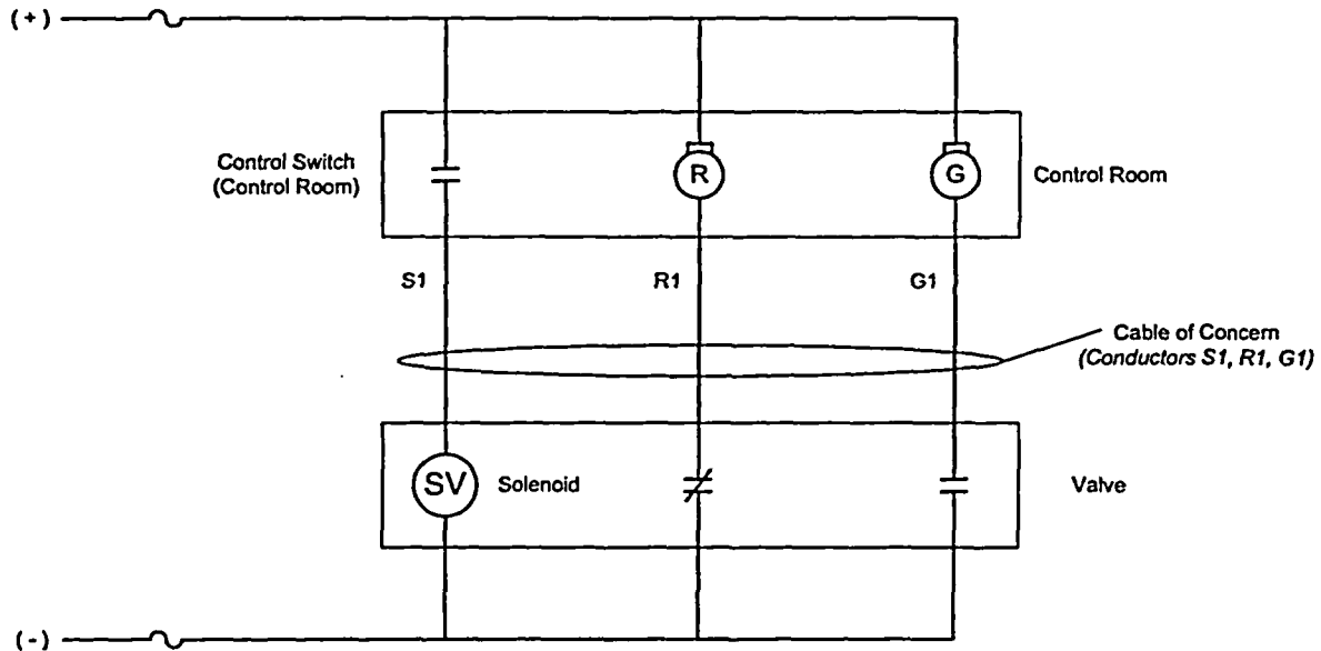
Figure I-14 Simple SOV Circuit with Alternate Contact Arrangement
