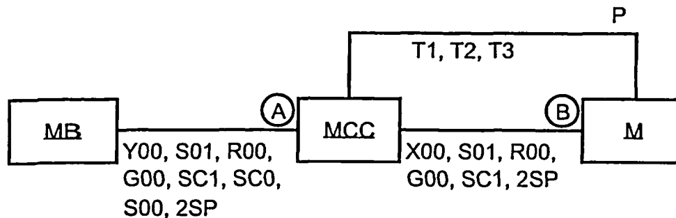
Figure K-3 Highlighted Block Diagram for Typical MOV Circuit Example
