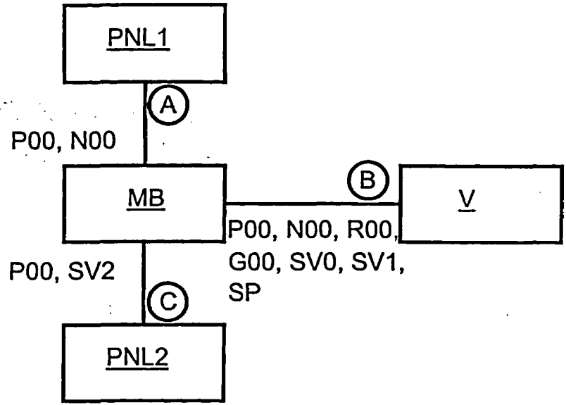
Figure K-1 Highlighted Block Diagram for Typical SOV Circuit Example
