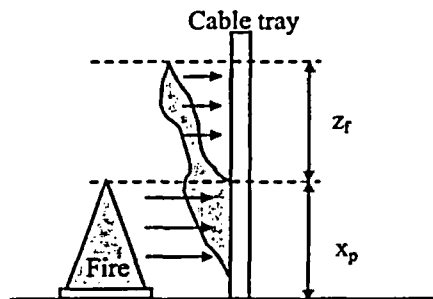
Figure R-4 Pictorial Representation of the Beginning of the Flame Spread Process
