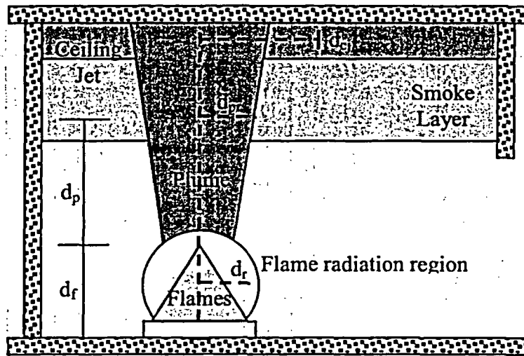
Figure F-2 Fire ZOI. d_p : Critical Distance for Targets in the Plume, d_p : Radius of the Plume at the Critical Distance, d_f : Flame Height, d_{c_j} : Critical Distance for Targets in the Ceiling Jet, d_r : Critical Distance for Targets Subjected to Flame Radiation
