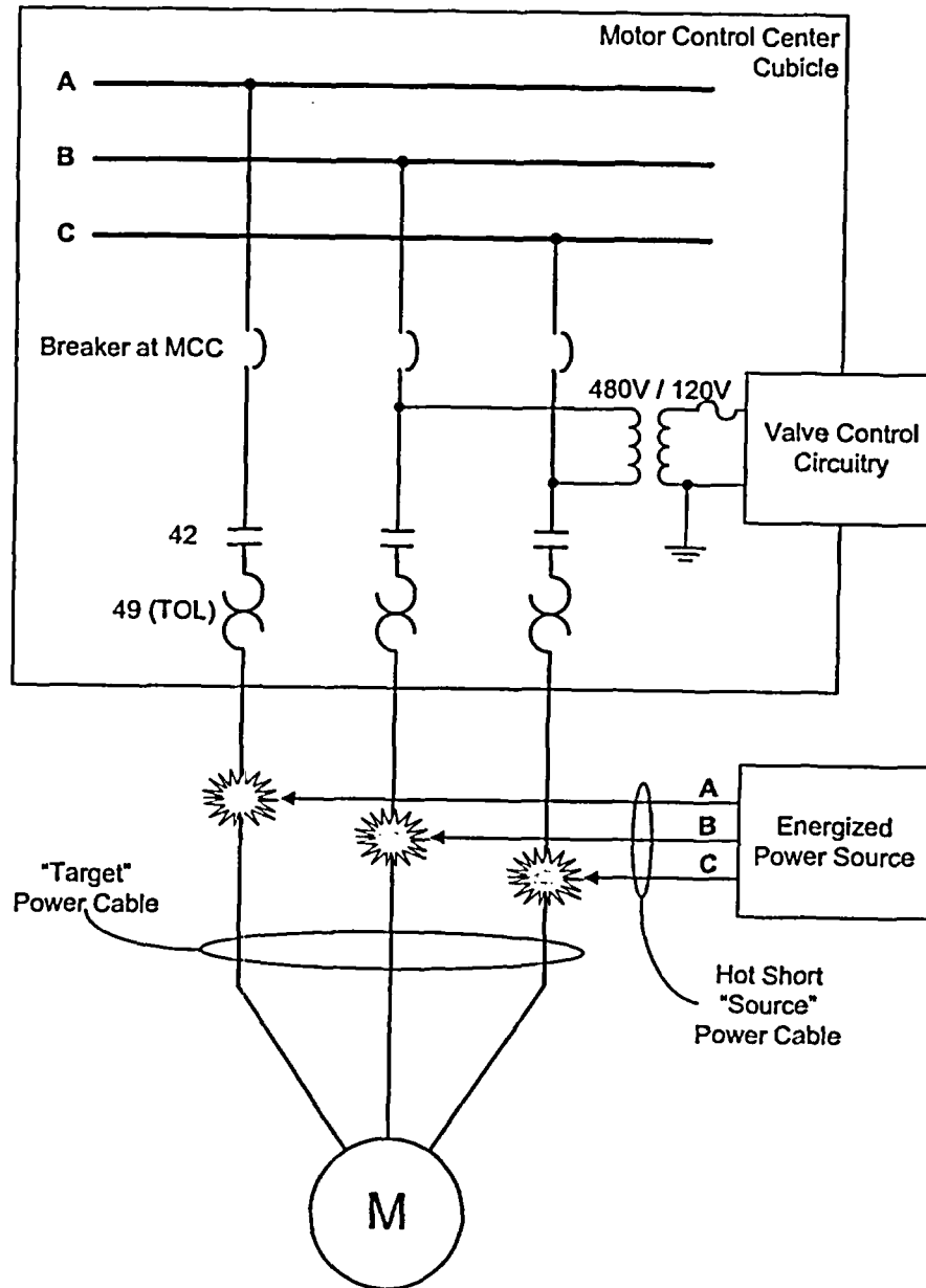
Figure I-13 Ungrounded Three-Phase Motor Power Supply
