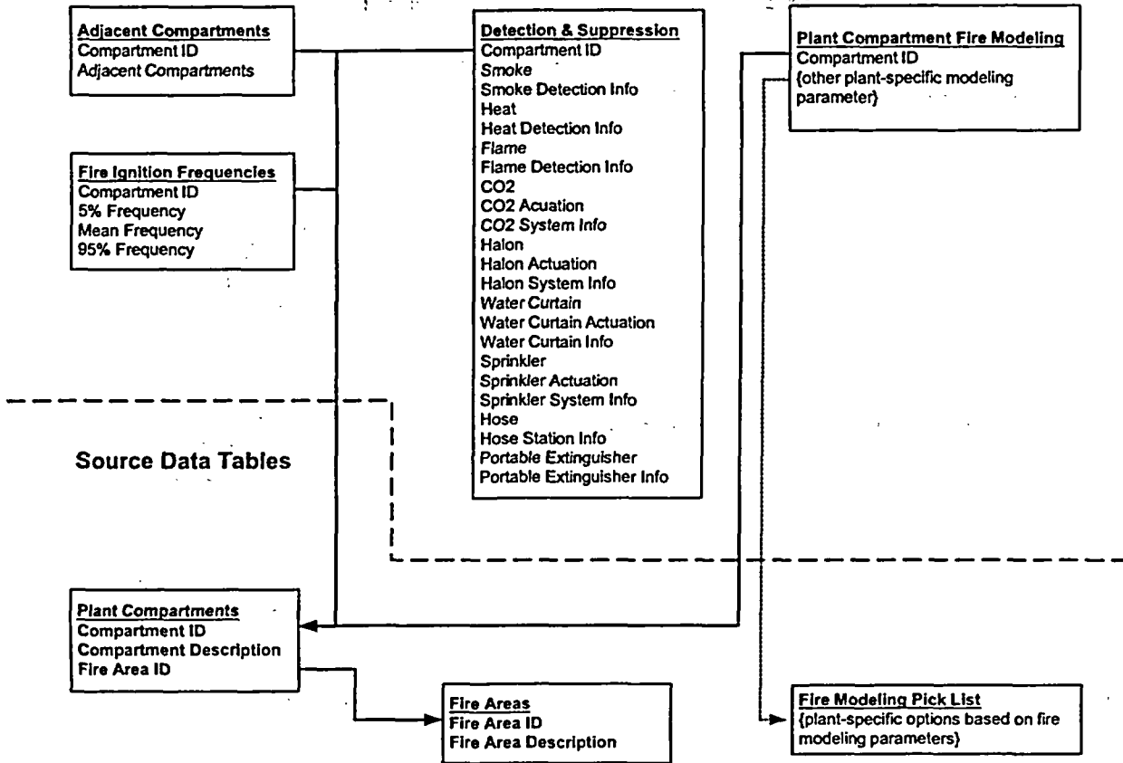
Figure W-2 Fire PRA Database Structure—Compartment, Areas, and Fire Protection
