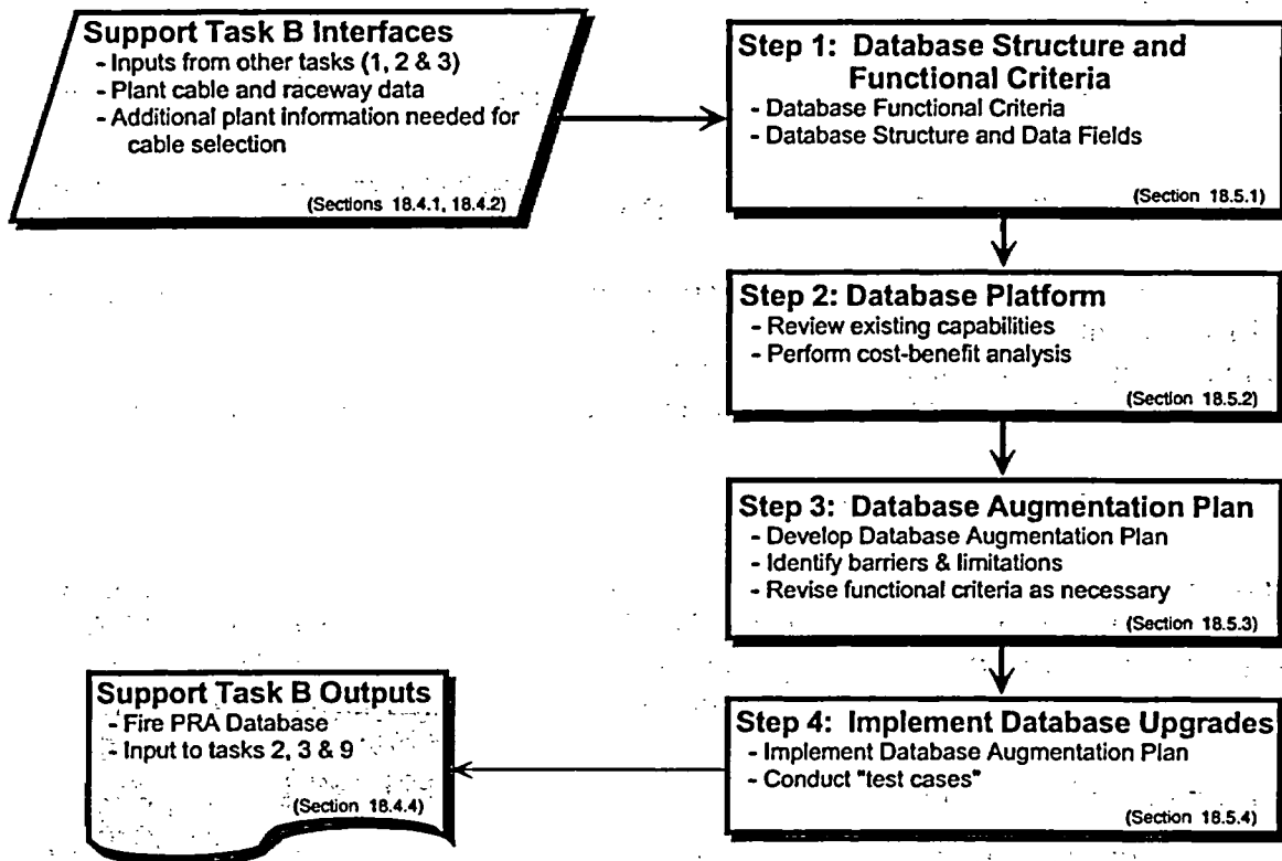
Figure 18-1 Fire PRA Database Structure—Equipment and Cables
