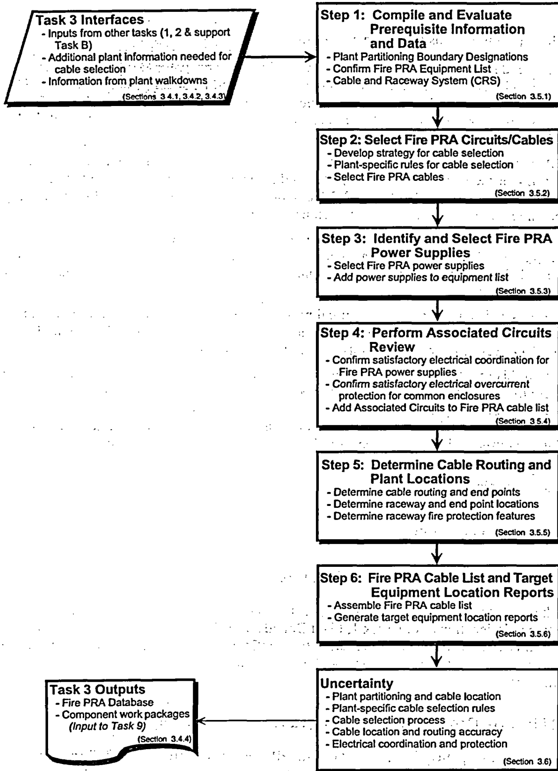
Figure 3-1 Fire PRA Cable Selection Process
