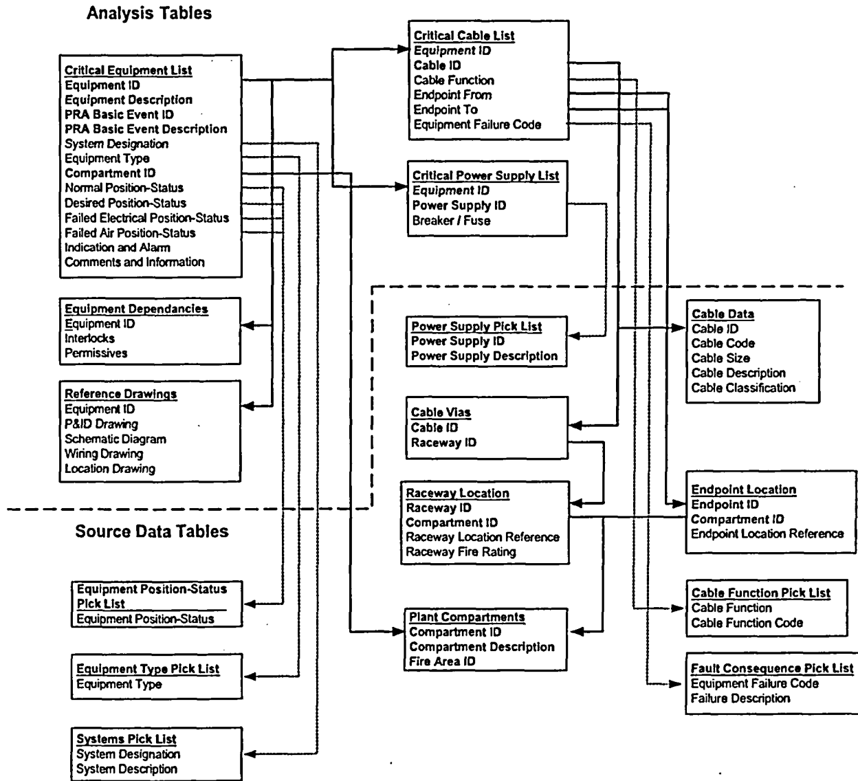
Figure W-1 Fire PRA Database Structure—Equipment and Cables
