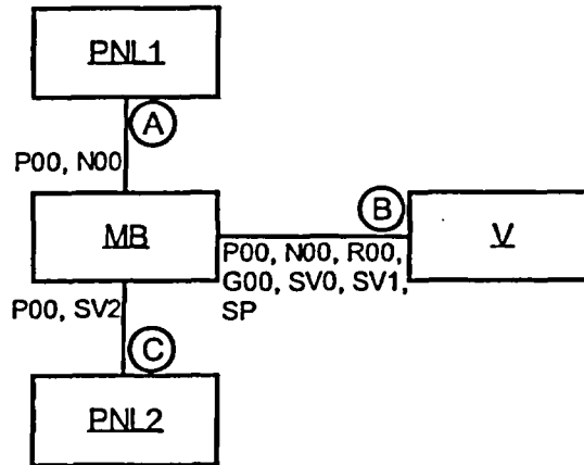
Figure I-1 Block Diagram for Typical SOV Circuit Analysis Example
