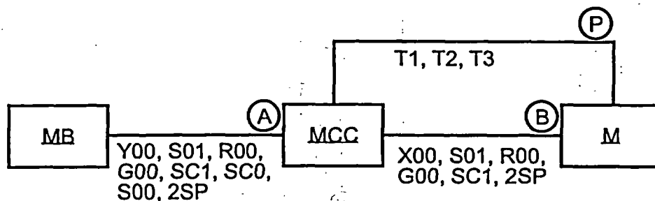
Figure I-3 Block Diagram for Typical MOV Circuit Analysis Example
