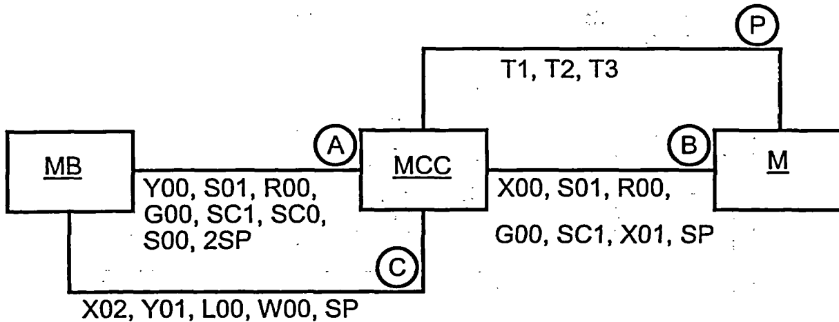
Figure K-11 Highlighted Block Diagram for MOV with Independent Control Circuits Example
