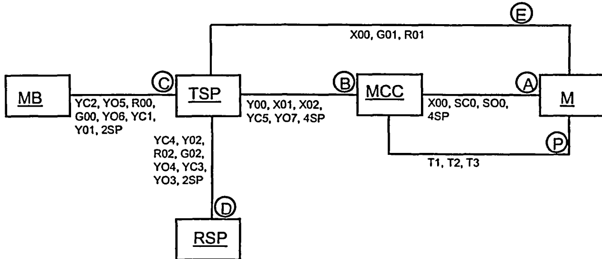
Figure K-7 Highlighted Block Diagram for Ungrounded, Inverted MOV Example
