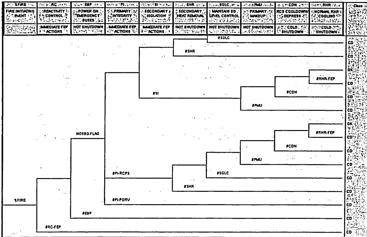
Figure 5-1 Illustration of a FEP Response Model
