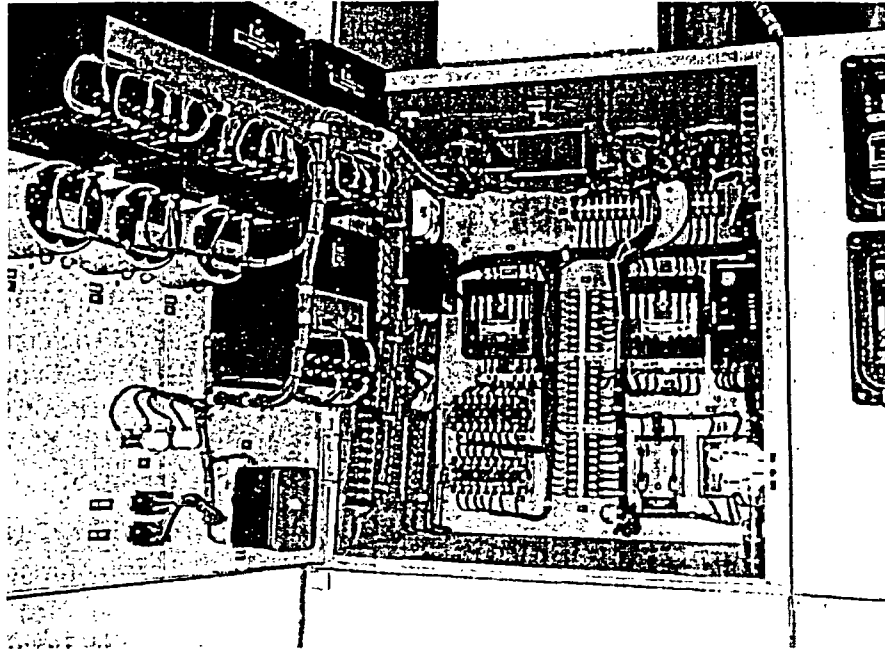
Figure G-3 4.16 kV Switchgear (Front Panel, Open)
