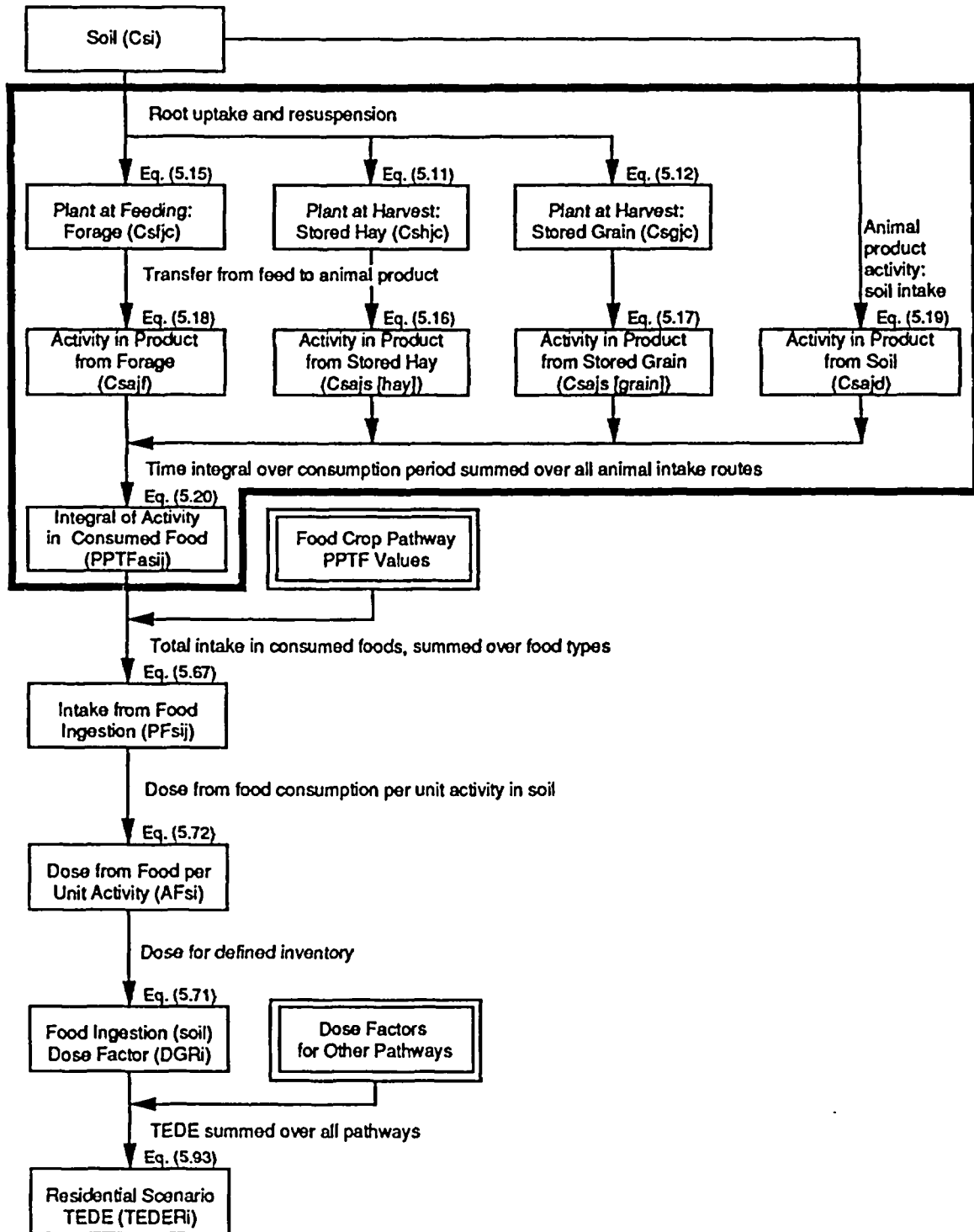
Figure 5.8 Soil-plant-animal-human pathway
