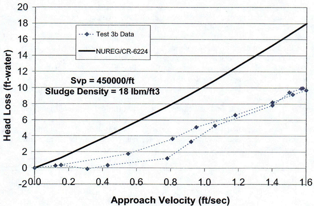
Figure 4.9. Comparison of Test 3b with NUREG/CR-6224 correlation.
