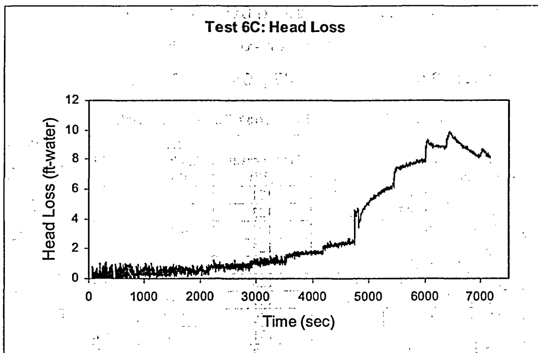
Figure F.3. Test 6C head-loss measurements.
