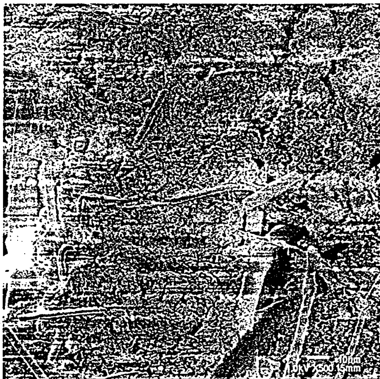
Figure 5.18. Typical Post-Test SEM Photo.
