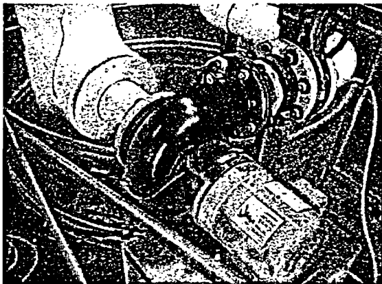
Figure A.11. 5-hp motor at the base of the vertical test section of the hydraulic loop.
