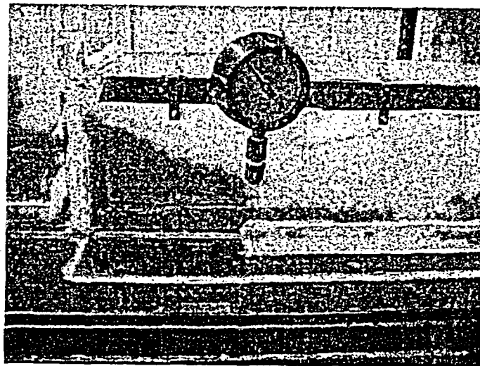
Air pocket formed downstream of screen after 12 pieces collected
