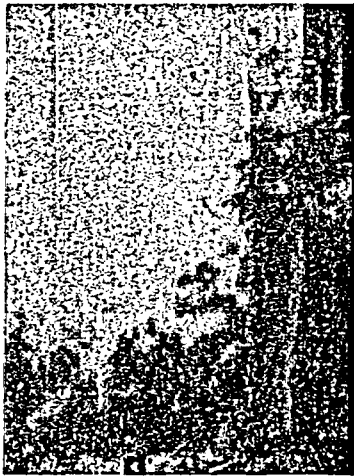
Initial appearance from right side
