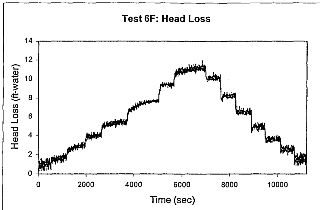
Figure F.7. Test 6F head-loss measurements.
