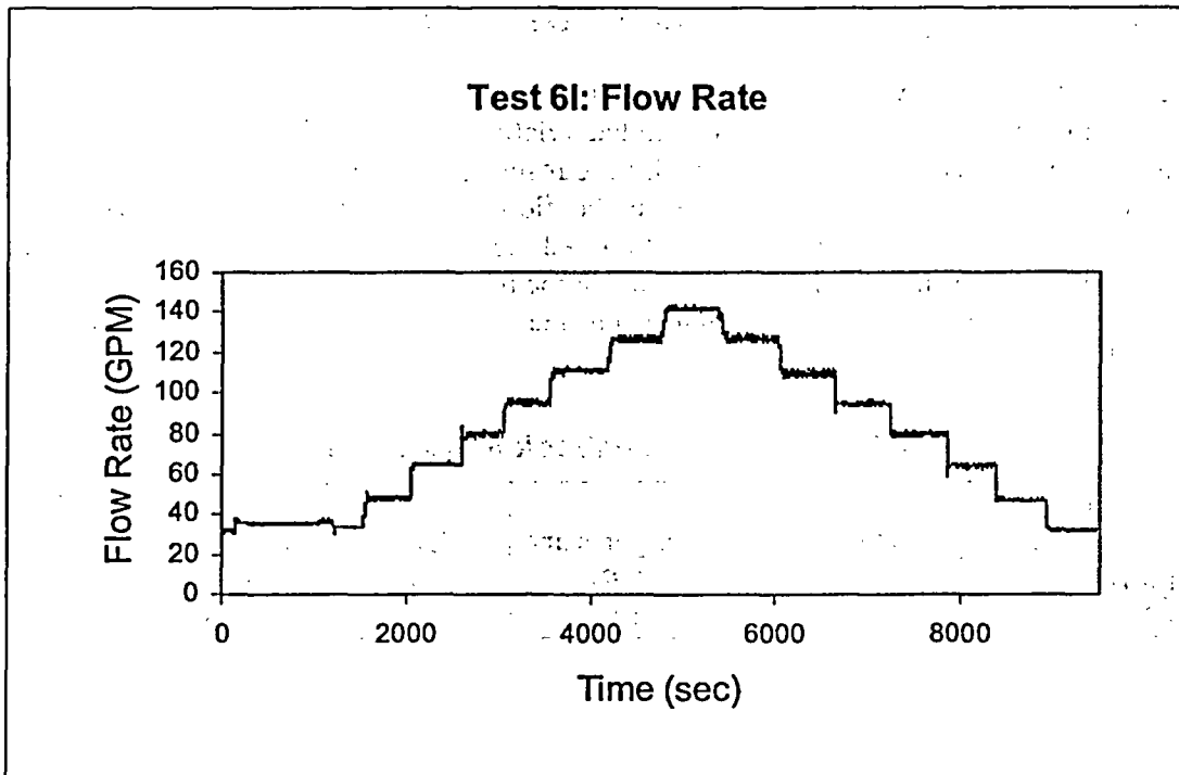
Figure F.13. Test 6I flow measurements.
