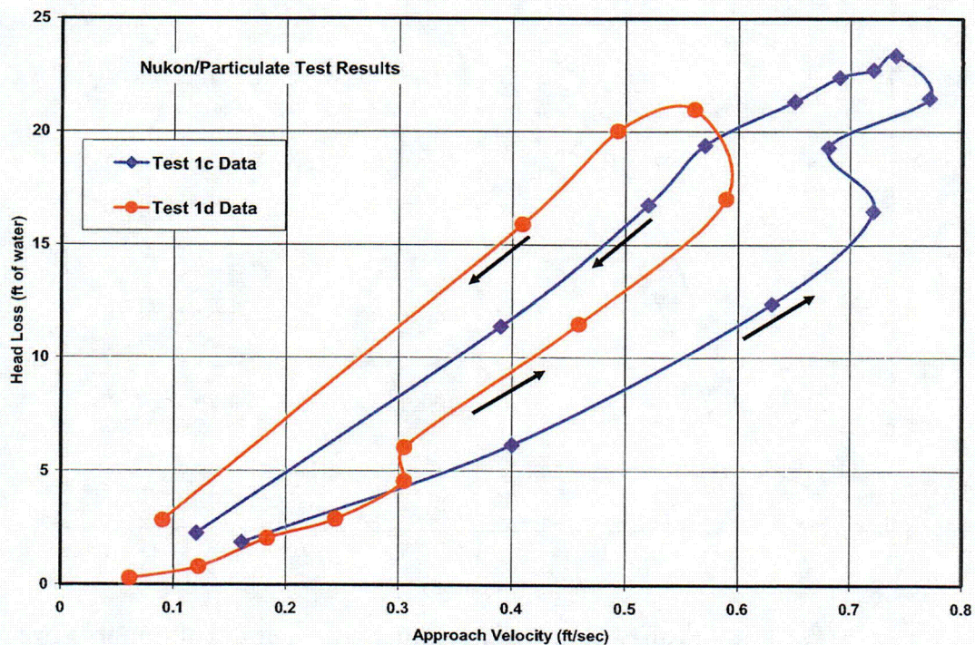
Figure 3.7. Measured head loss for NUKON TM fiber bed with particulate for two fiber bed thicknesses.
