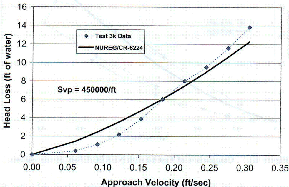
Figure 4.5. Comparison of Test 3k with NUREG/CR-6224 correlation.
