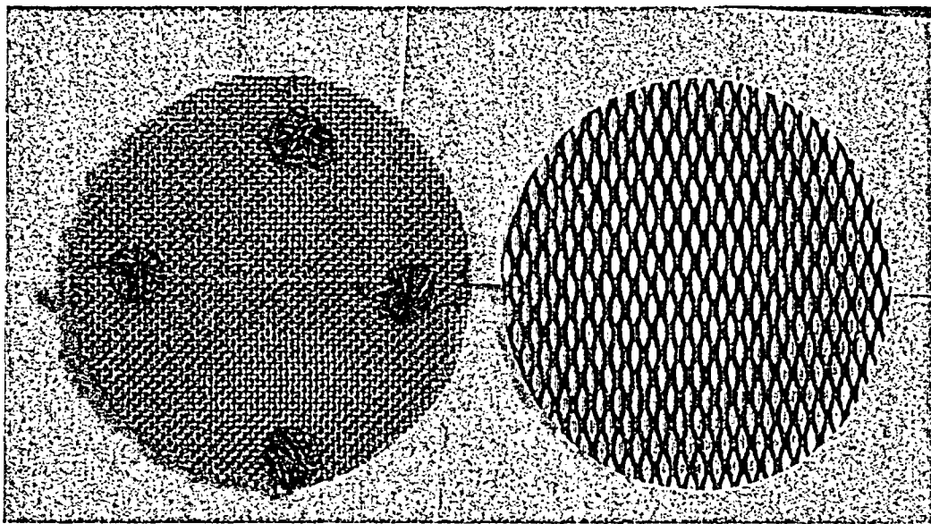
Figure A.9. 1/8-in. mesh 11.5-in.-diameter debris screen (left) and supporting steel reinforcement (right).
