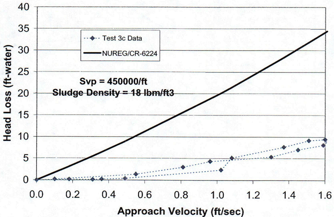
Figure 4.10. Comparison of Test 3c with NUREG/CR-6224 correlation.
