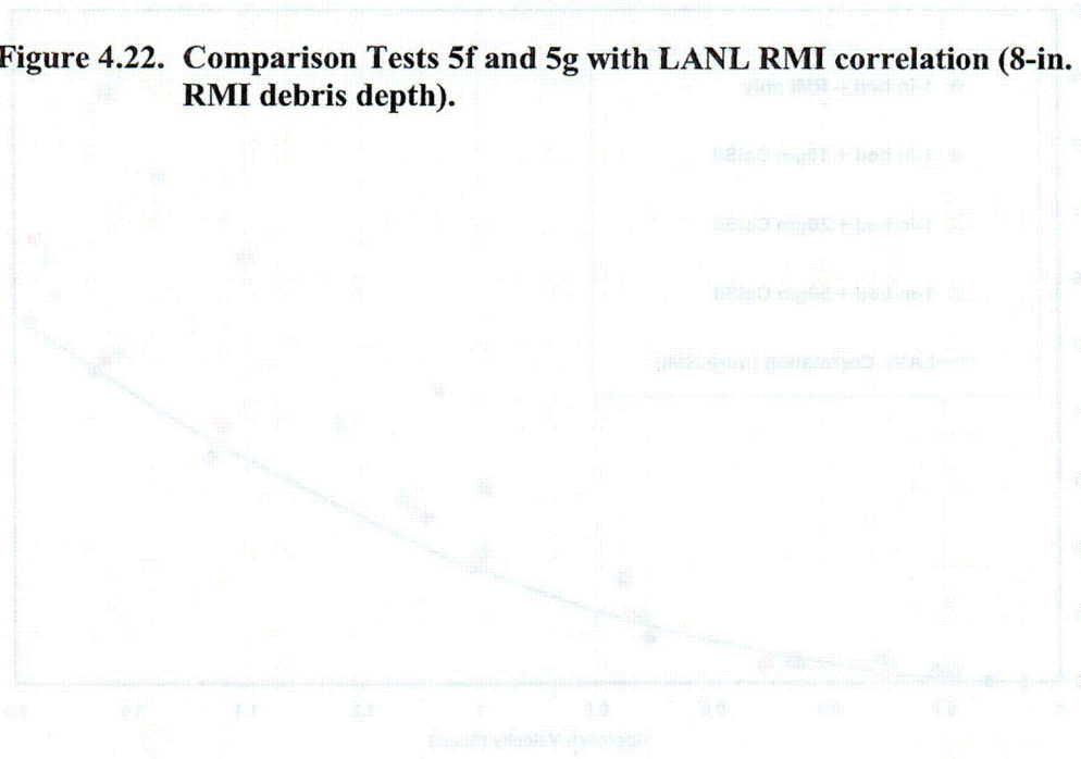
Figure 4.21. Comparison Tests 5c, 5d, and 5e with LANL RMI correlation (1.0-1.0R debris depth).
