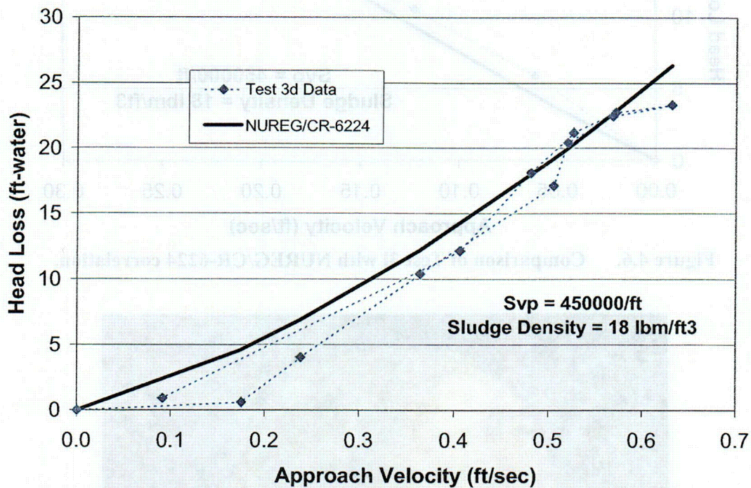
Figure 4.8. Comparison of Test 3d with NUREG/CR-6224 correlation.
