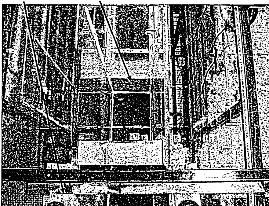
Figure A.3. Flume arrangement from end of converging section through the flow exit tunnel.
