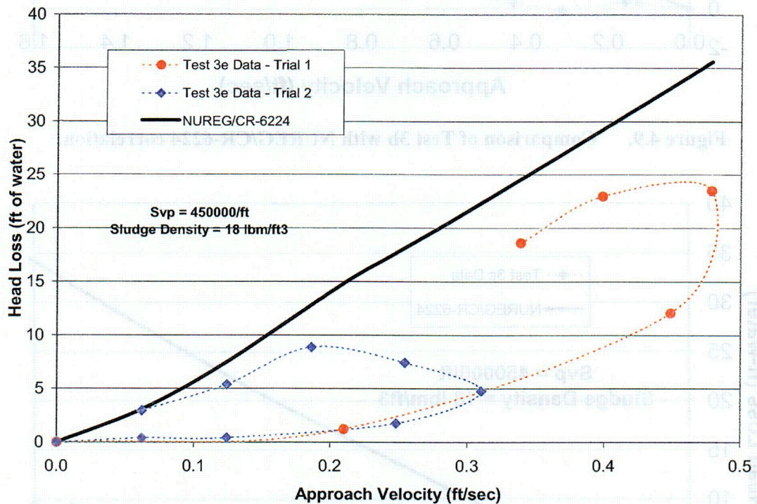
Figure 4.11. Comparison of Test 3e with NUREG/CR-6224 correlation.
