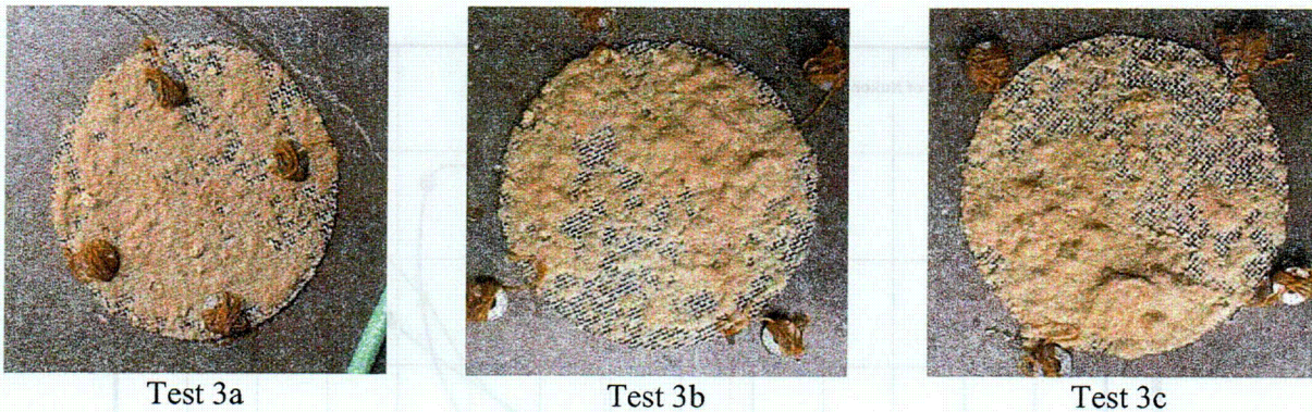
Figure 3.13. Post-test debris distribution on horizontal screens in thin-bed mixed debris Tests 3a-c.
