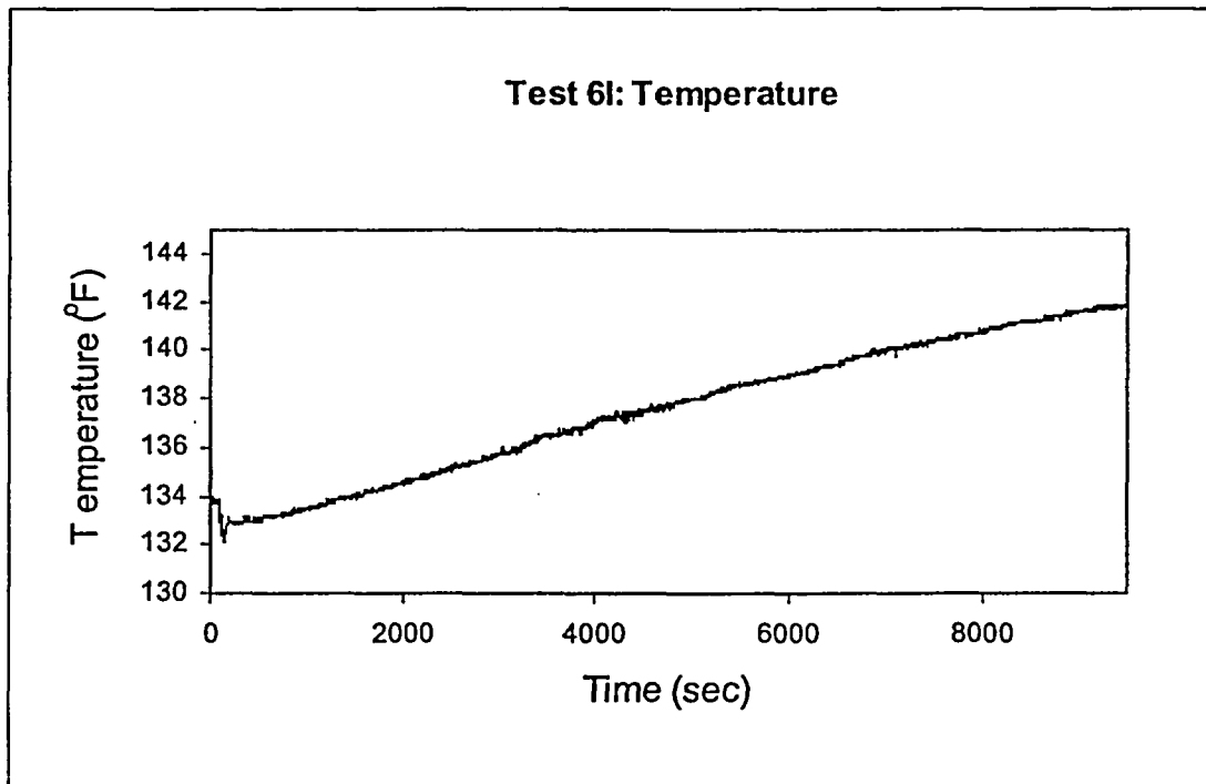
Figure F.14. Test 6I temperature measurements.
