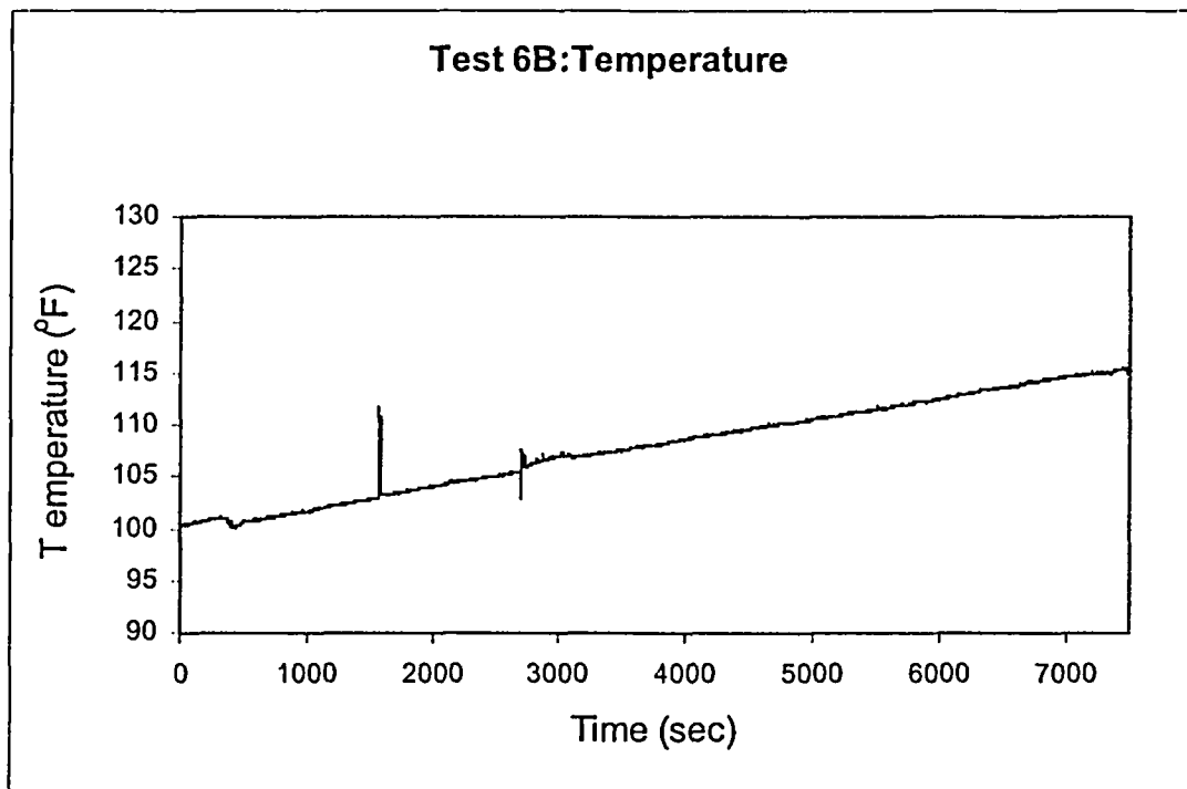
Figure F.2. Test 6B temperature measurements.
