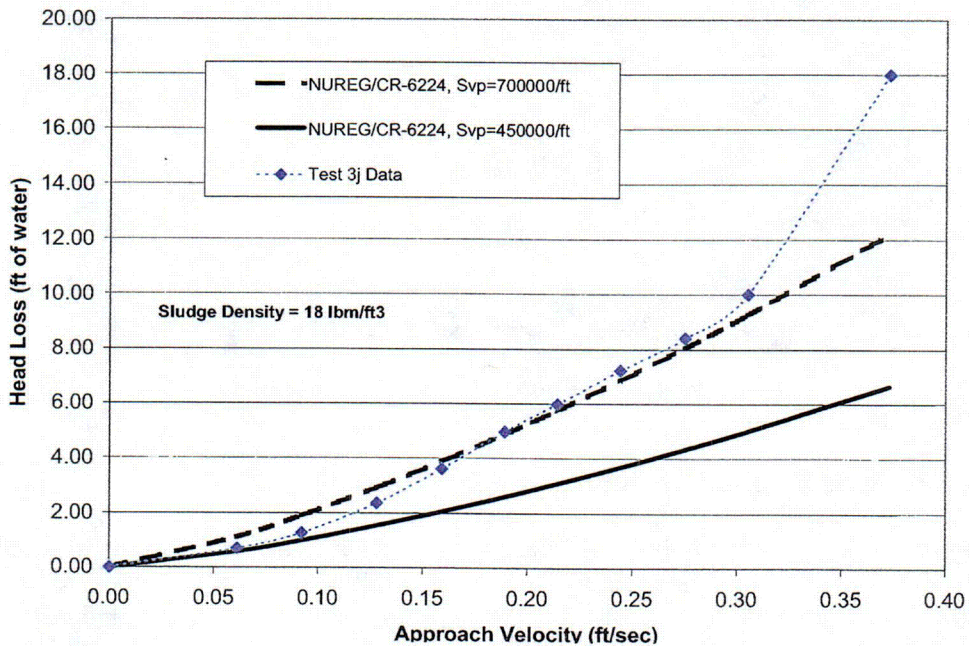
Figure 4.17. Comparison of Test 3j with NUREG/CR-6224 correlation.
