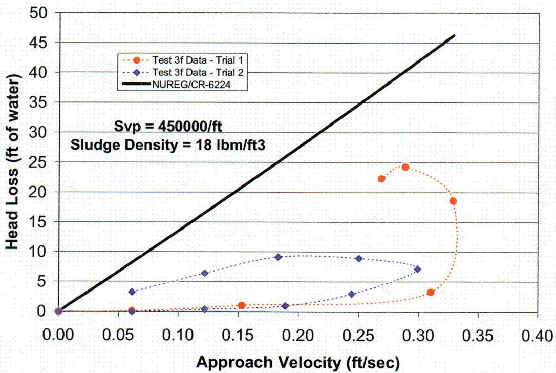
Figure 4.12. Comparison of Test 3f with NUREG/CR-6224 correlation.
