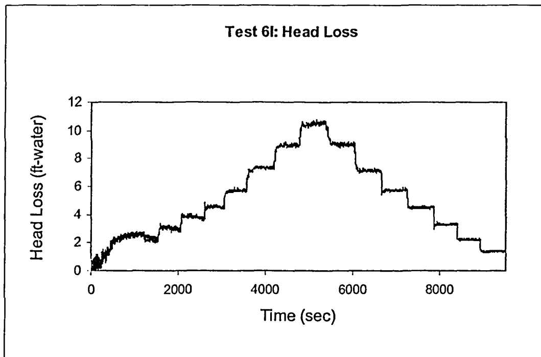
Figure F.12. Test 6I head-loss measurements.
