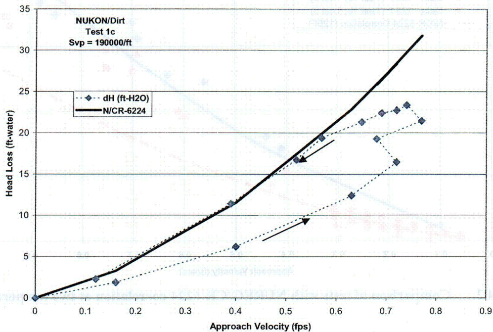
Figure 4.3. Comparison of Test 1c with NUREG/CR-6224 correlation.
