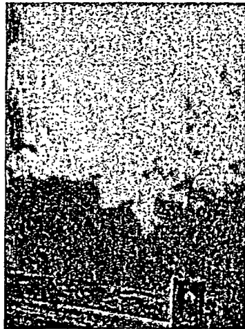
Initial appearance from left side
