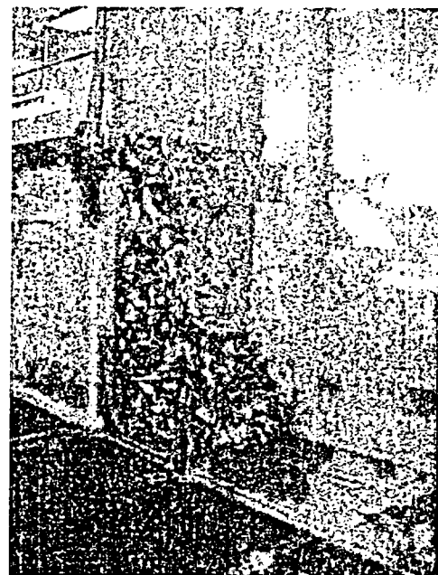
Test 4 (final accumulation profile)
