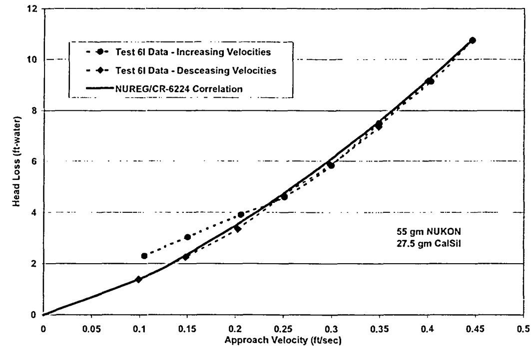
Figure 5.8. Comparison of NUREG/CR-6224 correlation with Test 6I head-loss data.
