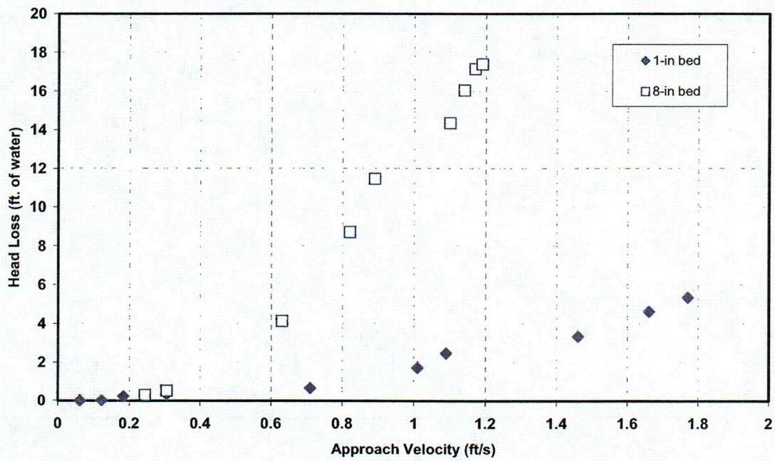
Figure 3.21. Stainless-steel RMI foil head-loss data.
