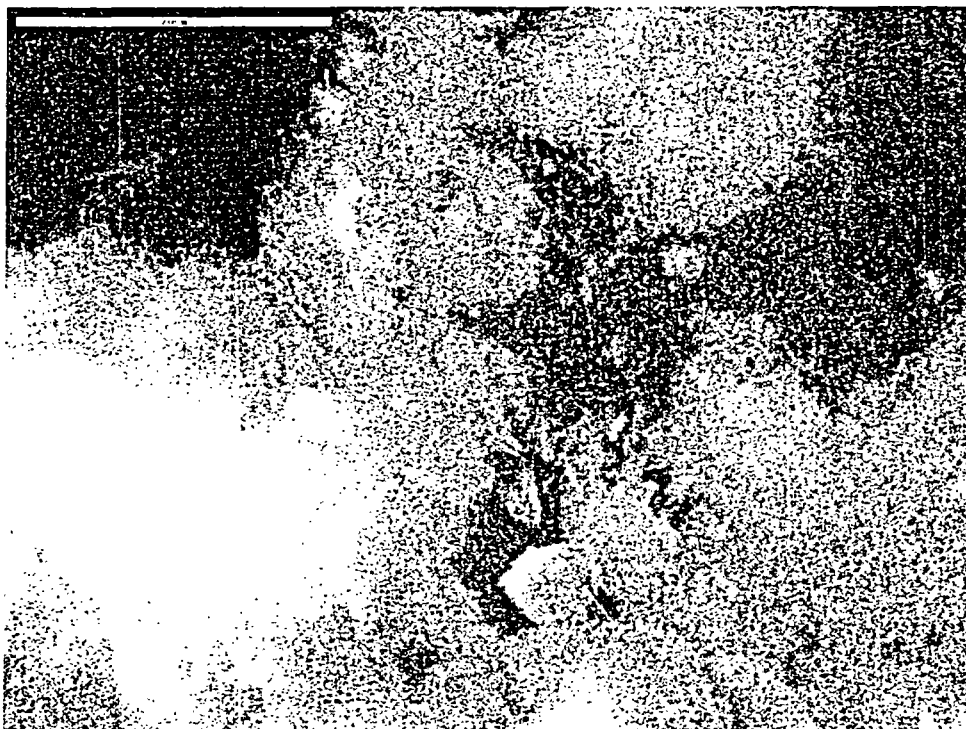
Figure 5.3. SEM photo at a magnification of 20 microns.
