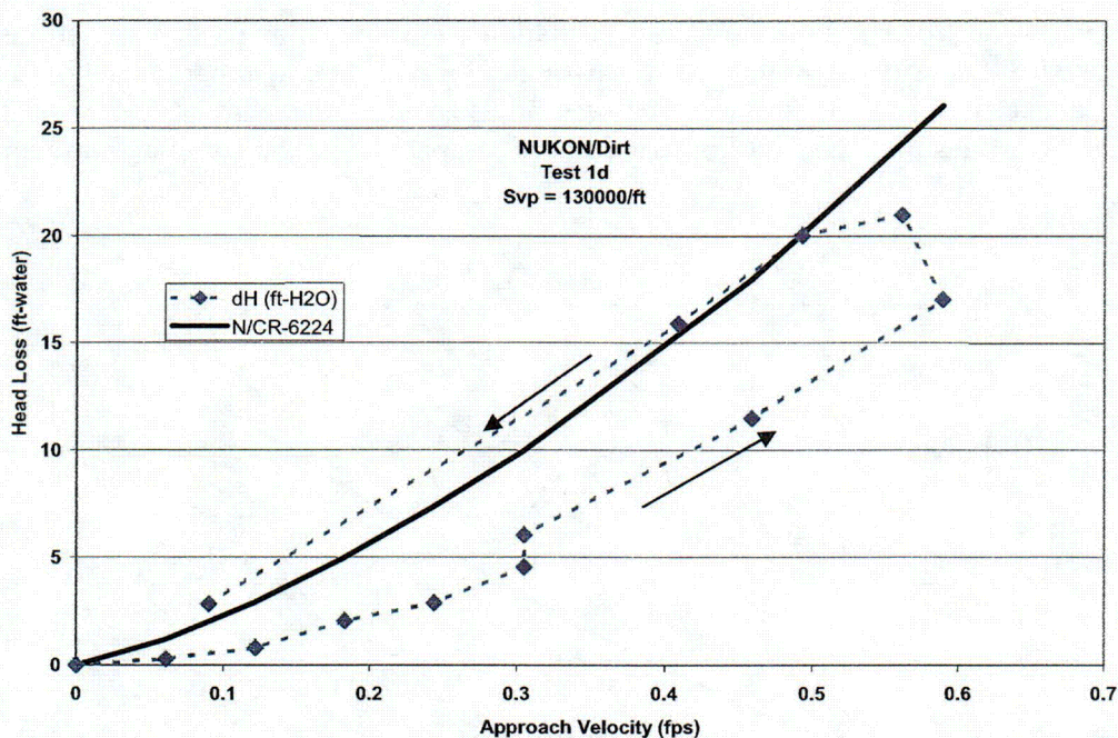
Figure 4.4. Comparison of Test 1d with NUREG/CR-6224 correlation.
