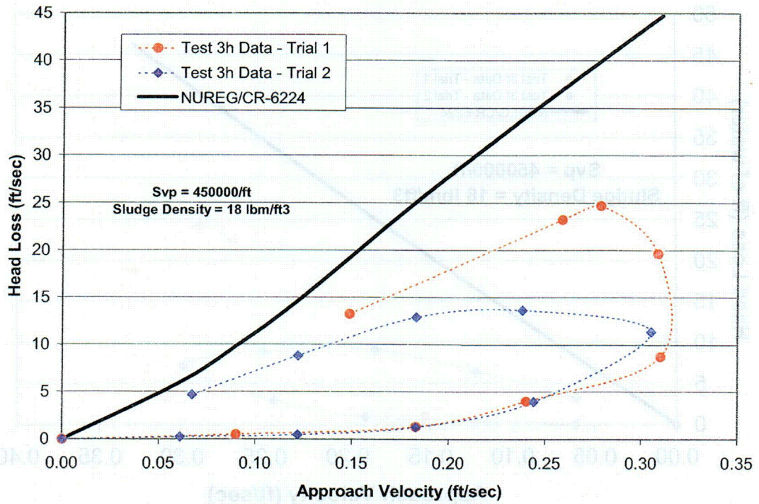
Figure 4.14. Comparison of Test 3h with NUREG/CR-6224 correlation.
