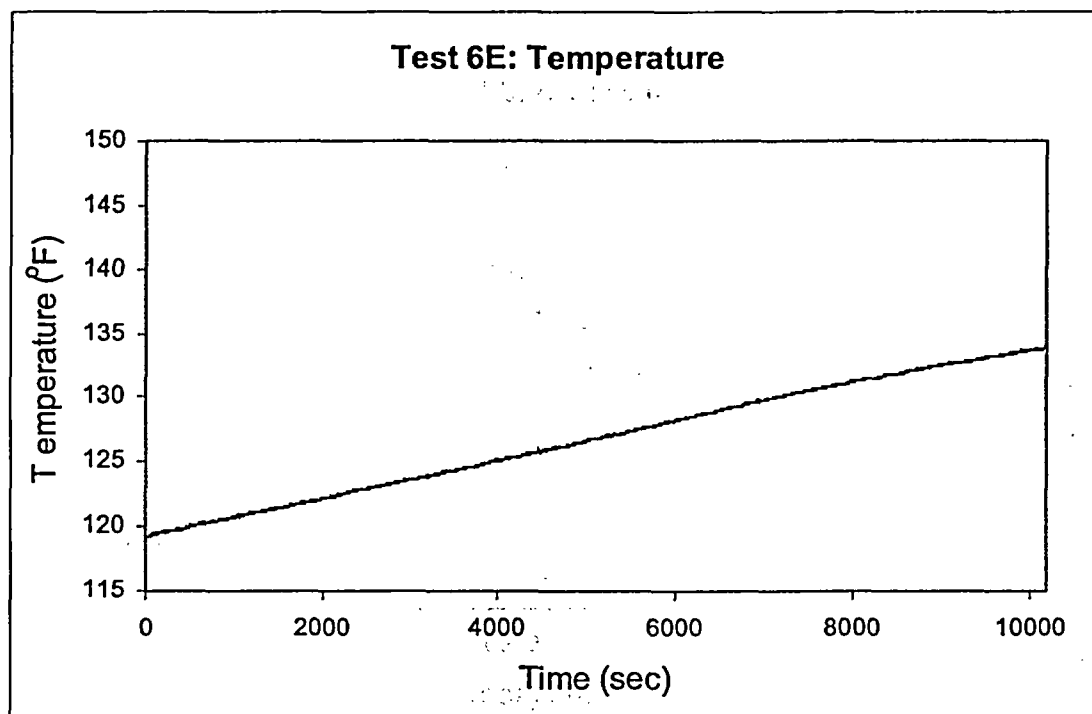
Figure F.6. Test 6E temperature measurements.
