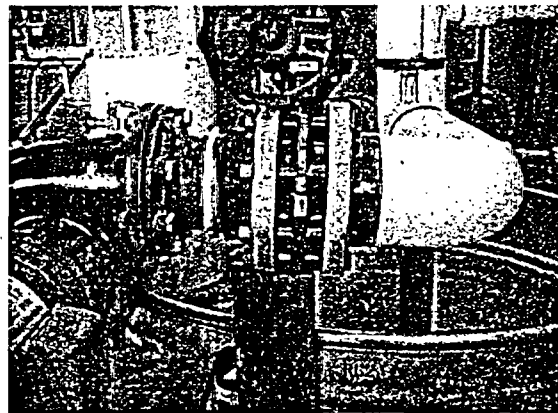
Figure A.12. Flow control valve adjacent to the loop pump.
