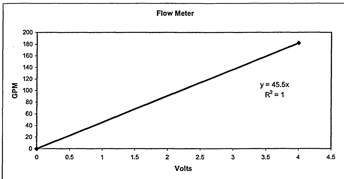
Figure E.2. Voltage-transmitter linear range correlation.
