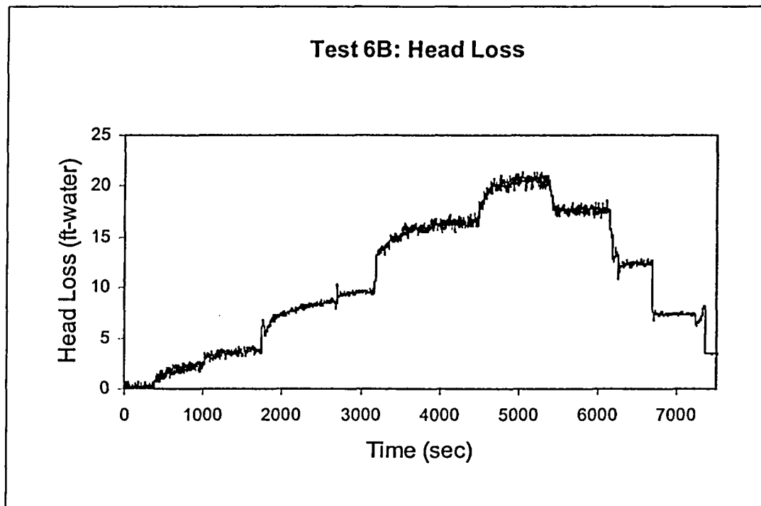
Figure F.1. Test 6B head-loss measurements.
