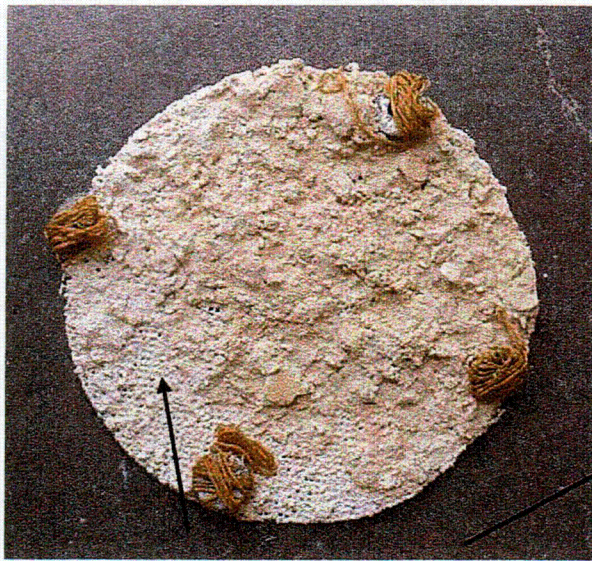
Test 2b. Screen visible through debris
