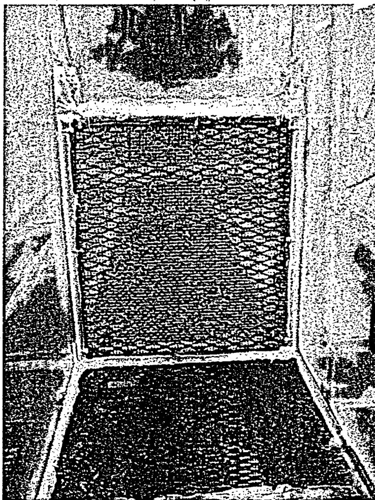
Figure A.2. Debris screen at entrance to flume exit tunnel (large, diamond-shaped mat behind screen is for structural reinforcement only).
