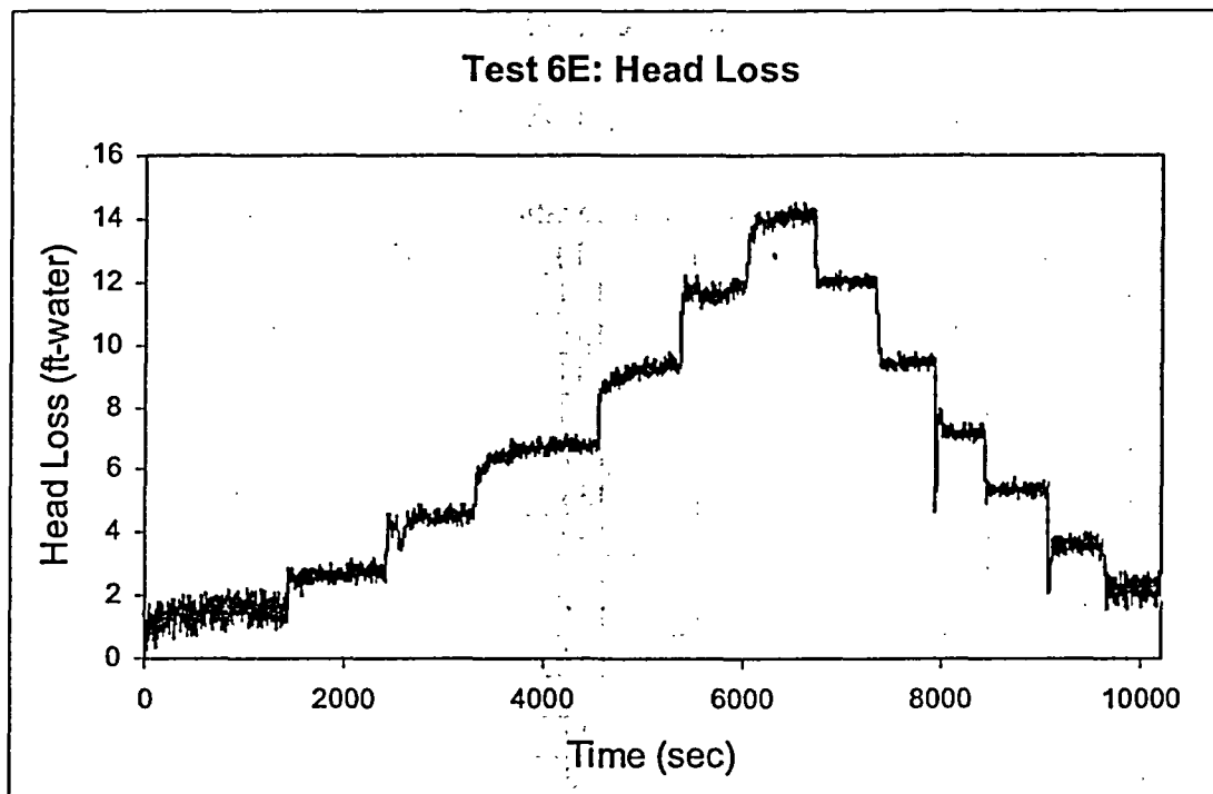
Figure F.5. Test 6E head-loss measurements.
