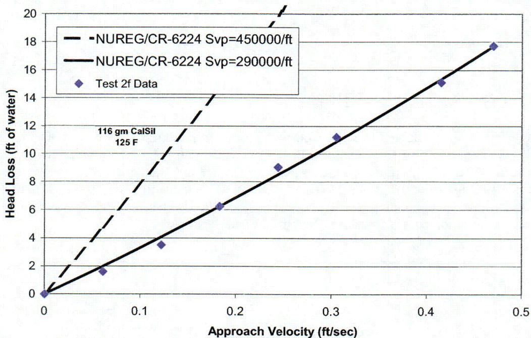
Figure 4.19. Comparison of Test 2f with NUREG/CR-6224 correlation.
