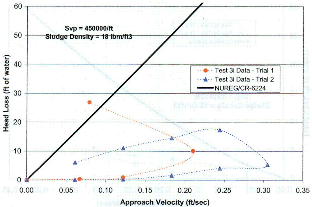
Figure 4.15. Comparison of Test 3i with NUREG/CR-6224 correlation.
