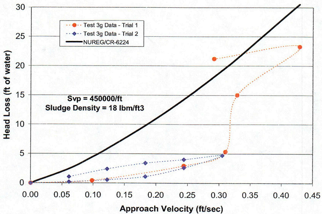
Figure 4.13. Comparison of Test 3g with NUREG/CR-6224 correlation.
