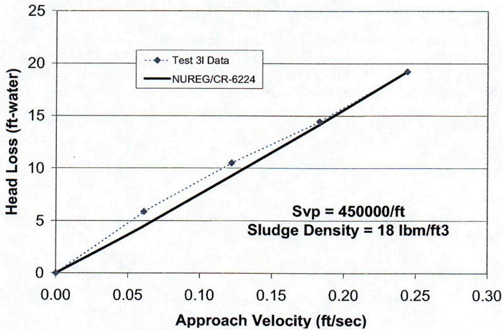
Figure 4.6. Comparison of Test 31 with NUREG/CR-6224 correlation.
