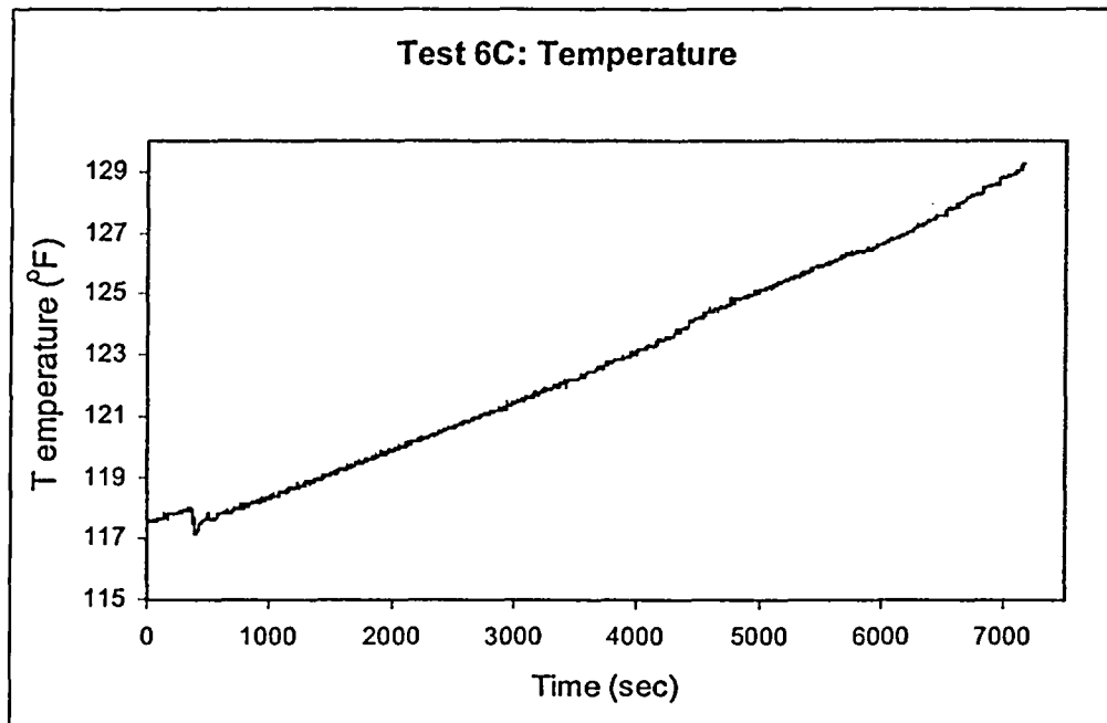
Figure F.4. Test 6C temperature measurements.
