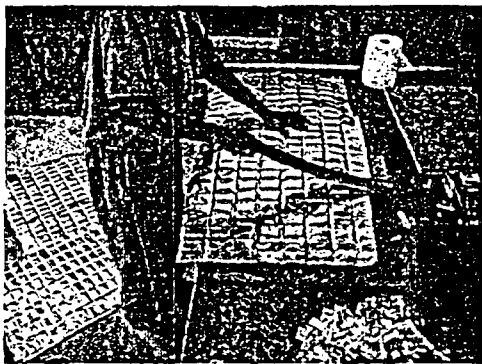
Figure C.3. Cutting RMI foil.
