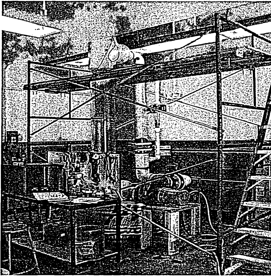
Figure A.8. UNM closed-loop head-loss test facility.
