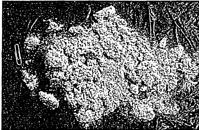
Figure C.2. Hand-crushed CalSil debris.
