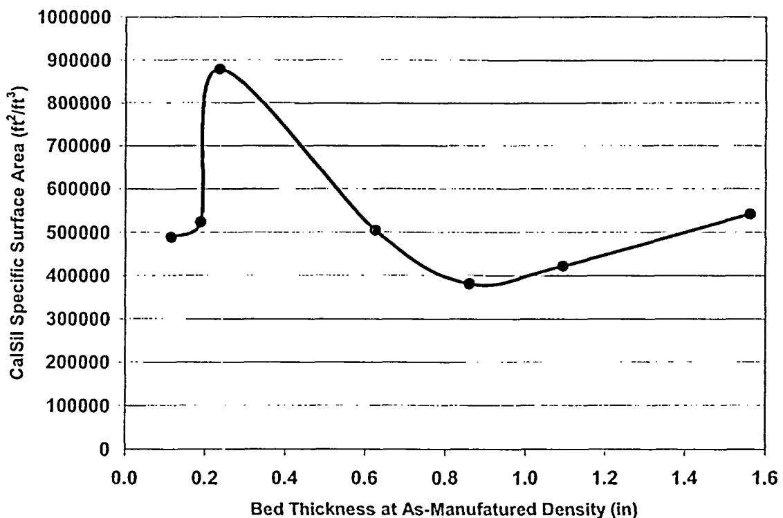
Figure 5.17. Comparison of deduced specific surface areas.
