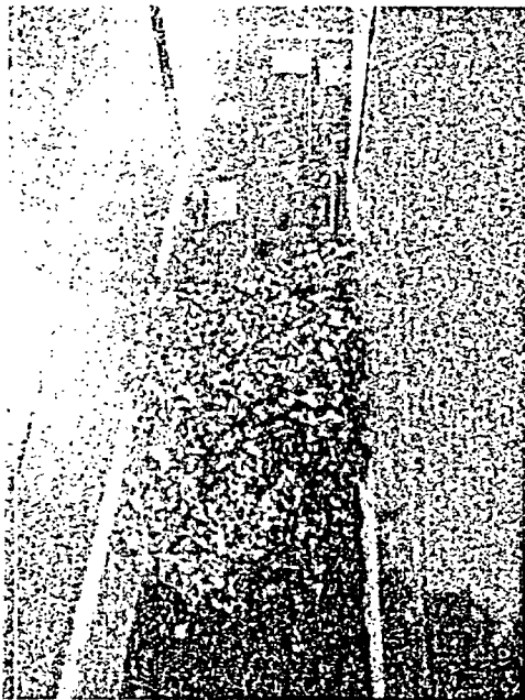
Test 4 (top view during transport)
