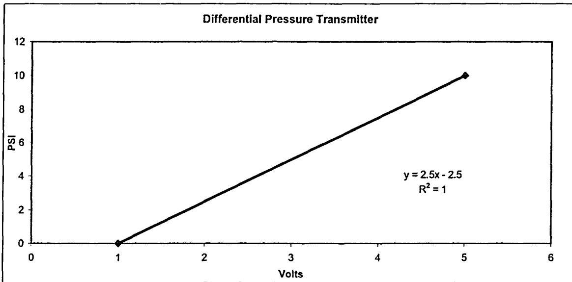
Figure E.1. Voltage-transmitter linear range correlation.
