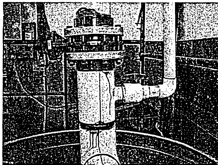
Figure A.10. Intersection of the bases of the 6-in. inner recirculation loop and the 2-in. outer recirculation loop.
