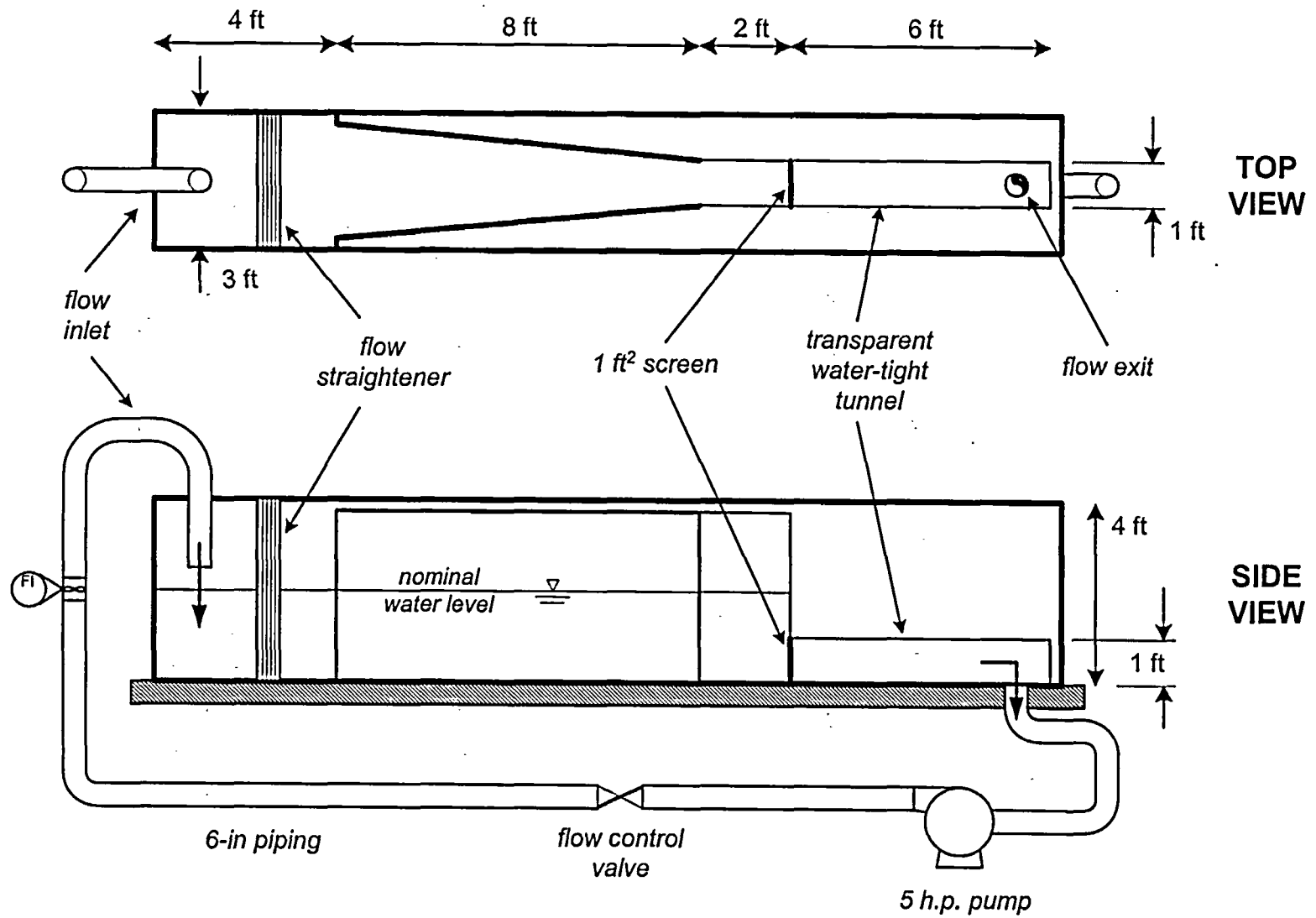
Figure A.1. Flume configuration.
