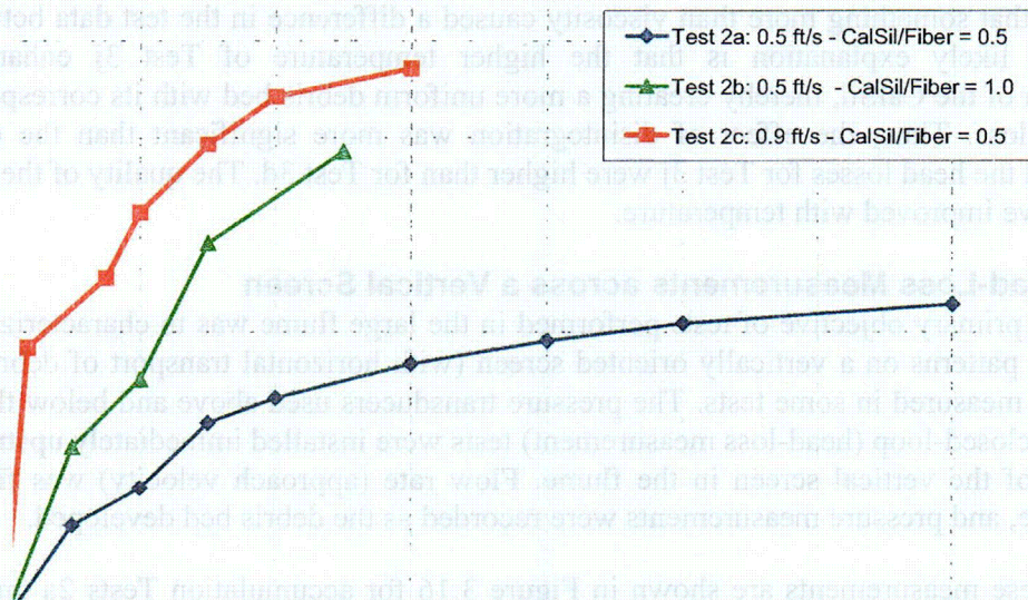
Figure 3.16. Time-dependent head-loss measurements during debris-accumulation Tests 2a-2c.
