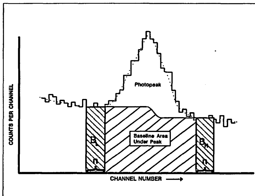
FIGURE 16.5 — Photopeak baseline continuum-step function
