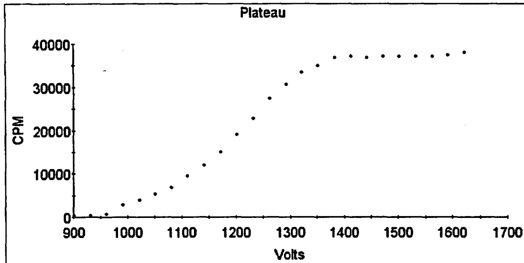
FIGURE 15.3 — Beta plateau generated by a ^{90}\text{Sr}/\text{Y} source on a GP counter using P-10 gas
