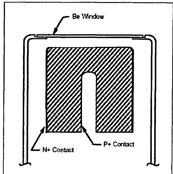
FIGURE 15.10 — Extended range coaxial germanium detector
