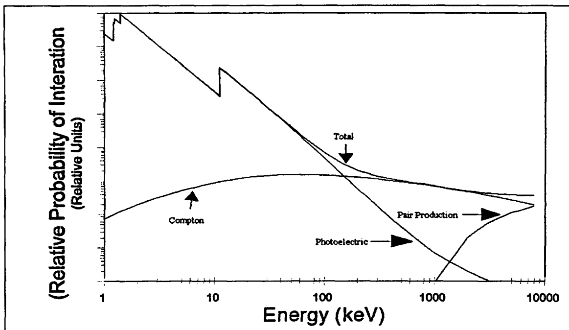
FIGURE 15.6 — Gamma-ray interactions with high-purity germanium
