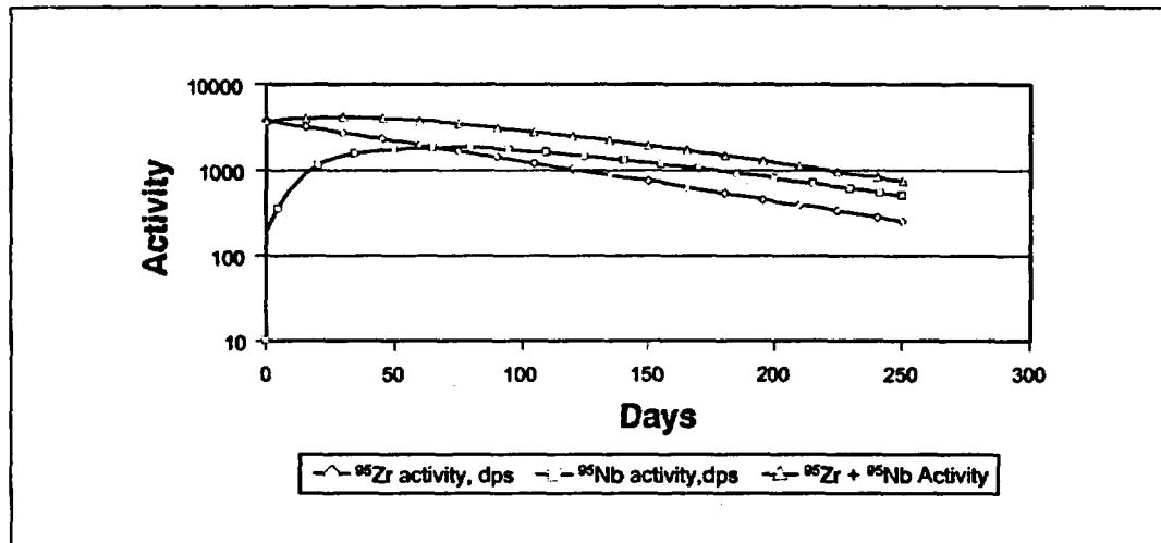
FIGURE 14A.3 — Transient equilibrium of 95 Zr/ 95 Nb
