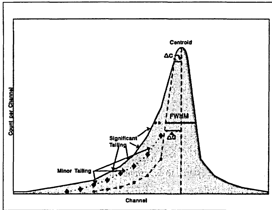
FIGURE 16.3 — Low-energy tailing
