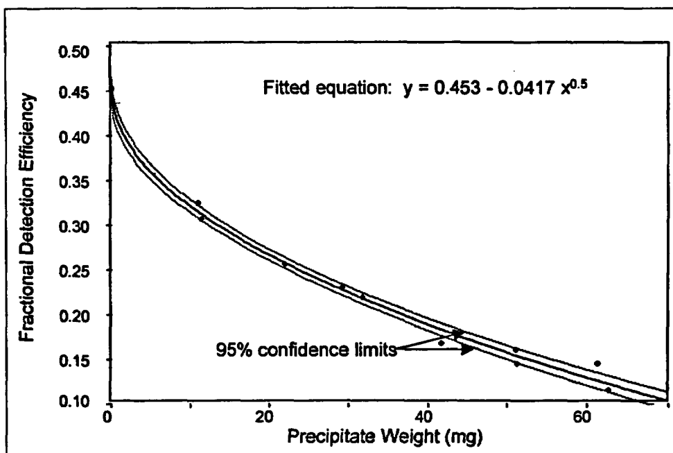
FIGURE 15.2 — Gas proportional counter self-absorption curve for ^{230}\text{Th}
