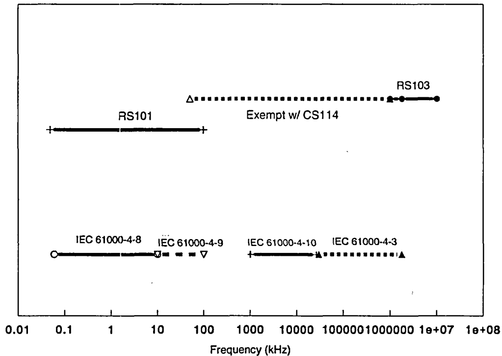
Fig. 7.1. Radiated susceptibility frequency coverage.
