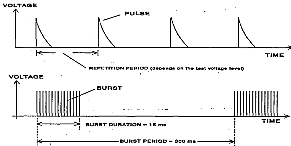
Fig. 6.8. IEC 6100-4-4 electrically fast transients/bursts.
