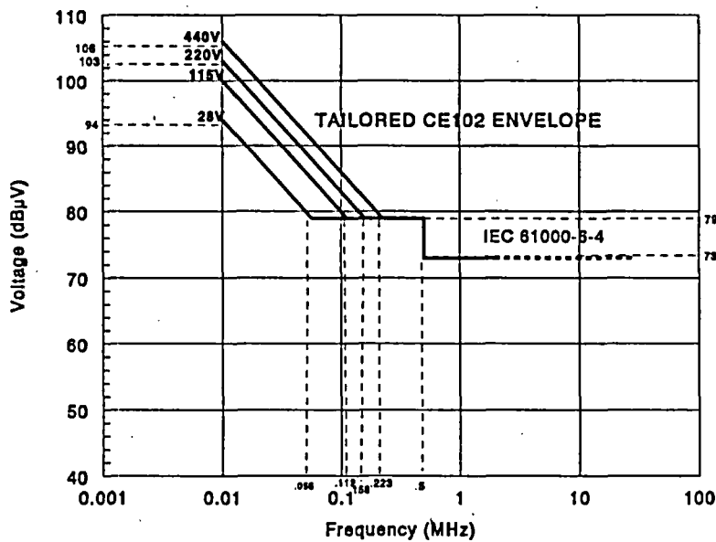
Fig. 5.5. CE102 operating envelope.
