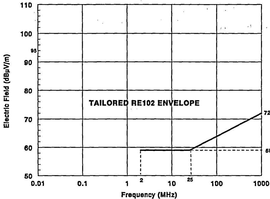
Fig. 5.6. RE102 operating envelope.
