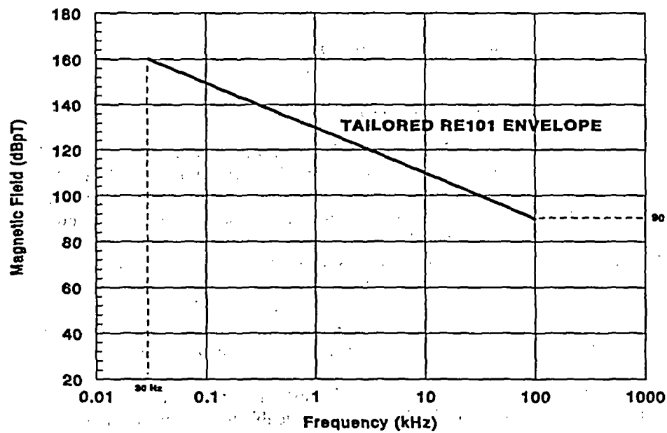
Fig. 5.3. RE101 operating envelope.
