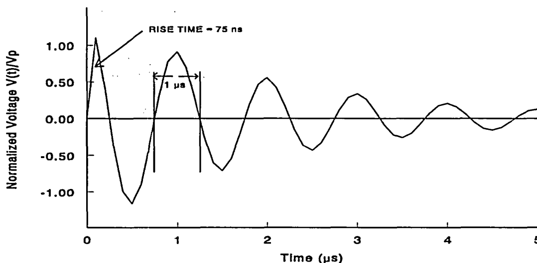
Fig. 6.13. Waveform of the damped oscillatory wave.
