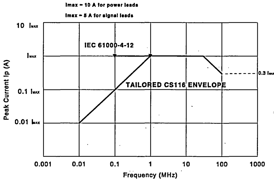
Fig. 6.14. Damped sinusoid conducted susceptibility operating envelopes.
