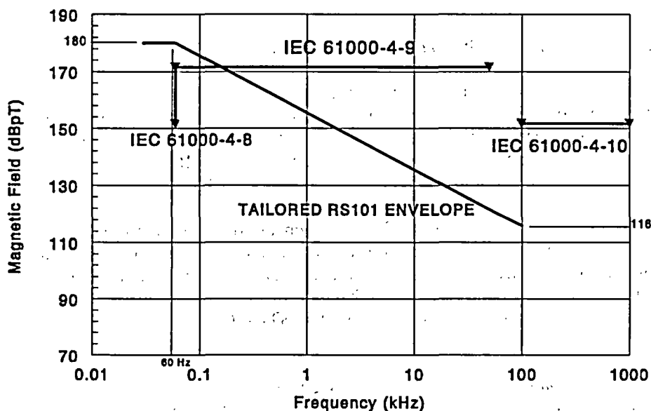
Fig. 7.2. Low-frequency radiated susceptibility operating envelopes.
