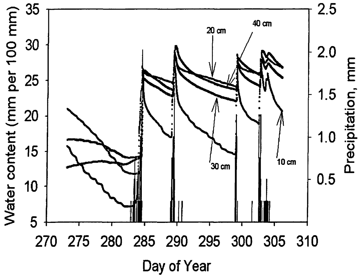
Figure 5. Dynamics of water contents measured over a 30-day period during October, 2002 in location LIPI. The data from the four depths are noted in the figure.
