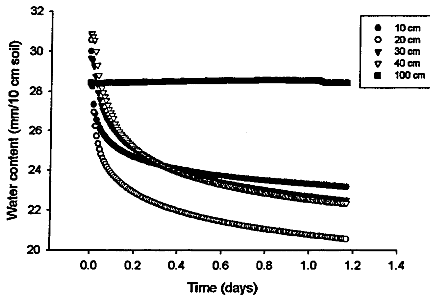
Figure 10. Redistribution as a function of time for the sandy soil at 5 depths. The data are from spatial averages of 8 locations and temporal averages over 15 minute periods.
