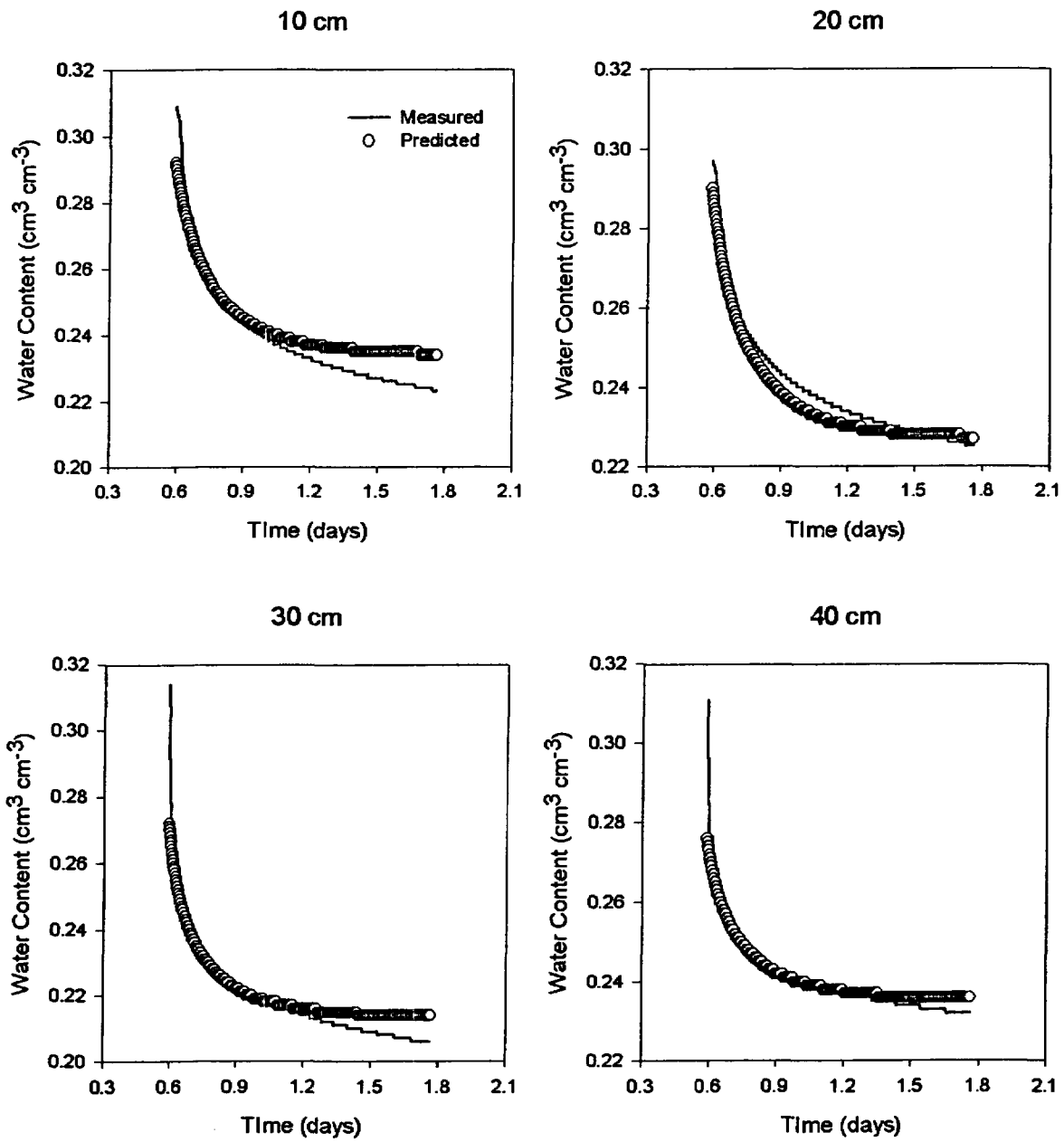
Figure 25. Measured water contents and water contents predicted by HYDRUS-2D for the optimal inverse solution.
