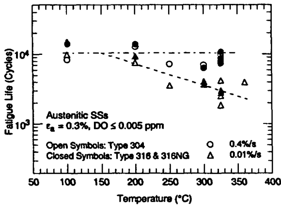
Figure 14. Change in fatigue lives of austenitic stainless steels in low-DO water with temperature (Refs. 17,19-22,26,27).
