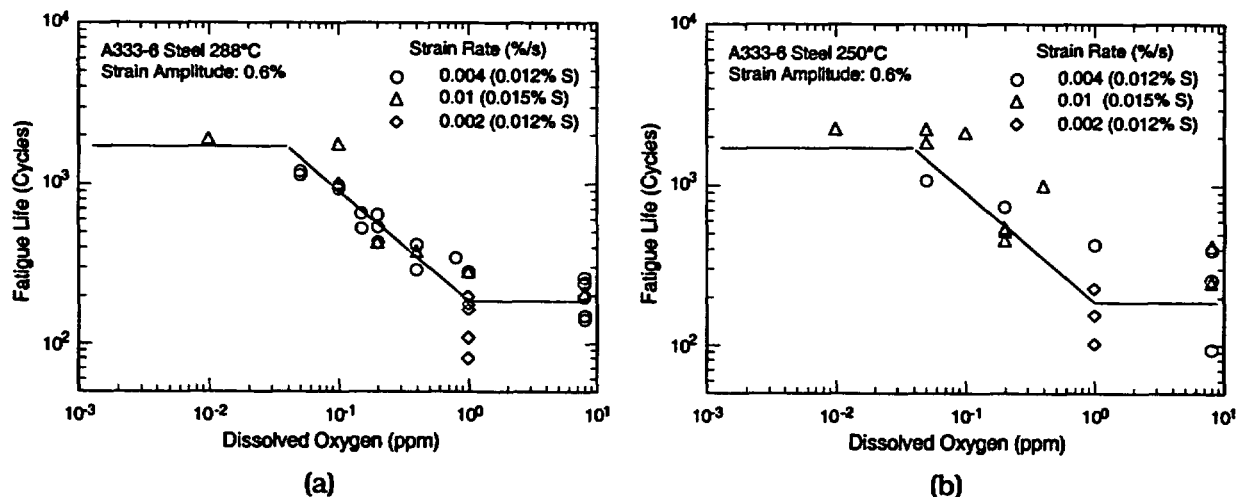
Figure 7. Dependence on dissolved oxygen of fatigue life of carbon steels at (a) 288 and (b) 250^{\circ}\text{C} (Refs. 7,9).
