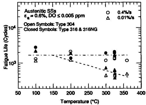
Figure 14. Change in fatigue lives of austenitic stainless steels in low-DO water with temperature (Refs. 17,19-22,26,27).
