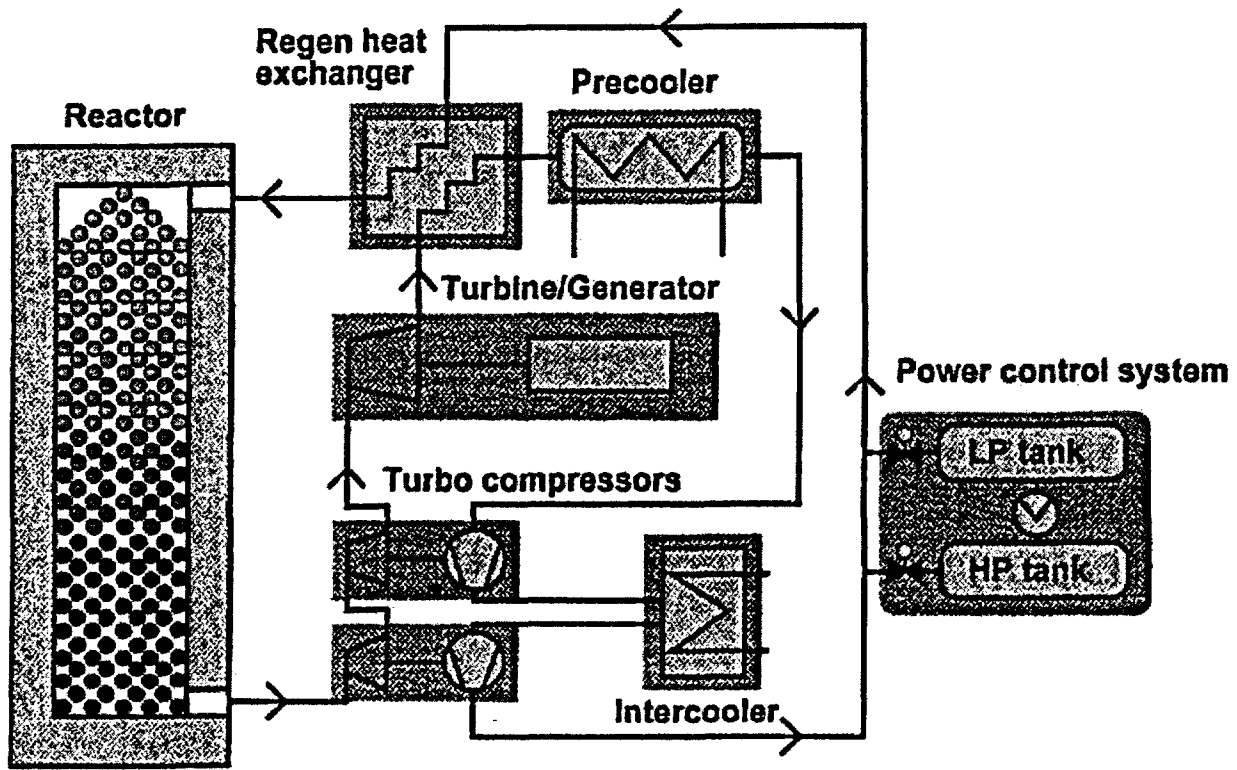
Figure 1.2 Schematic of pebble bed modular helium reactor (PBMHR)
