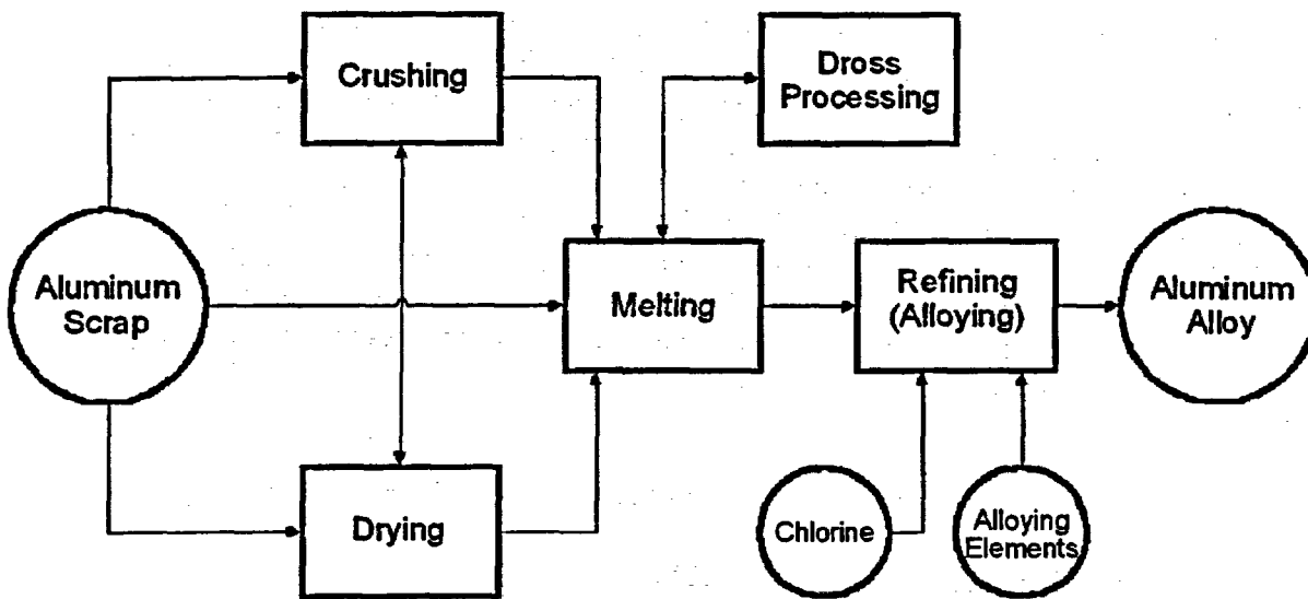
Figure 5.2 Processing and melting of aluminum scrap at typical secondary smelter
