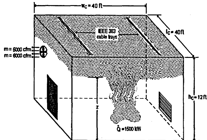
Problem 6: Compartment Fire with Forced Ventilation
