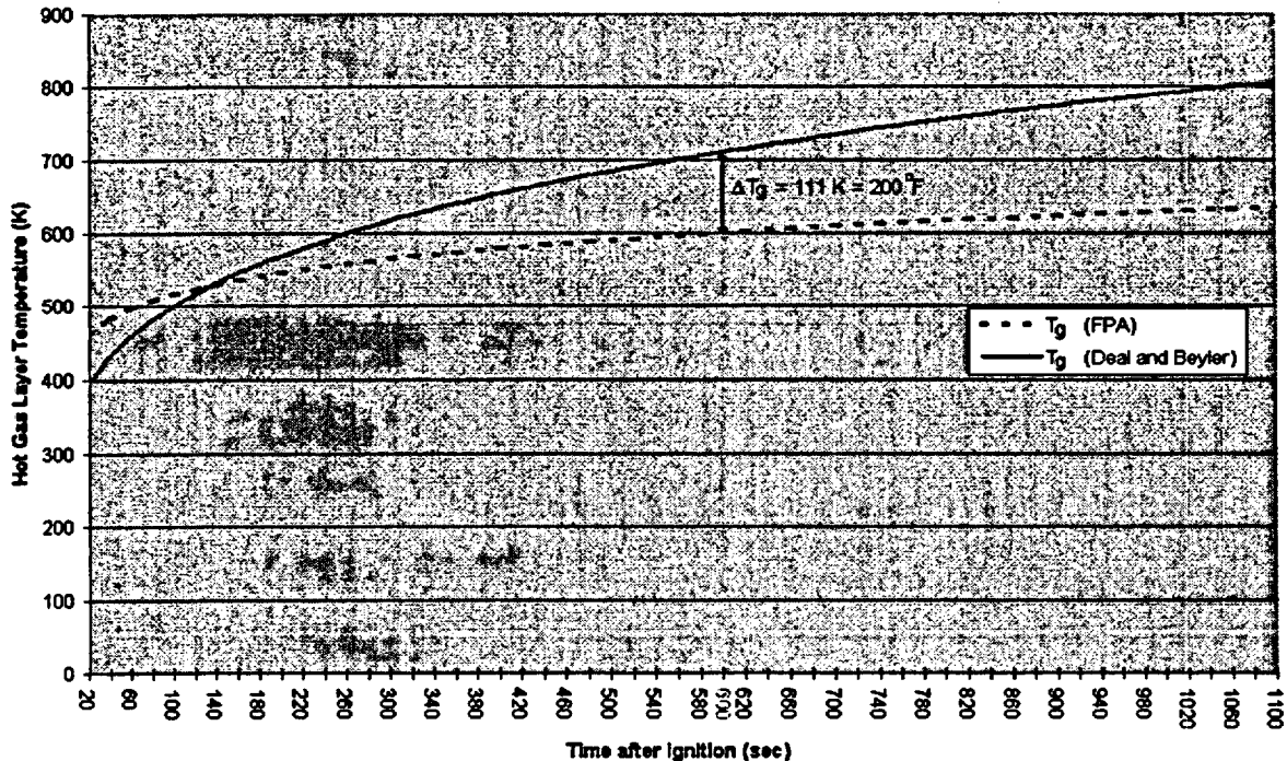
Problem 3: Hot Gas Layer Temperature for Forced Ventilation Scenario Method of FPA and Deal-Beyler
