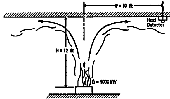
Problem 12: Fire Scenario with Heat Detectors
