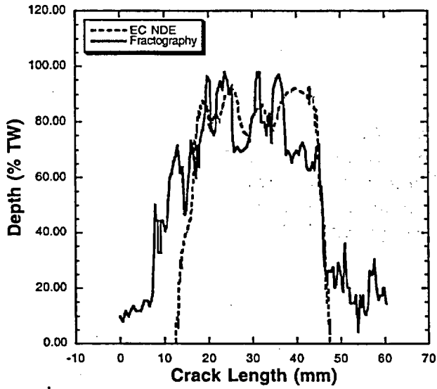
Figure 64. Comparison of NDE and fractography profiles for specimen AGL 824 with axial ODSCC
