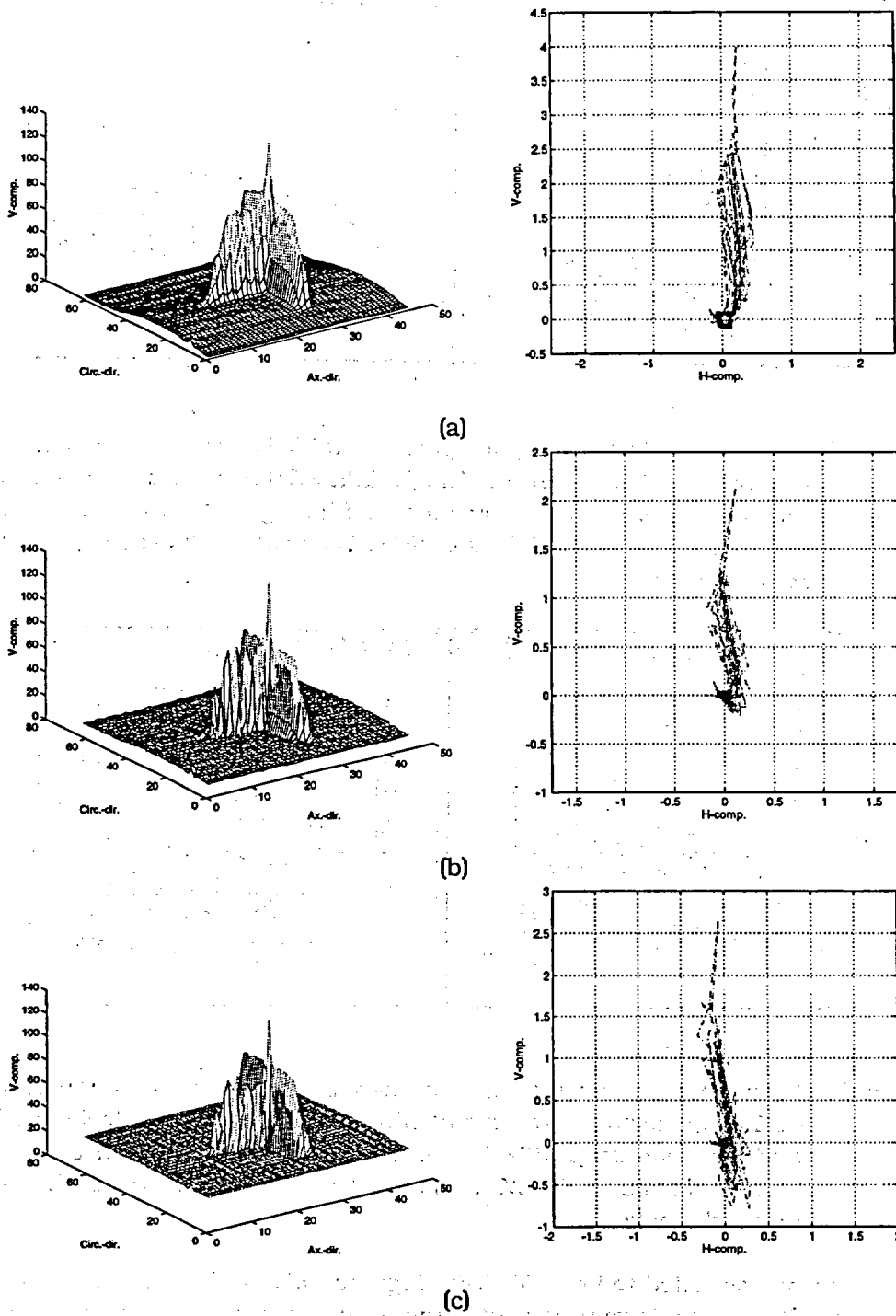
Figure 15. (a) Original and (b)-(c) restored signals with 2-D Lorentzian kernels for Type-9 laser-cut specimen #5469-4-3 with nominal OD flaw depth of 80% TW. NDE maximum depth estimates were 48% by bobbin coil (phase-angle) and 69% by multiparameter analysis of RPC (2.92-mm [0.115-in.] pancake) data.
