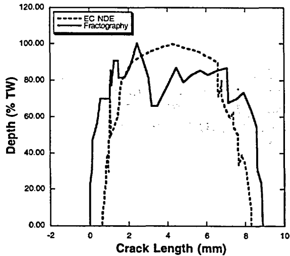
Figure 59. Comparison of NDE and fractography profiles for specimen AGL 535 with axial ODSCC.
