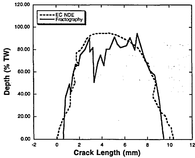
Figure 58. Comparison of NDE and fractography profiles for specimen AGL 533 with axial ODSCC.
