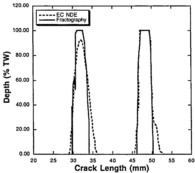
Figure 57. Comparison of NDE and fractography profiles for specimen AGL 394 with circumferential ODSCC.
