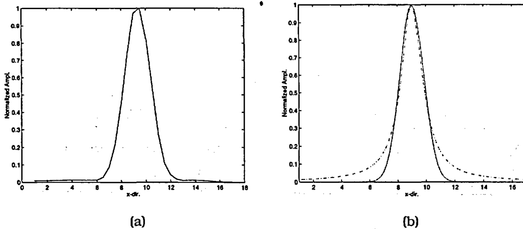
Figure 5. (a) Typical amplitude response of RPC (2.92-mm [0.115-in.] pancake) to 100% TW, 6.35-mm (0.25-in.)-long axial EDM notch at 300 kHz and (b) normalized Gaussian [solid line] and Lorentzian (dashed line) impulse responses having approximately same parameters.
