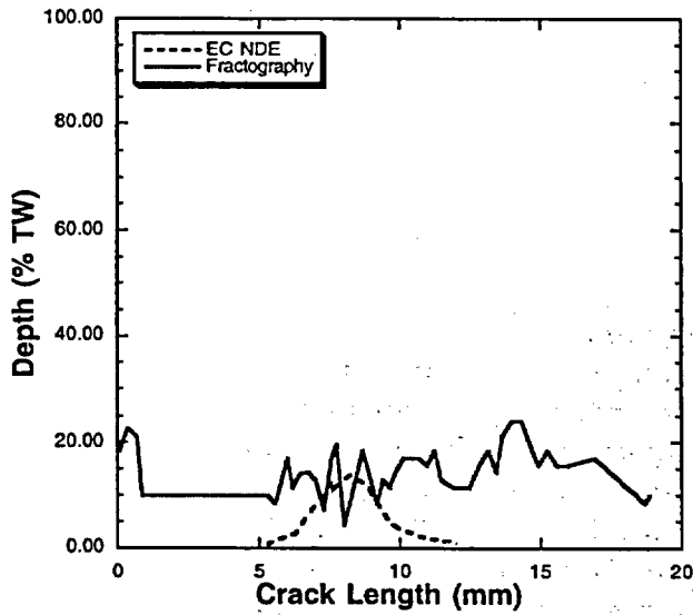
Figure 76. Comparison of NDE and fractography profiles for specimen AGL 816 with axial IDSCC (2)
