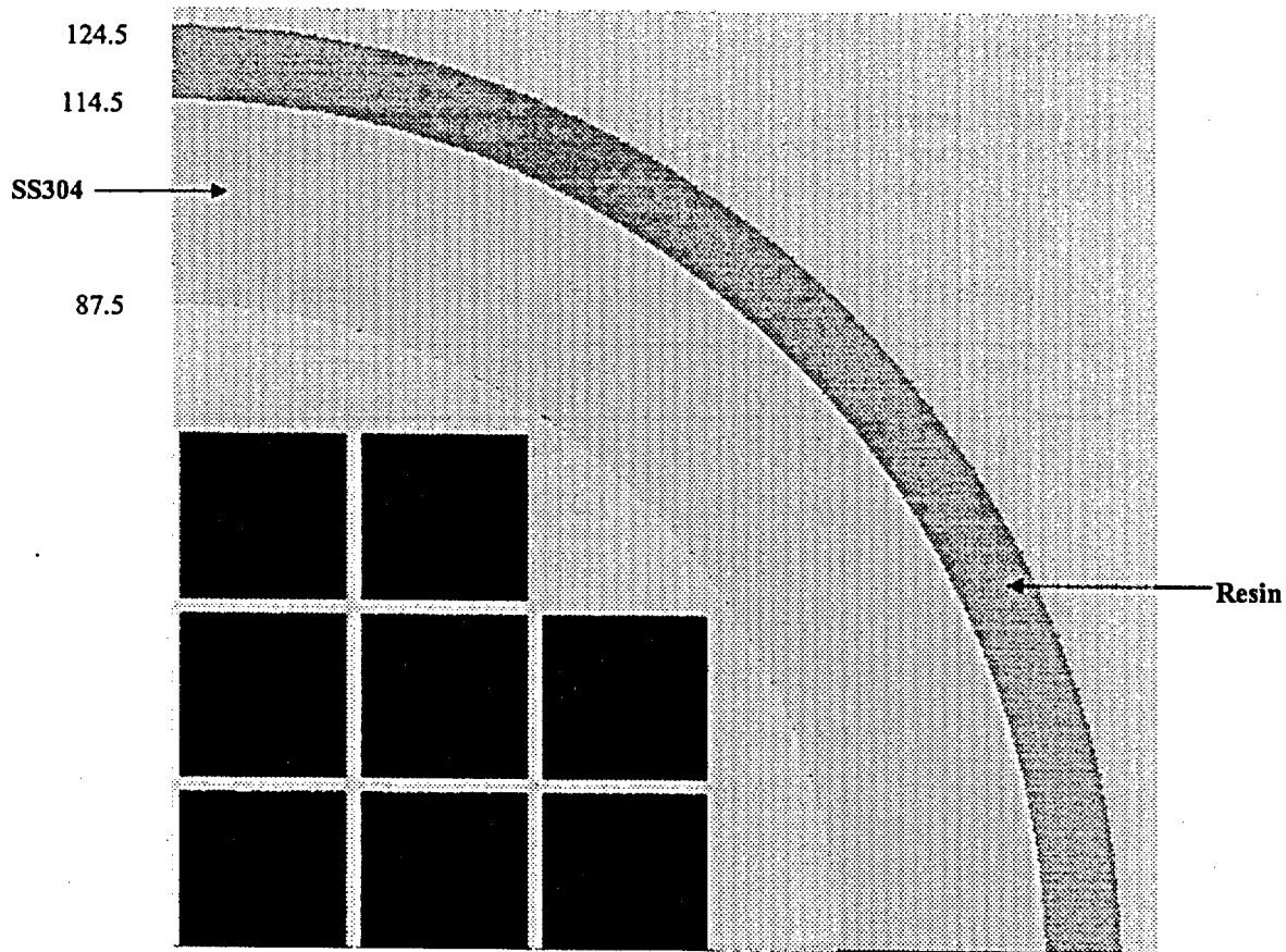
Figure C.1 Shielding model – radial (radii in cm)
