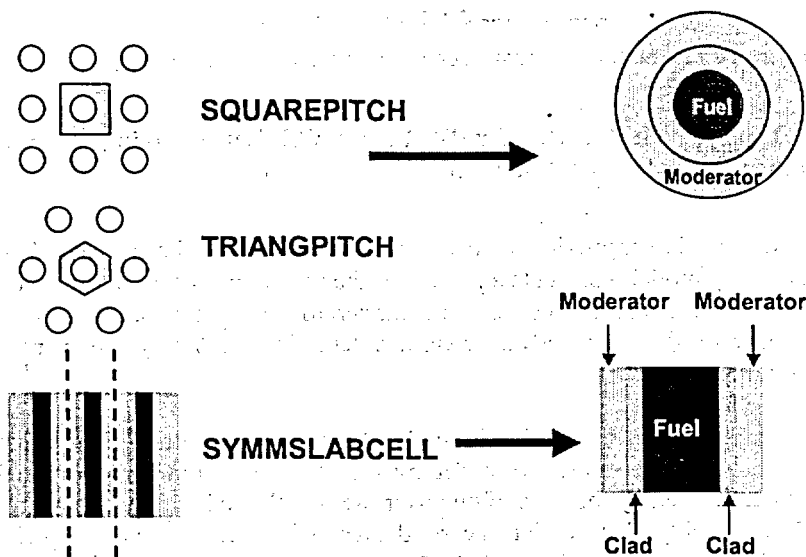
Figure A.3 Pin-cell model for representing the repeating lattice structure of a typical fuel assembly
