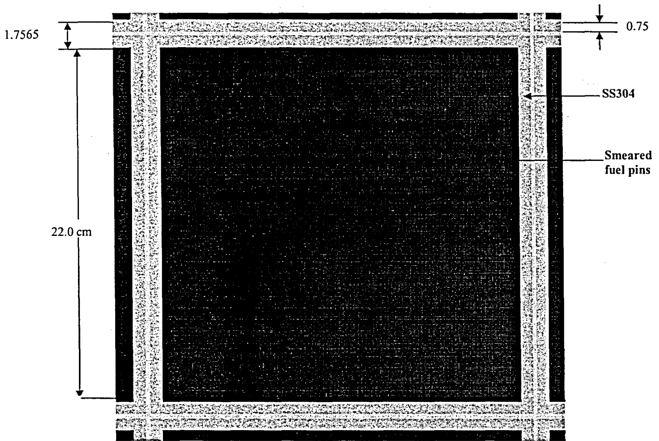
Figure C.3 GBC-32 detailed basket model (in cm)
