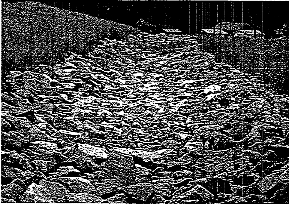
Figure F-2. Marginally-placed riprap
