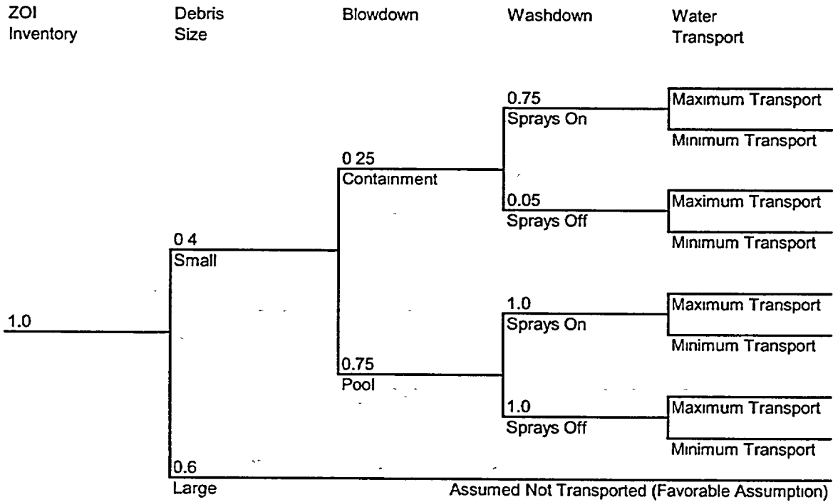
Figure 11 SLOCA Logic Tree—Washdown Transport Quantified
