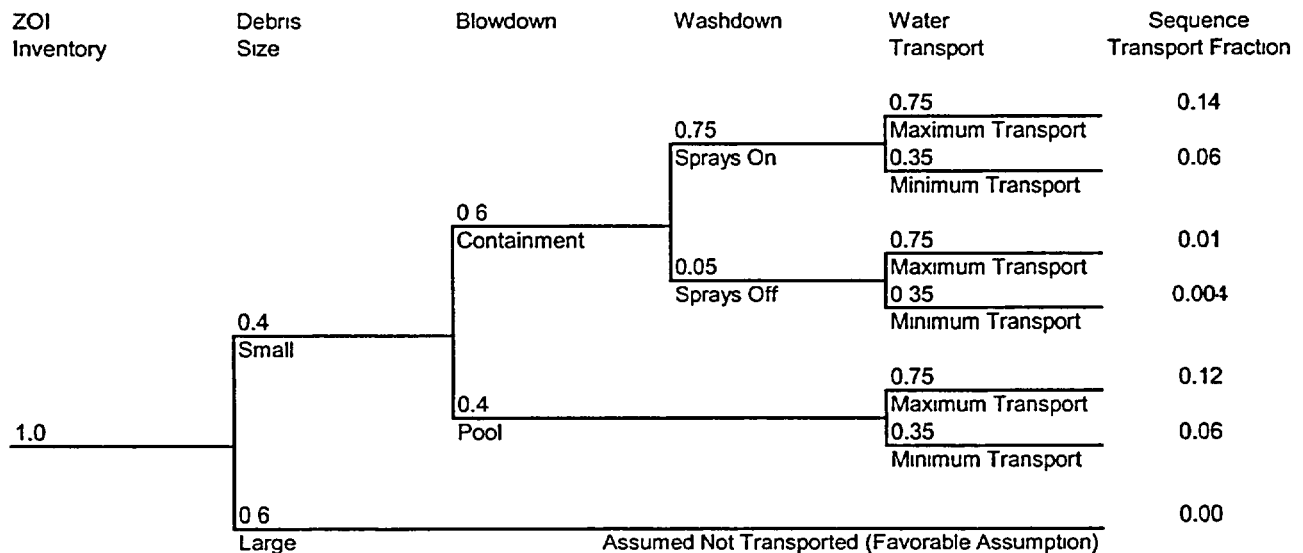
Figure 12 Quantified LLOCA Logic Tree
