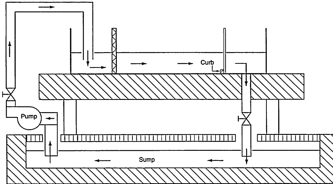
Figure 1 Schematic of Large Flume Assembly
