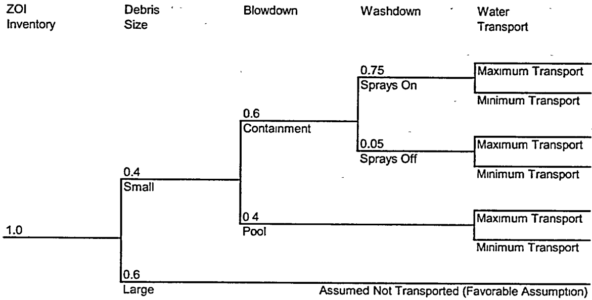
Figure 10 LLOCA Logic Tree—Washdown Transport Quantified
