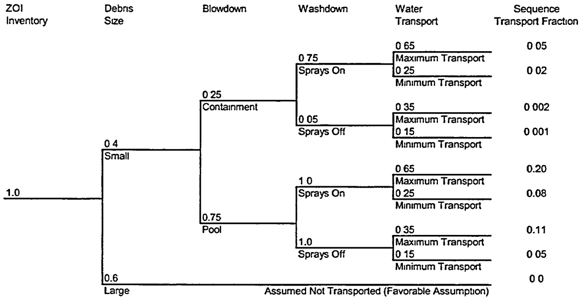
Figure 13 Quantified SLOCA Logic Tree
