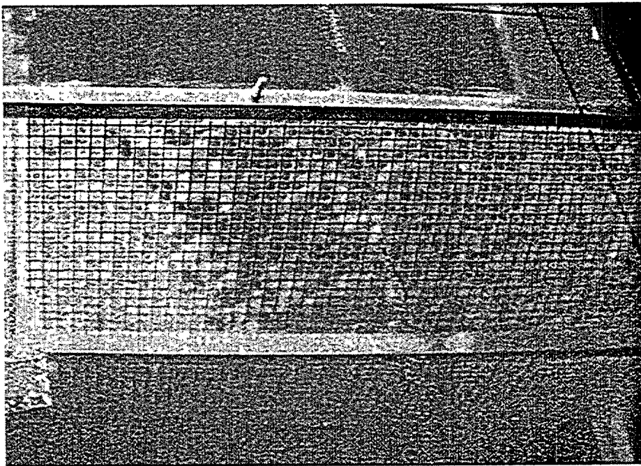
Figure 4 Thin Fiber Bed Beginning to Build on Vertical Screen of 1/4-in. Mesh Opening
