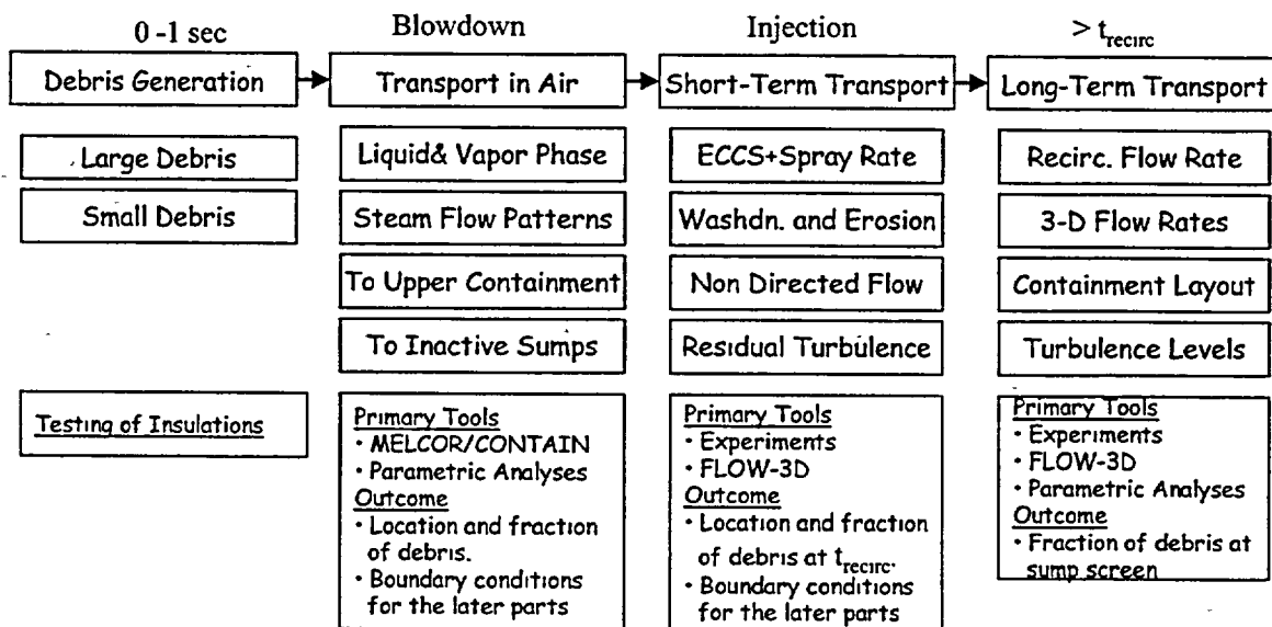
Figure 5 Debris Transport Phenomenology
