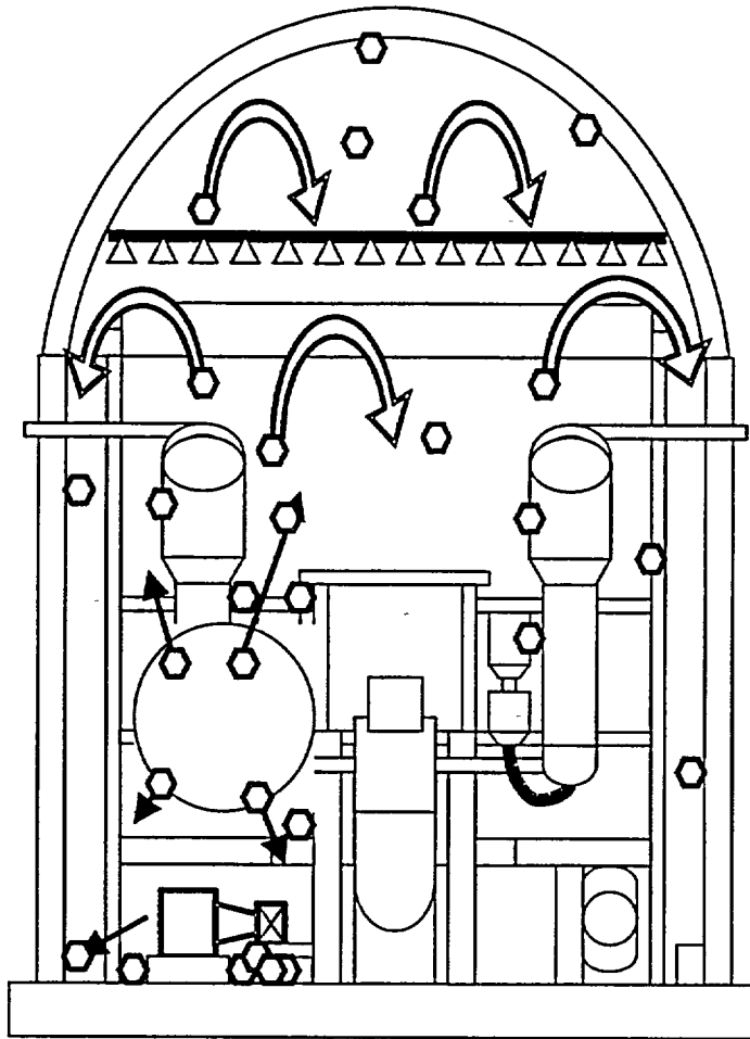
Figure 7 Debris Transport During LOCA Blowdown
