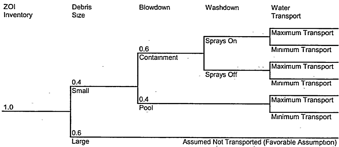
Figure 8 LLOCA Logic Tree—Blowdown Transport Quantified
