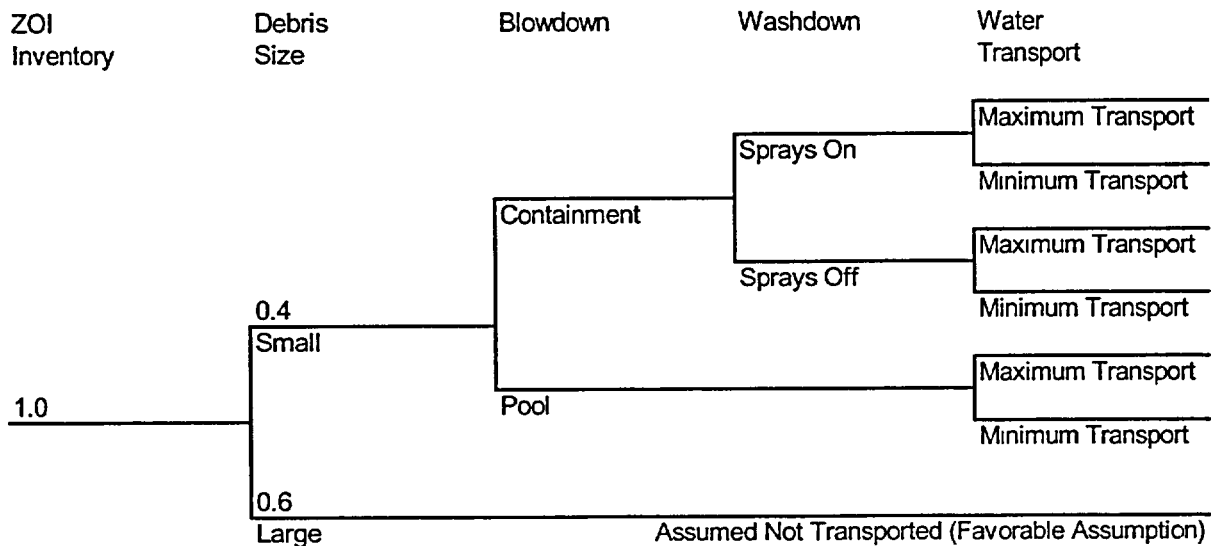
Figure 6 Logic Tree for Quantification of Debris Transport During a LOCA
