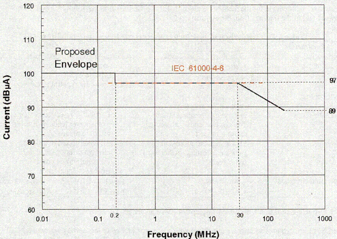
Fig. 6.6. High-frequency conducted susceptibility operating envelopes.
