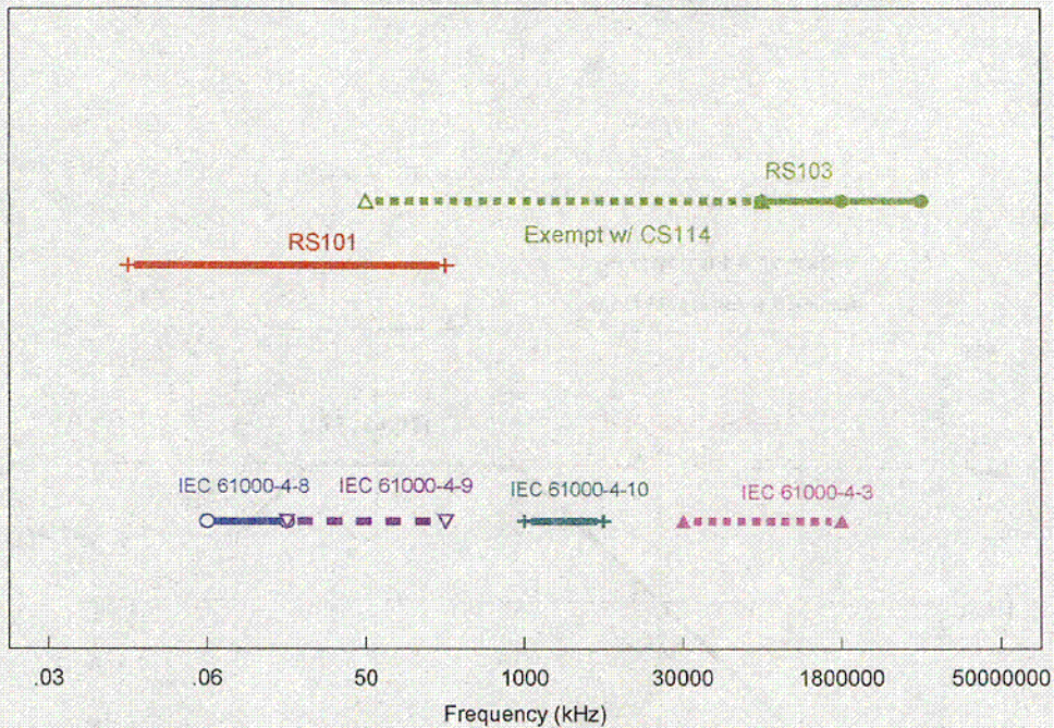
Fig. 7.1. Radiated susceptibility frequency coverage.
