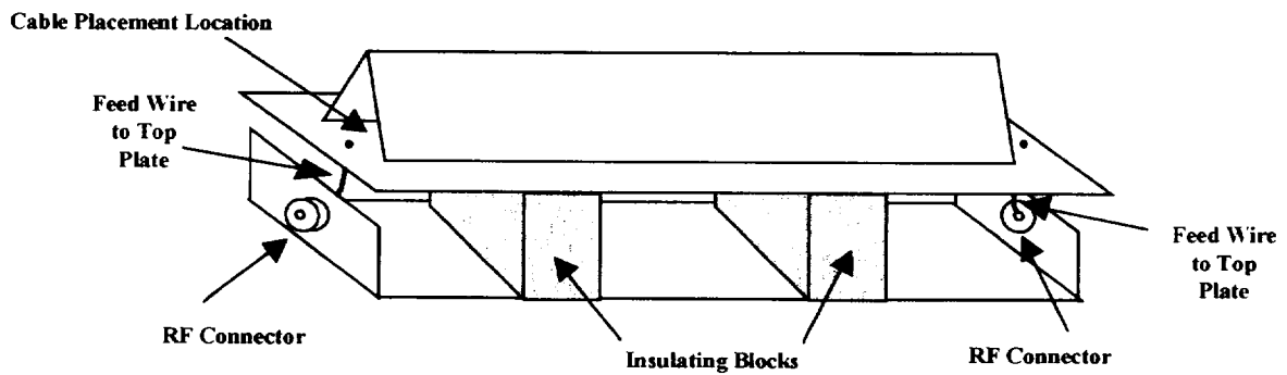
Fig. 6.10. IEC 61000-4-4 capacitive injection clamp.
