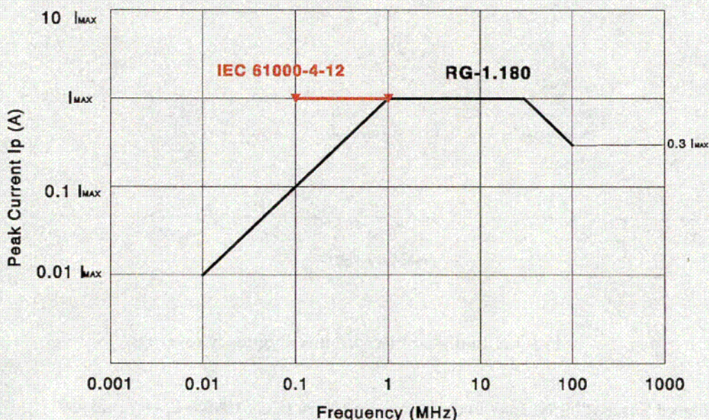
Fig. 6.14. Damped sinusoid conducted susceptibility operating envelopes.
