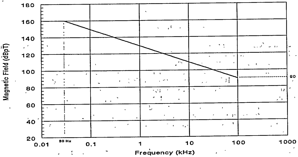
Fig. 5.3. RE101 operating envelope.
