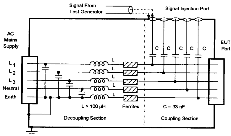
Fig. 6.11. IEC 61000-4-4 coupling/decoupling network.
