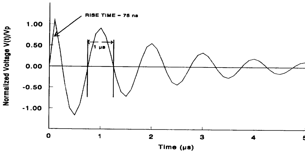
Fig. 6.13. Waveform of the damped oscillatory wave.
