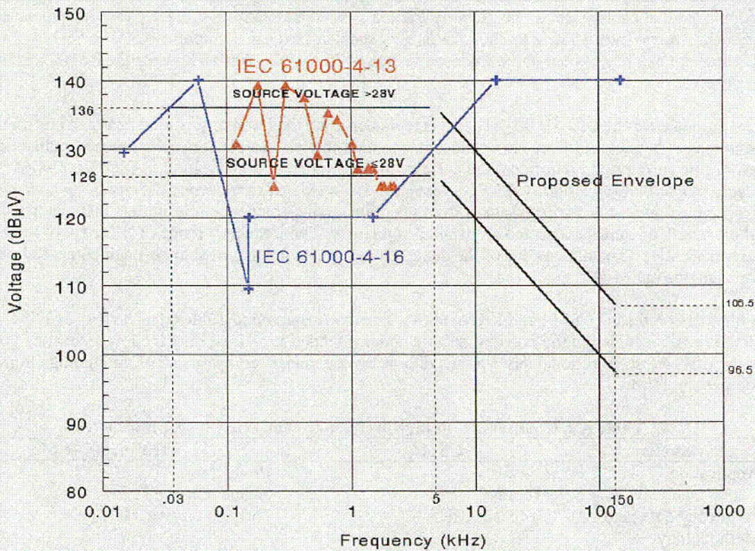
Fig. 6.3. Low-frequency susceptibility operating envelopes.
