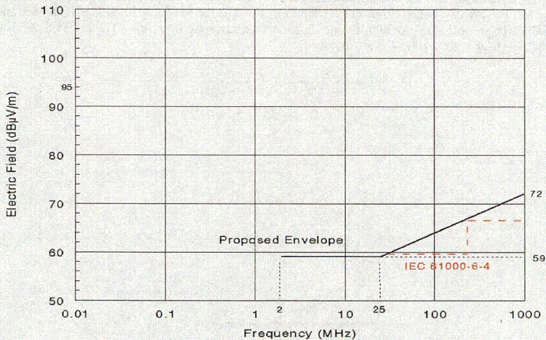
Fig. 5.6. RE102 operating envelope.
