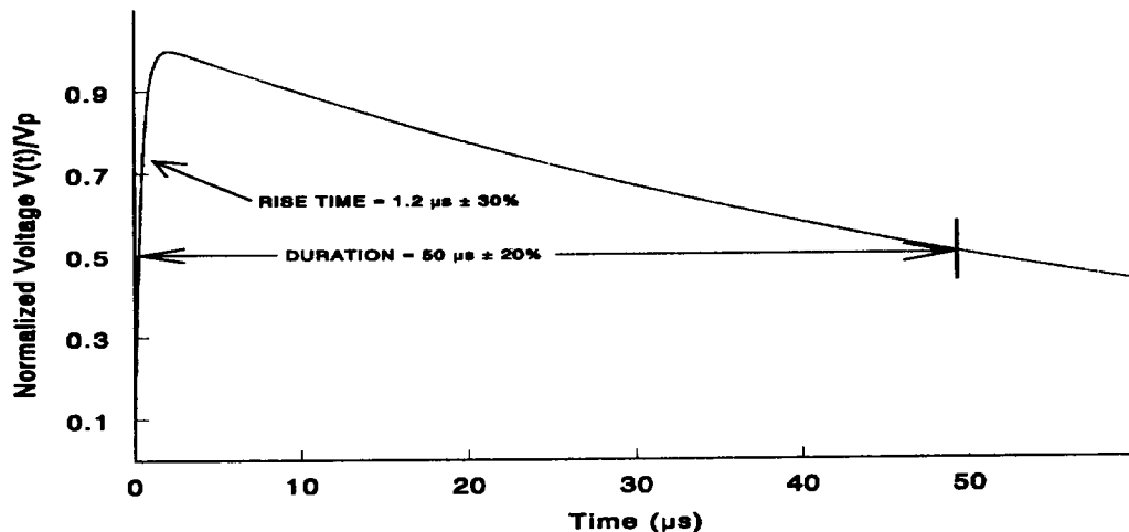
Fig. 8.2. Combination wave, open-circuit voltage.
