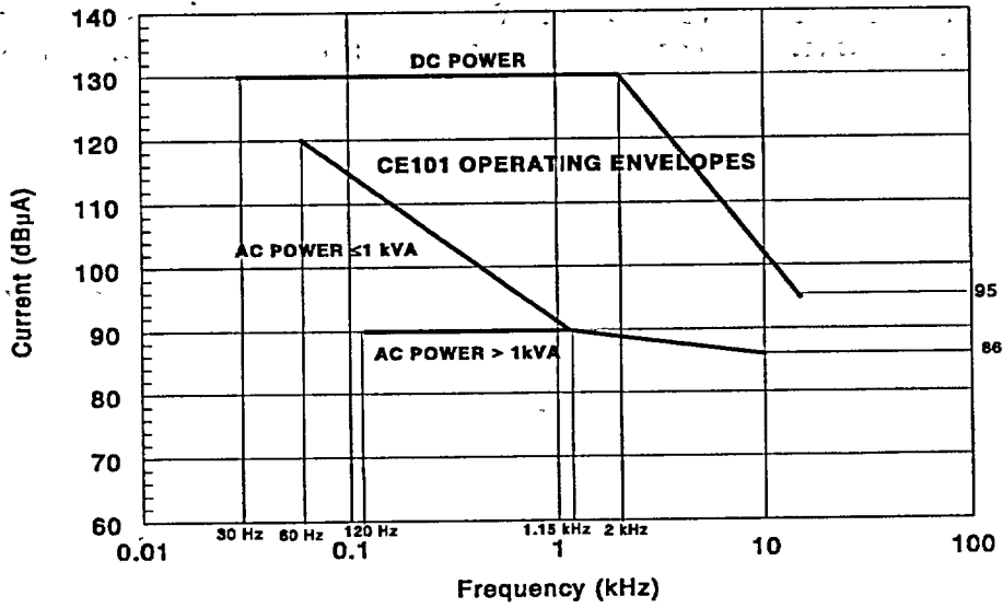
Fig. 5.2. CE101 operating envelope.
