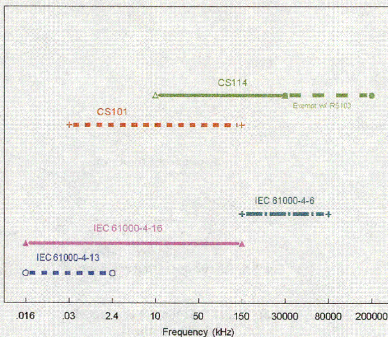
Fig. 6.1. Conducted susceptibility frequency coverage.
