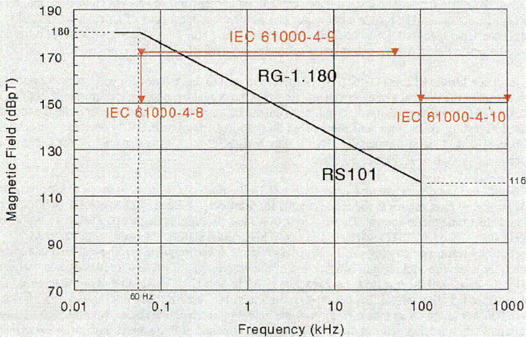
Fig. 7.2. Low-frequency radiated susceptibility operating envelopes.
