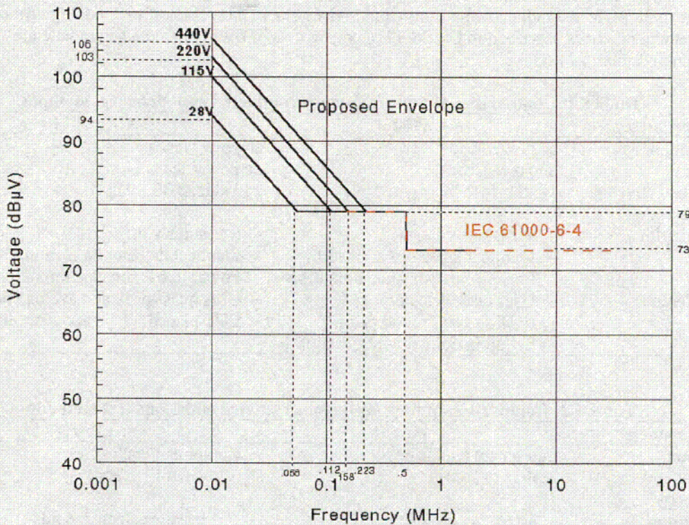
Fig. 5.5. CE102 operating envelope.
