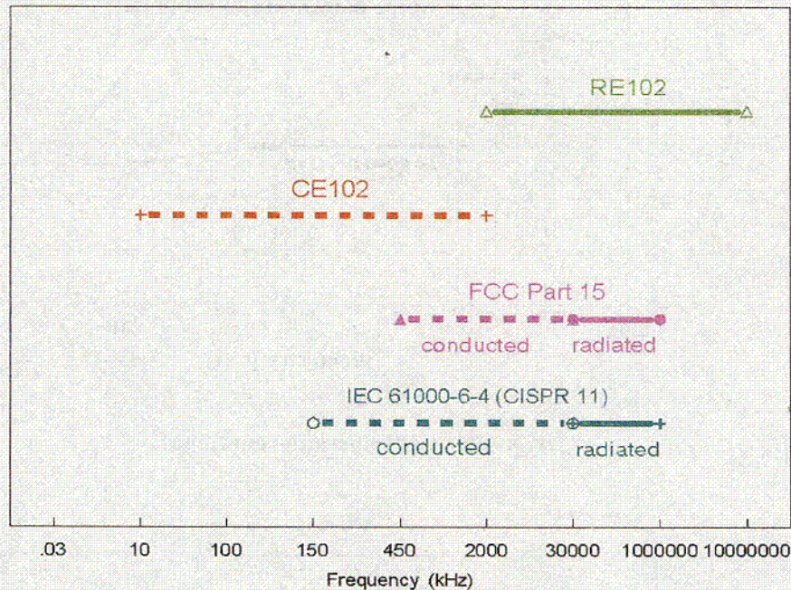
Fig. 5.4. High frequency emissions coverage.
