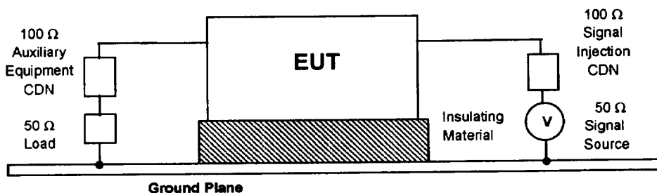
Fig. 6.5. IEC 61000-4-6 signal injection setup.
