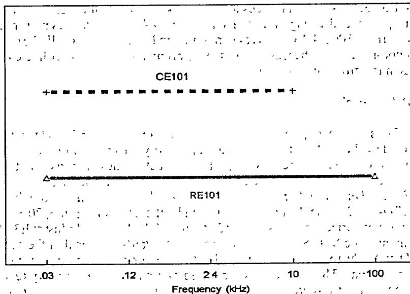
Fig.5.1. Low-frequency emissions coverage.
