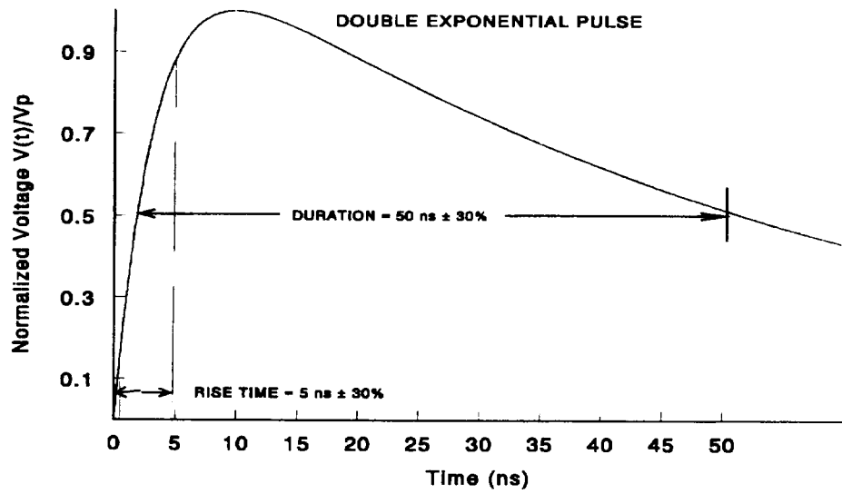
Fig. 6.9. Waveform of fast transient.
