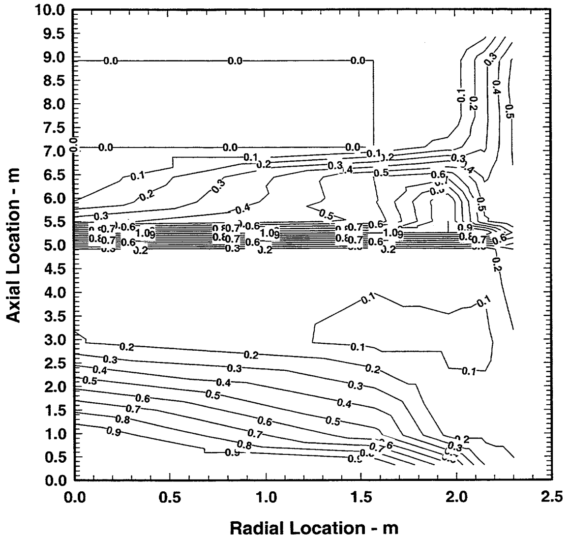
Figure 12-25. Core Material Volume Fraction at 5000 Seconds
