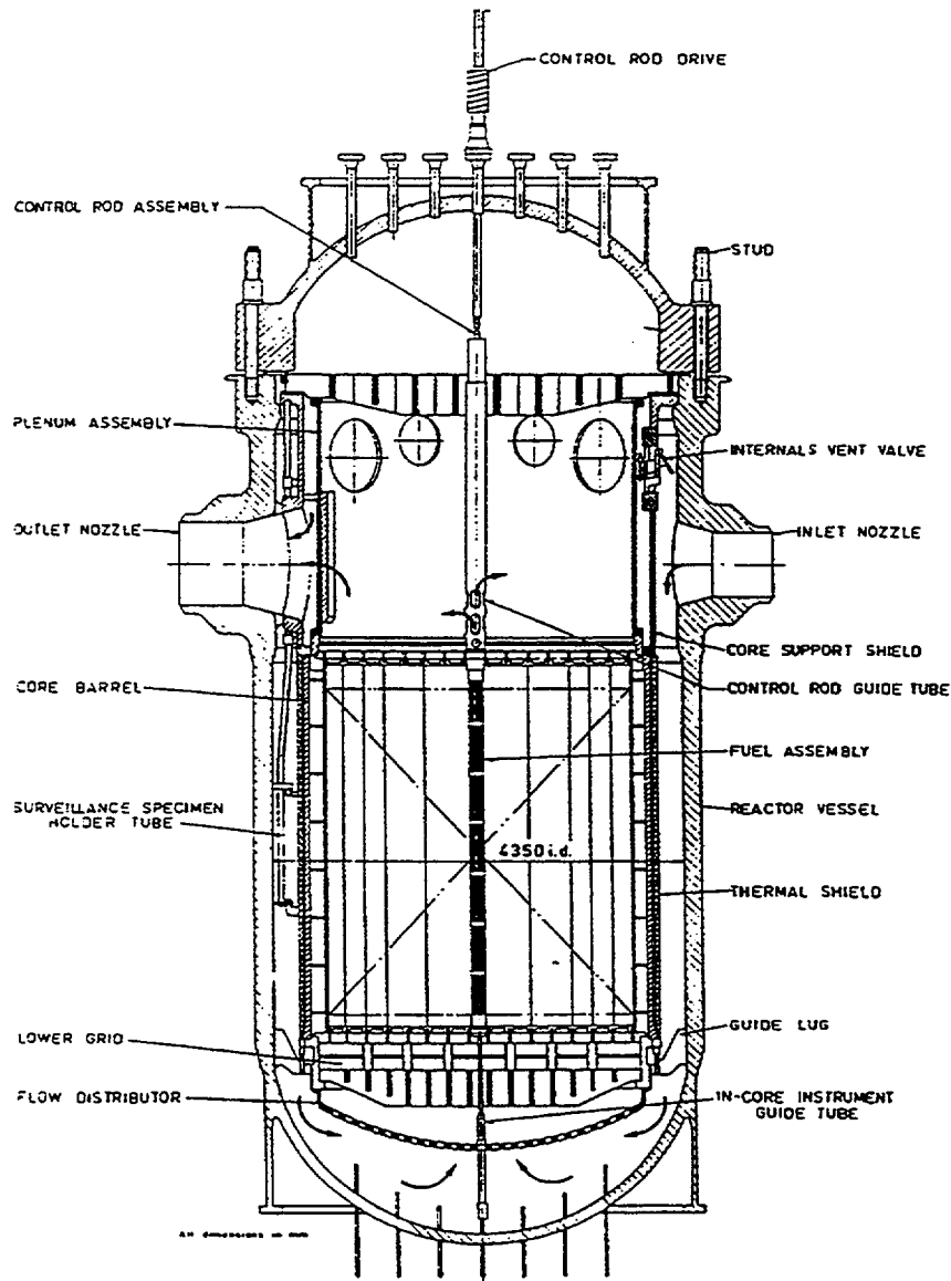
Figure 13-1. Cross-Section of the TMI-2 Reactor Vessel
