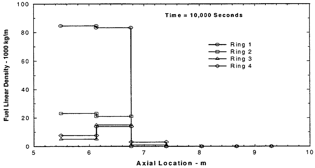
Figure 12-5. Core Material Disposition at 10,000 Seconds—Version 1.8.5 Calculation
