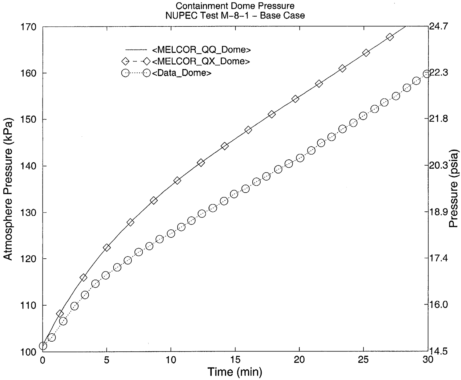
Figure 1-4. Containment Pressure Response
