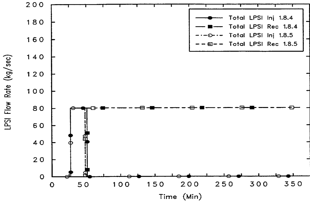
Figure 9-13. Zion LB LOCA: LPSI Flow
