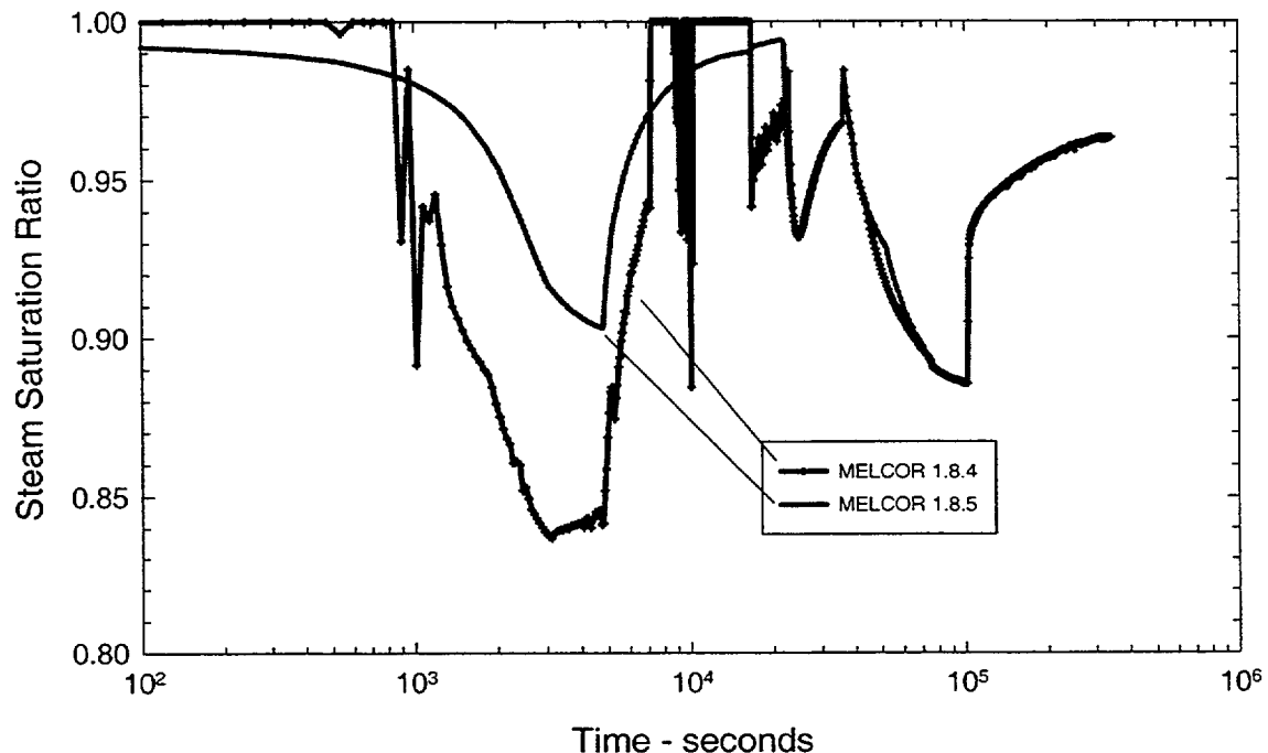
Figure 3-7. Test Vessel Relative Humidity
