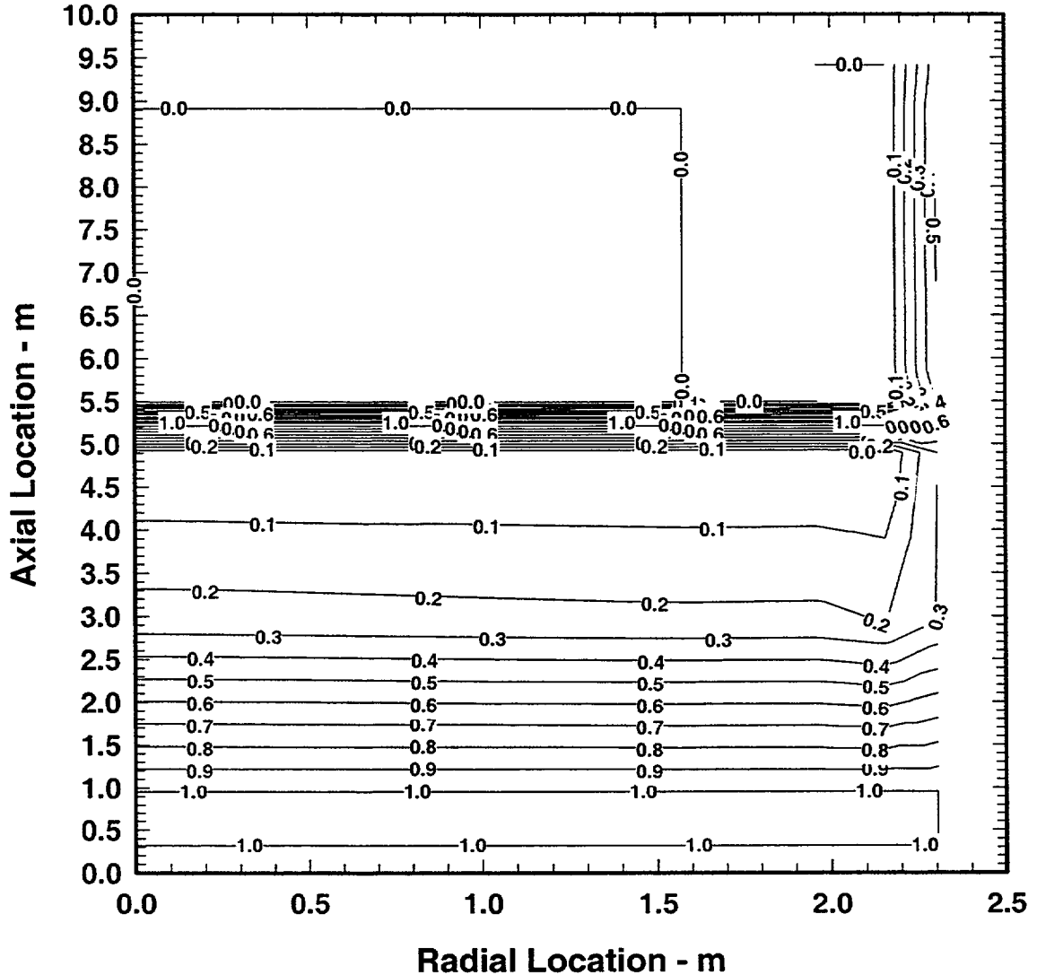
Figure 11-25. Core Material Volume Fraction at 5000 Seconds
