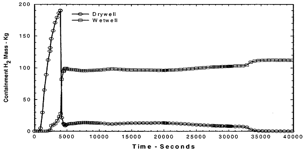
Figure 11-14. Hydrogen in Containment—Version 1.8.4 Calculation
