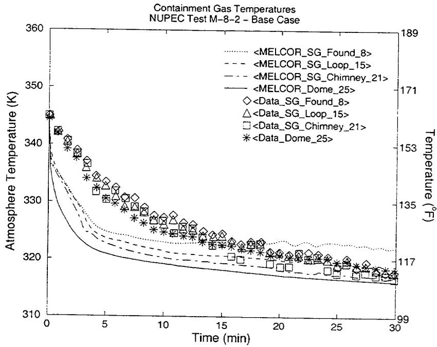
Figure 2-14. Gas Temperature Response in CVs 8, 15, 21, and 25: MELCOR Versus Experiment
