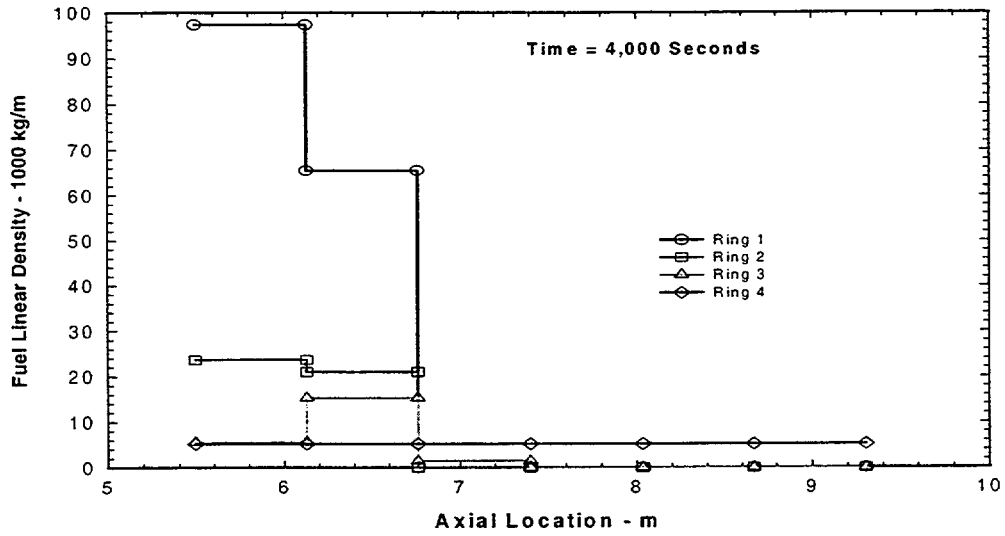
Figure 11-5. Core Material Disposition at 4000 Seconds—Version 1.8.5 Calculation
