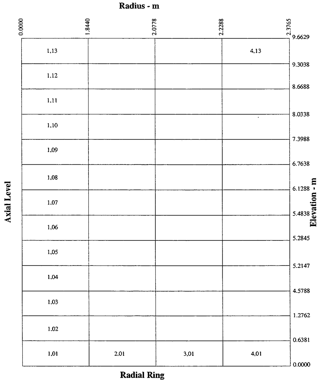
Figure 11-2. Core Nodalization
