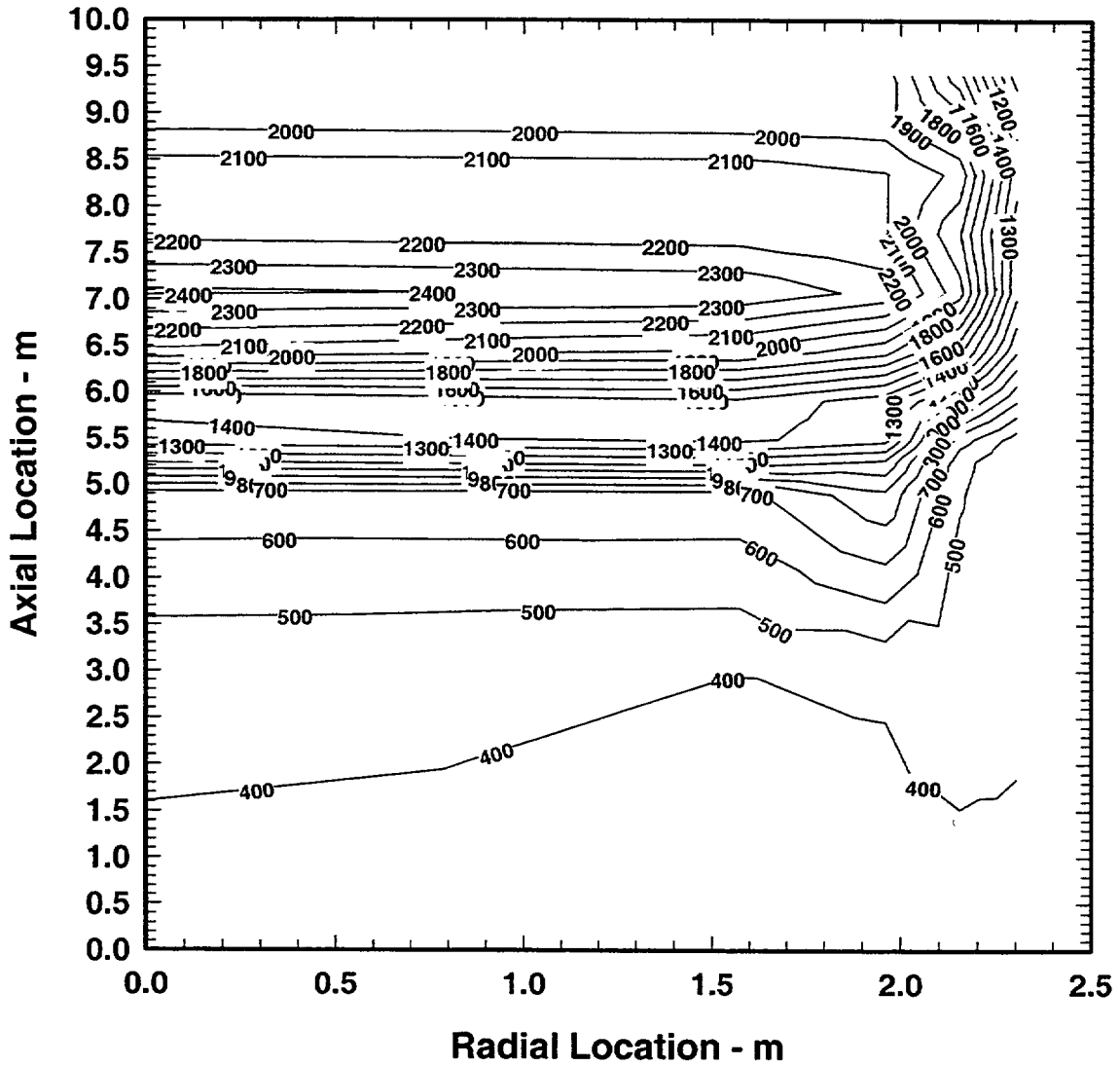
Figure 12-27. Core Temperature Profile at 4000 Seconds
