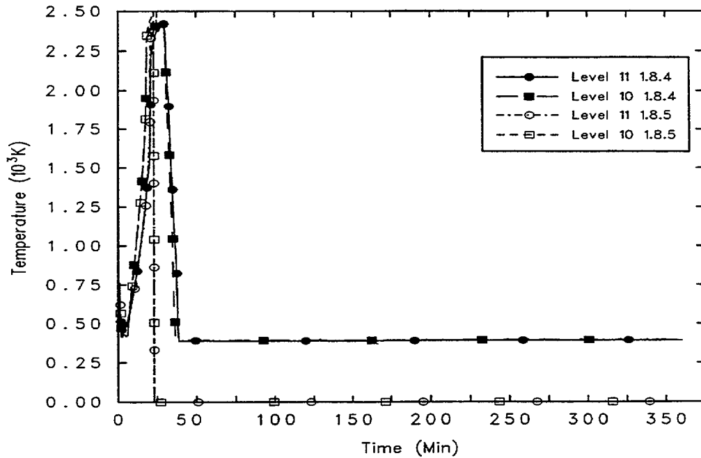
Figure 9-10. Zion LB LOCA: Ring 1 TAF Fuel Temperatures (long term)
