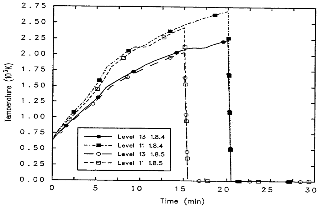
Figure 8-8. Surry LB LOCA: Ring 1 Fuel Temperature (top of core)
