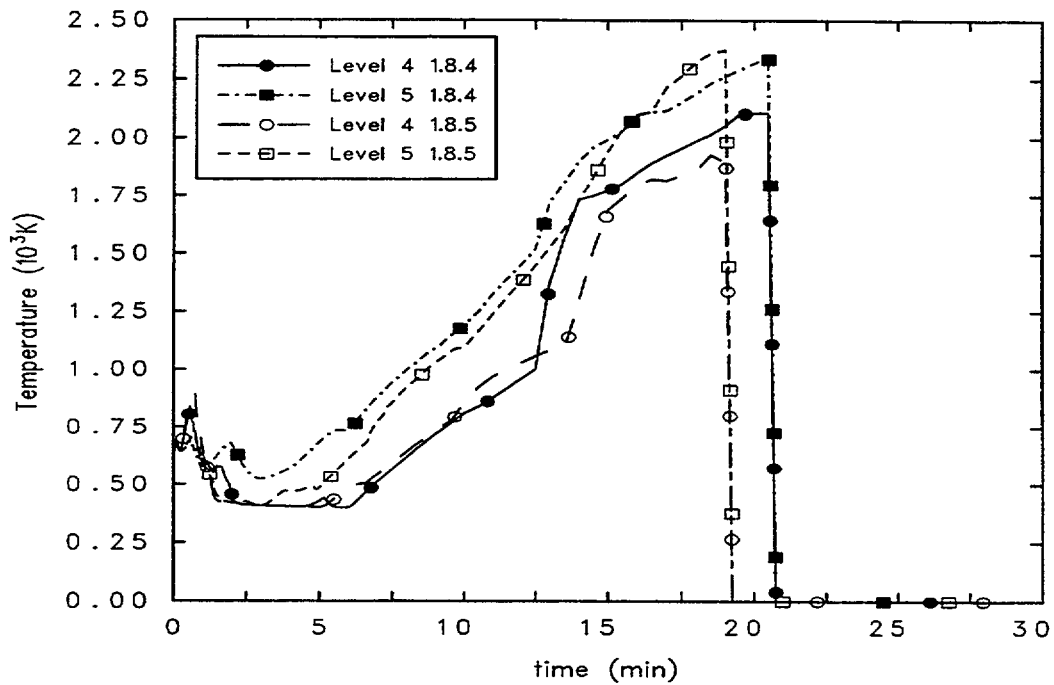
Figure 8-10. Surry LB LOCA: Ring 1 Fuel Temperature (bottom of core)
