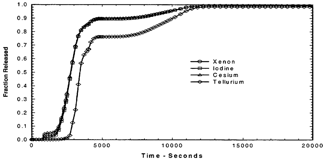
Figure 11-18. Fuel Fission Product Releases—Version 1.8.4 Calculation
