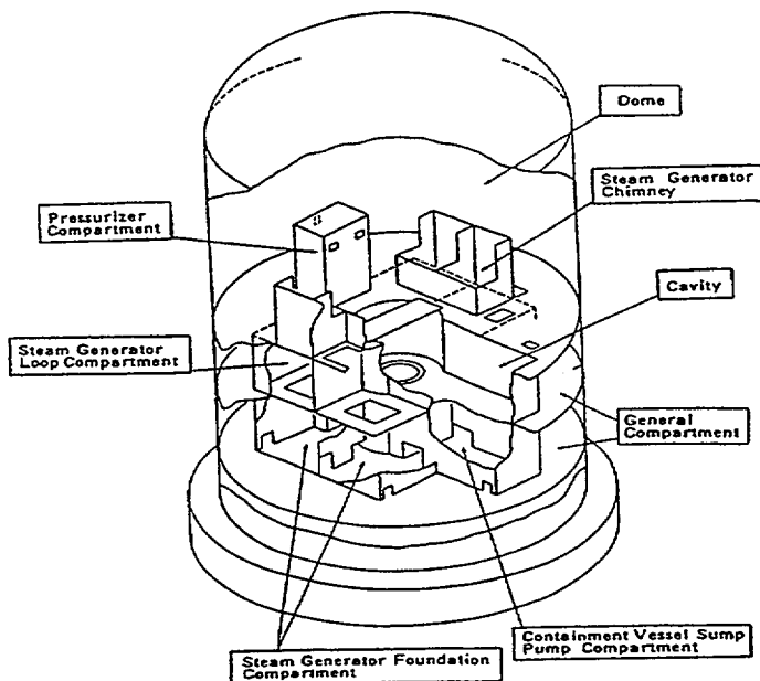
Figure 2-1. NUPEC 1/4-Scale Containment Mixing Facility [1]
