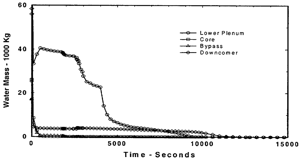
Figure 11-9. Core Coolant Inventory—Version 1.8.5 Calculation
