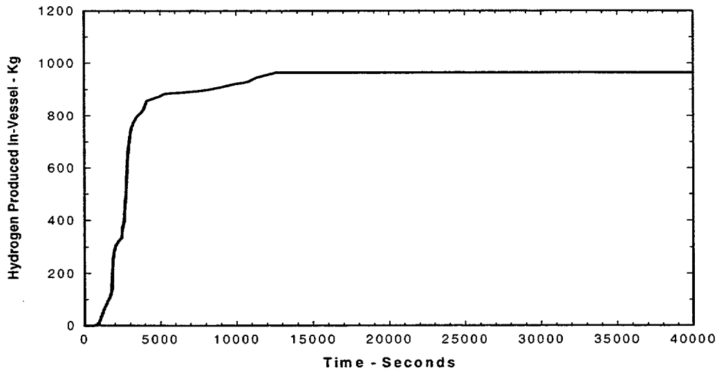
Figure 11-11. In-core Hydrogen Produced—Version 1.8.5 Calculation
