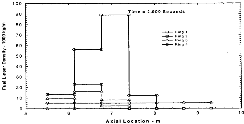
Figure 11-6. Core Material Disposition at 4000 Seconds—Version 1.8.4 Calculation
