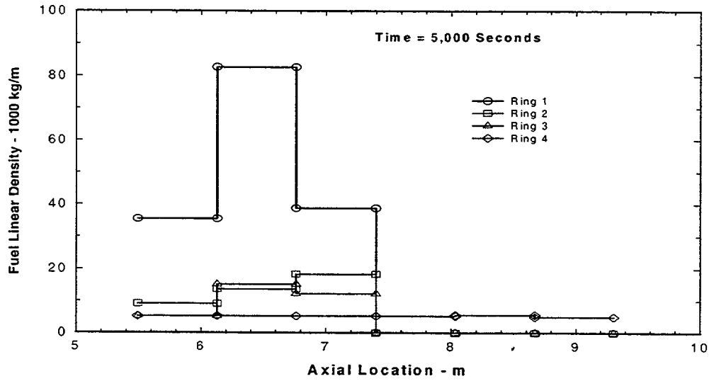
Figure 12-3. Core Material Disposition at 5000 Seconds– Version 1.8.5 Calculation
