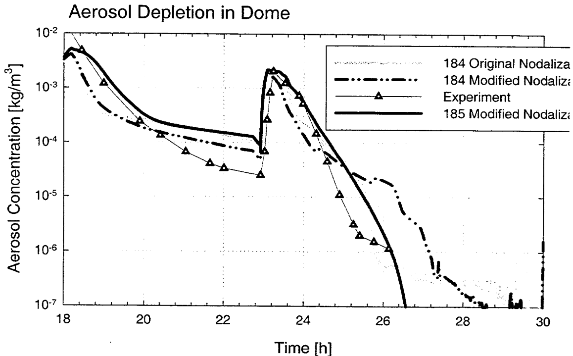
Figure 4-10. Aerosol Depletion Behavior in Dome, as Predicted by MELCOR
