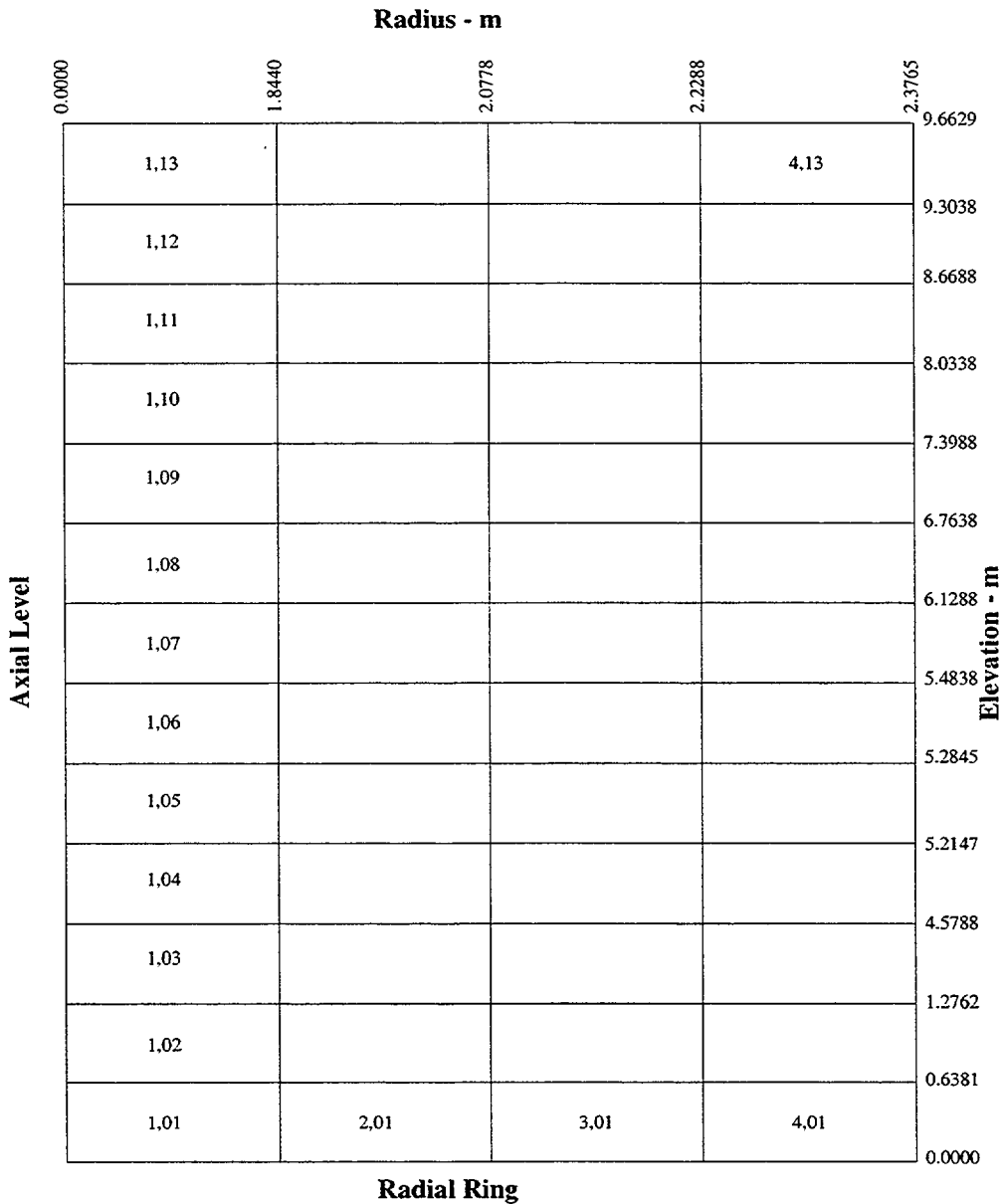
Figure 12-2. Core Nodalization
