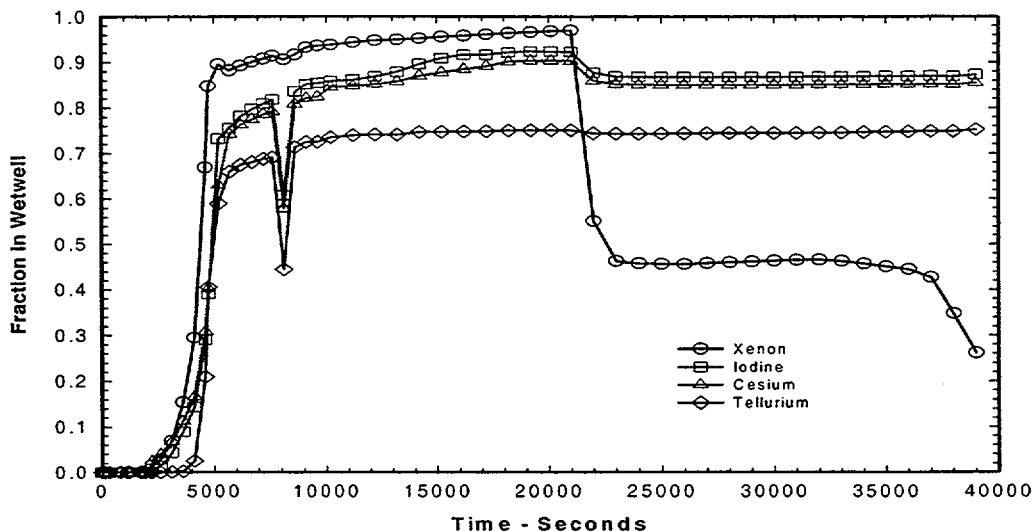
Figure 12-19. Fission Products in Containment—Version 1.8.5 Calculation
