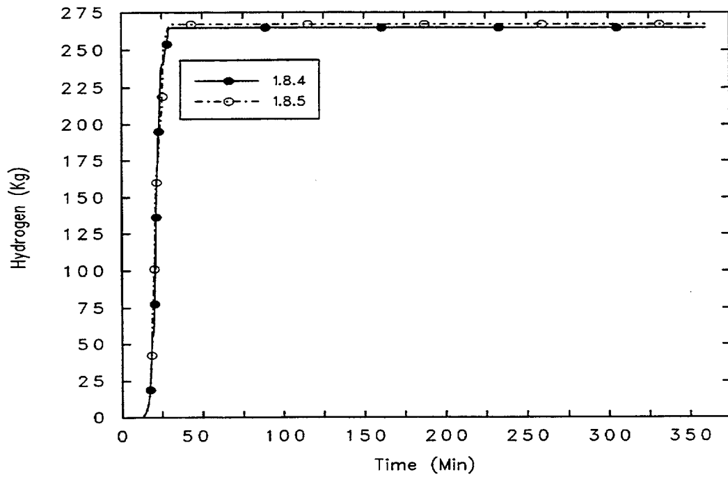
Figure 9-14. Zion LB LOCA: In-Vessel Hydrogen Production
