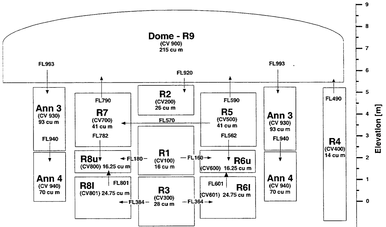
Figure 4-6. Modified Nodalization Where R6 and R8 are Divided into Upper and Lower Regions
