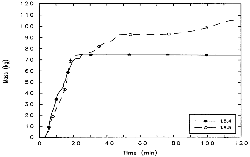
Figure 8-11. Surry LB LOCA: In-Vessel Hydrogen Production
