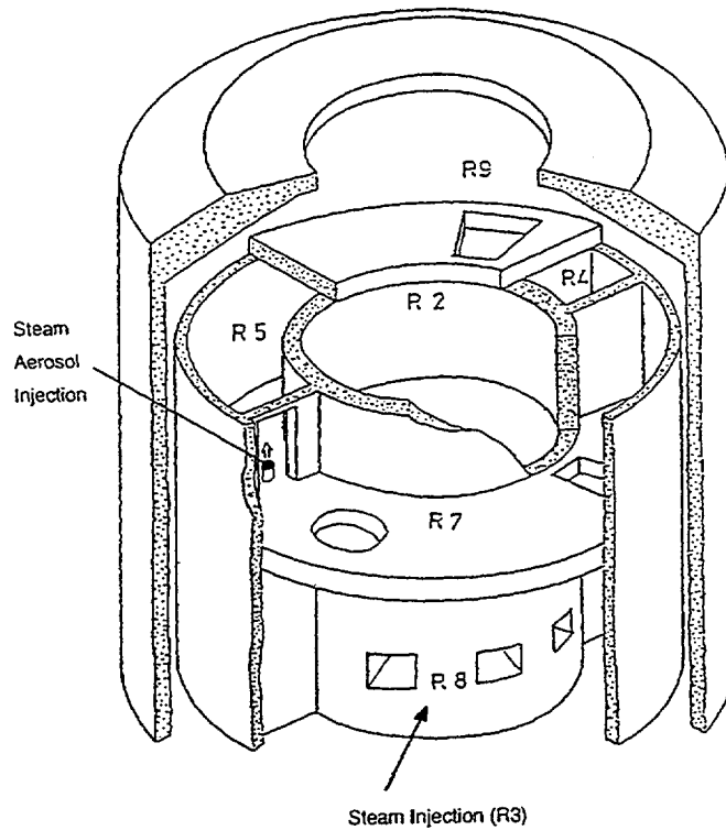
Figure 4-1. Schematic of the BMC Facility
