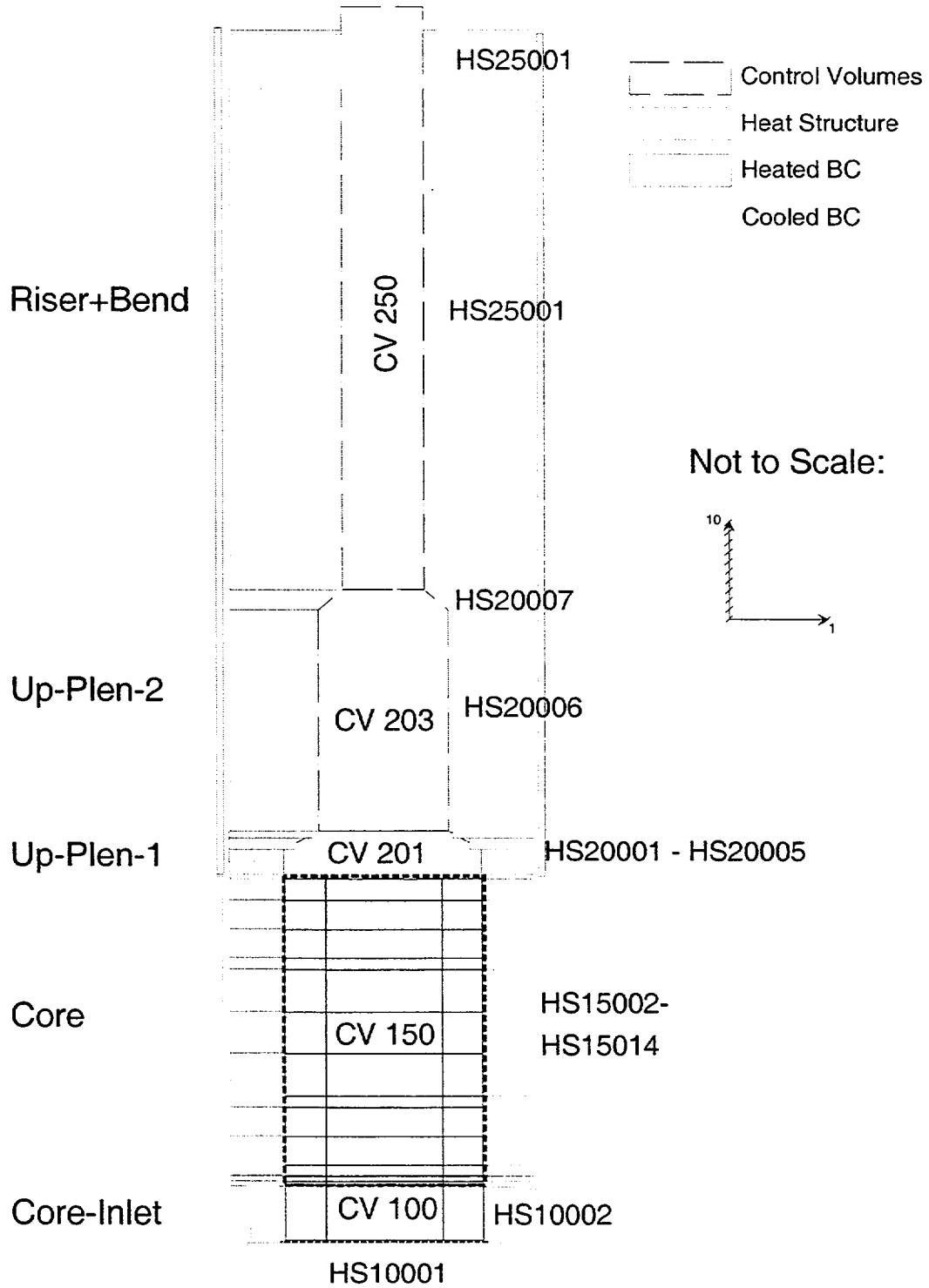
Figure 7-1. MELCOR FPT-1 Test Section Nodalization
