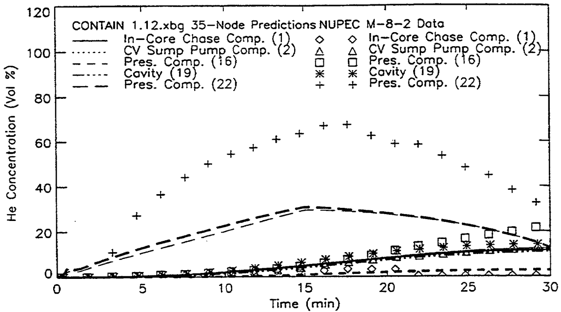
Figure 2-12. Helium Concentrations in Cells 1, 2, 16, 19, and 22: CONTAIN Versus Experiment [2]
