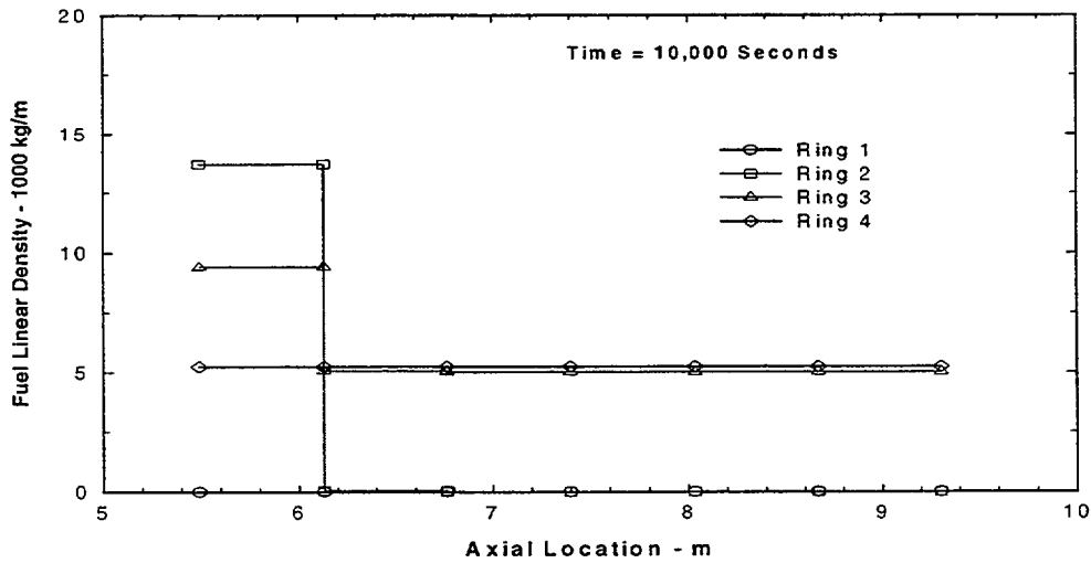
Figure 12-6. Core Material Disposition at 10,000 Seconds—Version 1.8.4 Calculation
