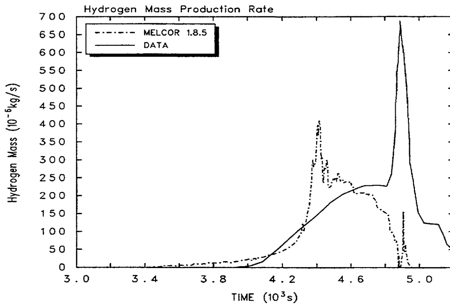
Figure 5-8. Measured and Calculated Hydrogen Generation Rate
