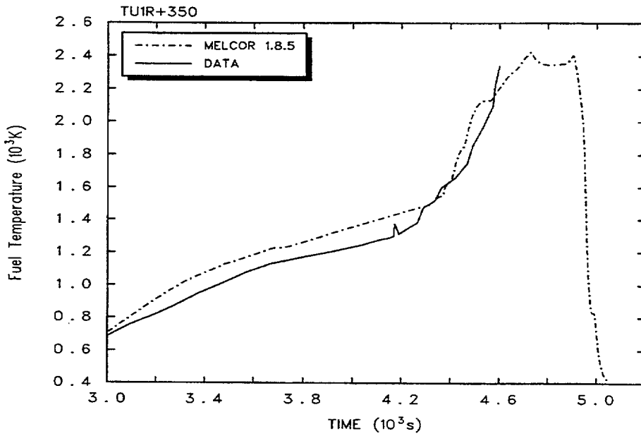
Figure 5-3. Measured and Calculated Fuel Temperature at 350 mm
