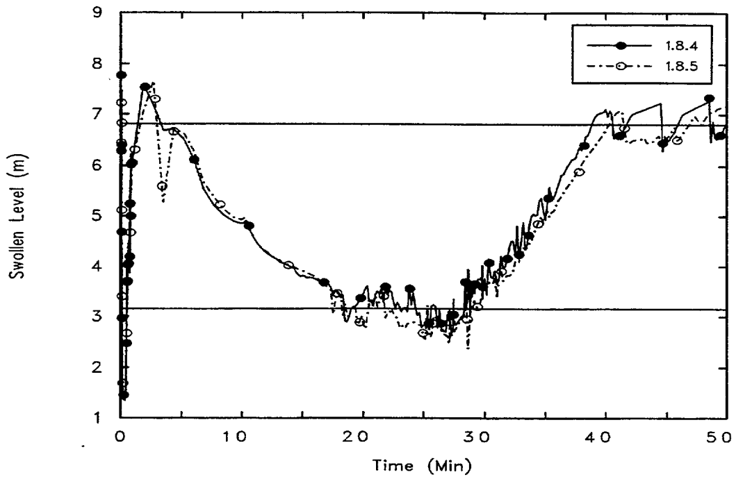
Figure 9-4. Zion LB LOCA: Reactor Water Level (short term)
