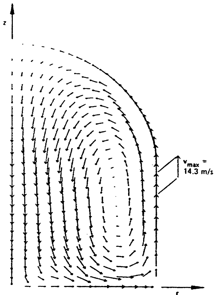
Figure 2-4. Flow Patterns in Containment During Spray Operation [2]
