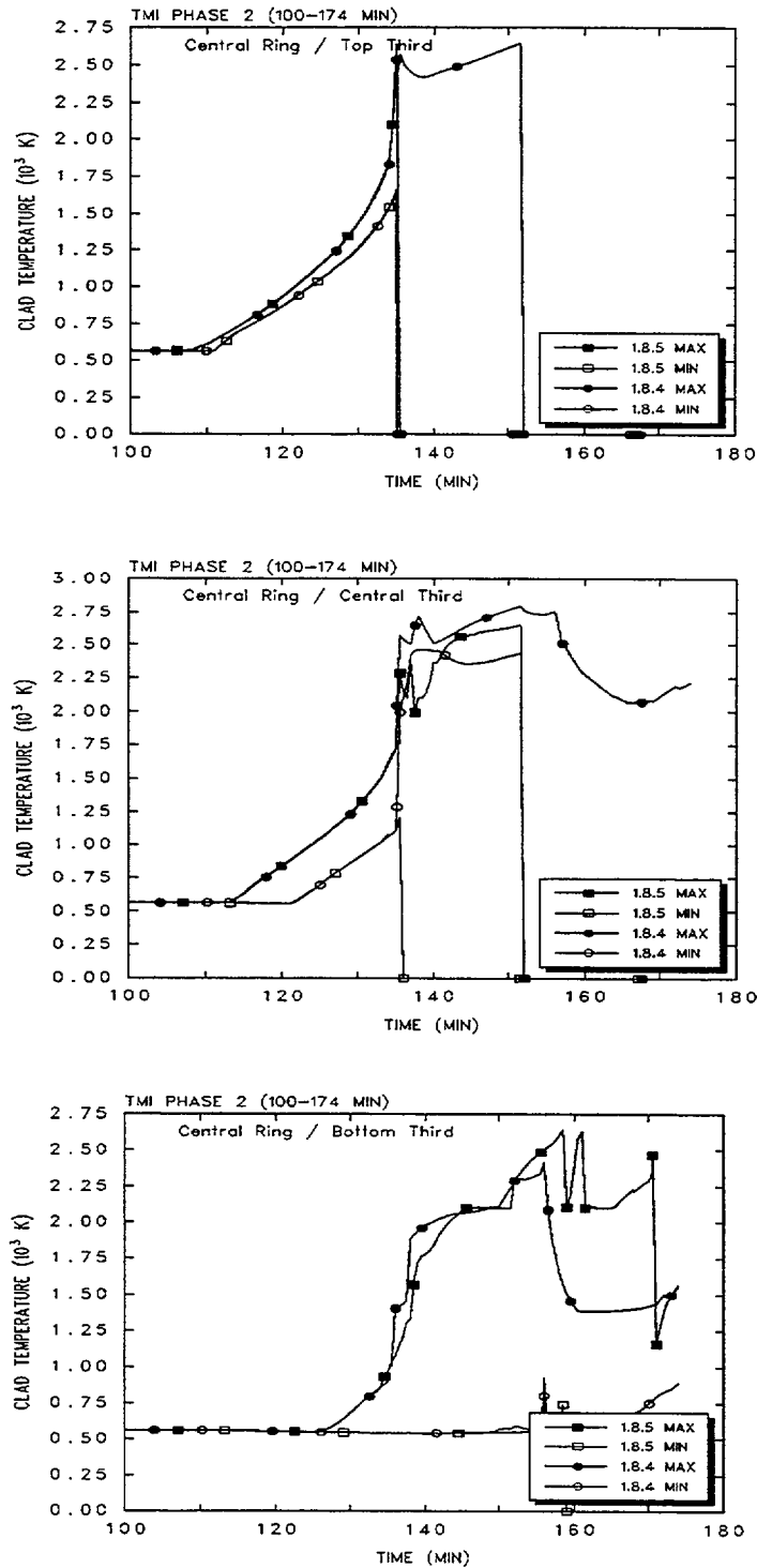
Figure 13-6. Cladding Temperatures
