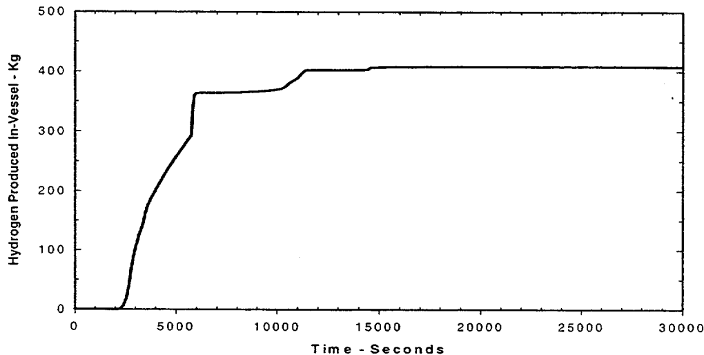
Figure 12-12. In-core Hydrogen Produced—Version 1.8.4 Calculation
