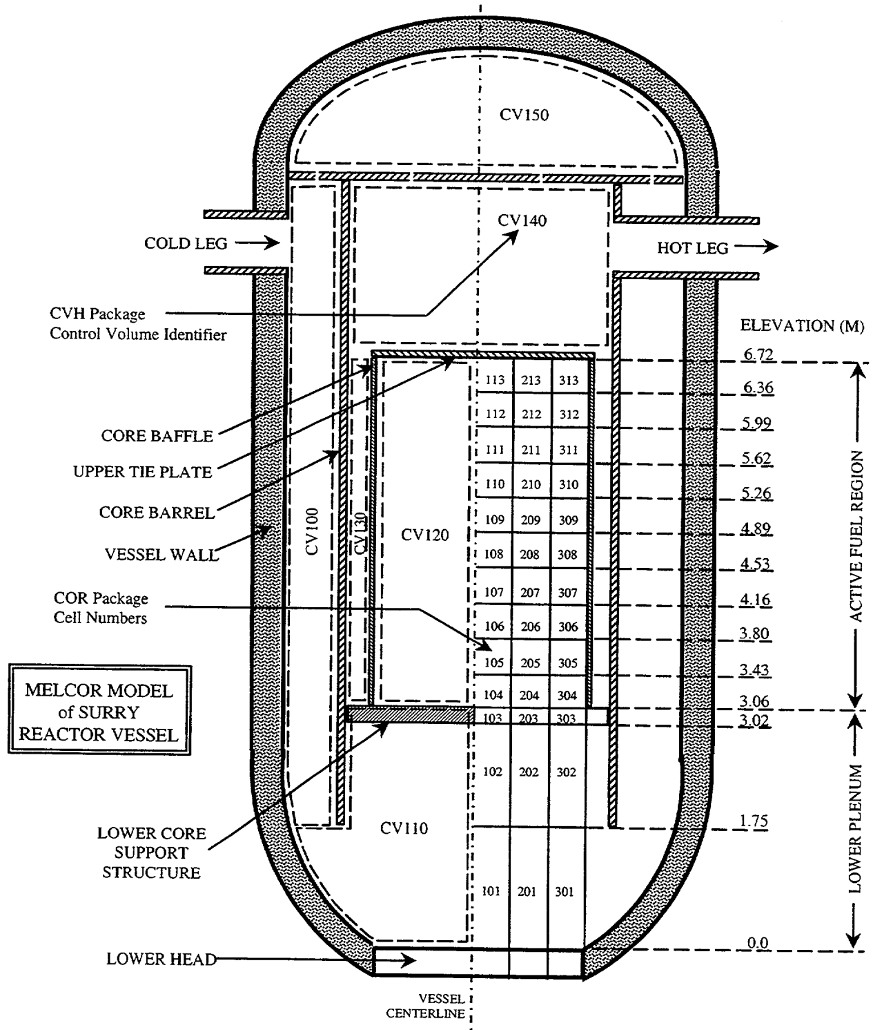
Figure 8-3. MELCOR Core Configuration for Surry Plant
