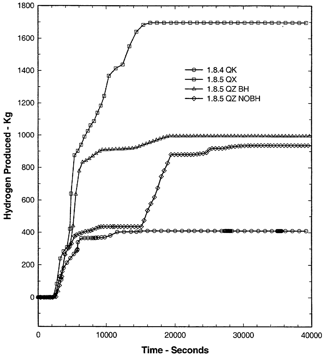
Figure 12-30 Comparison of Total H 2 Production
