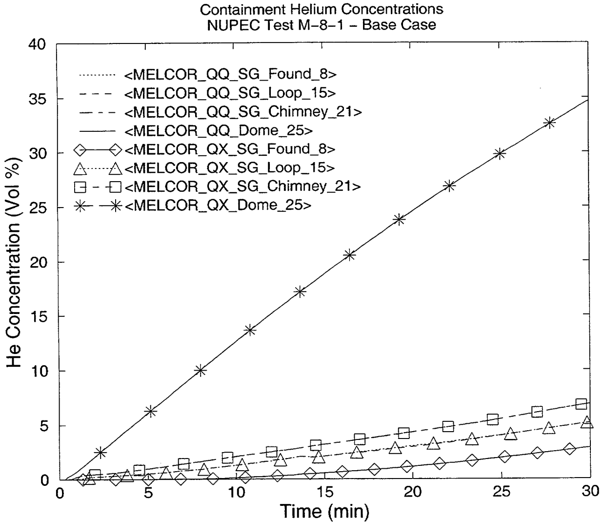
Figure 1-8. Containment He Concentrations (comparison to MELCOR 1.8.4)
