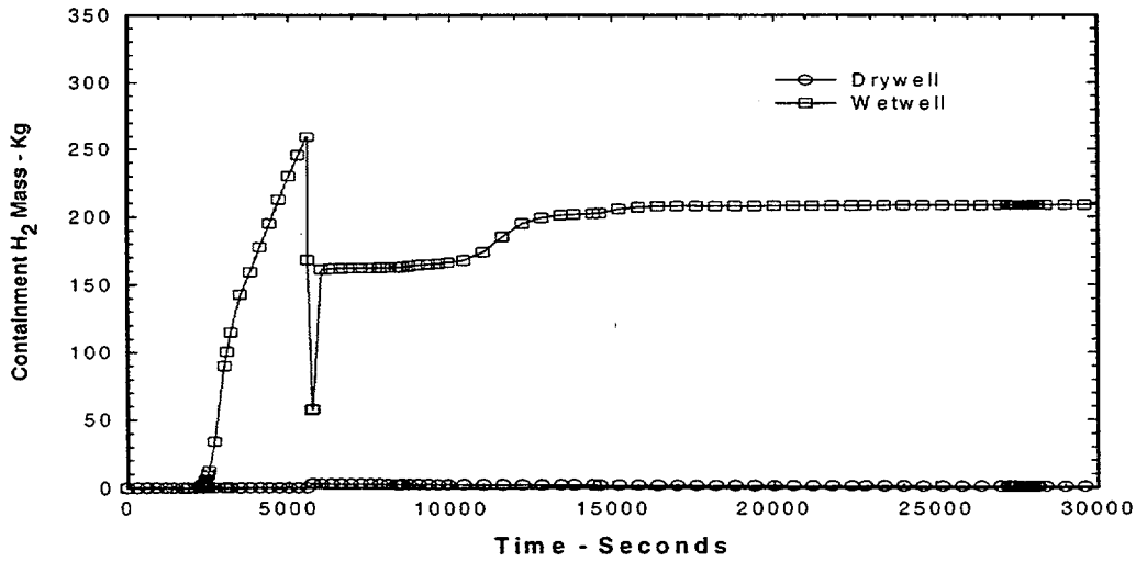
Figure 12-14. Hydrogen in Containment—Version 1.8.4 Calculation
