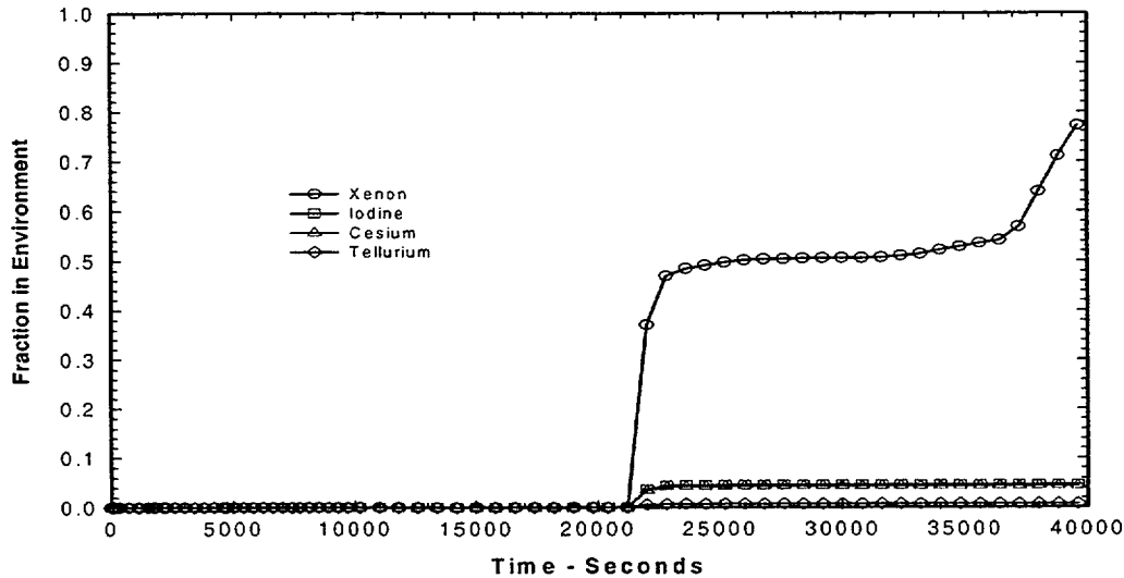
Figure 12-21. Fission Products Released into Environment—Version 1.8.5
