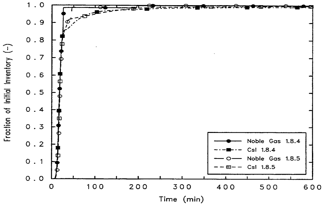
Figure 8-13. Surry LB LOCA: Noble Gas and Csl Release from Fuel
