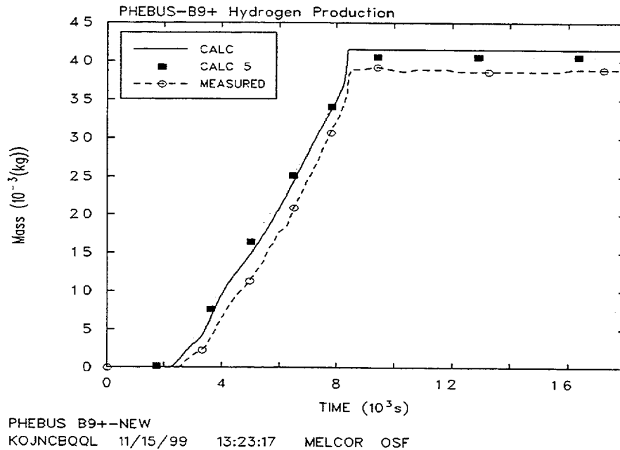
Figure 6-4. MELCOR 1.8.4 and 1.8.5 Calculated Hydrogen Production and Data
