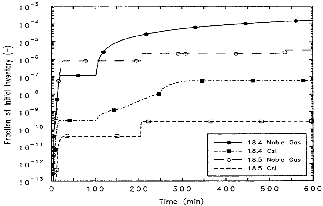
Figure 8-15. Surry LB LOCA: Noble Gas and Csl Environmental Release
