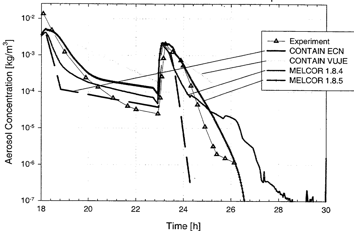
Figure 4-13. Aerosol Depletion Predicted by CONTAIN Users With Comparison to MELCOR
