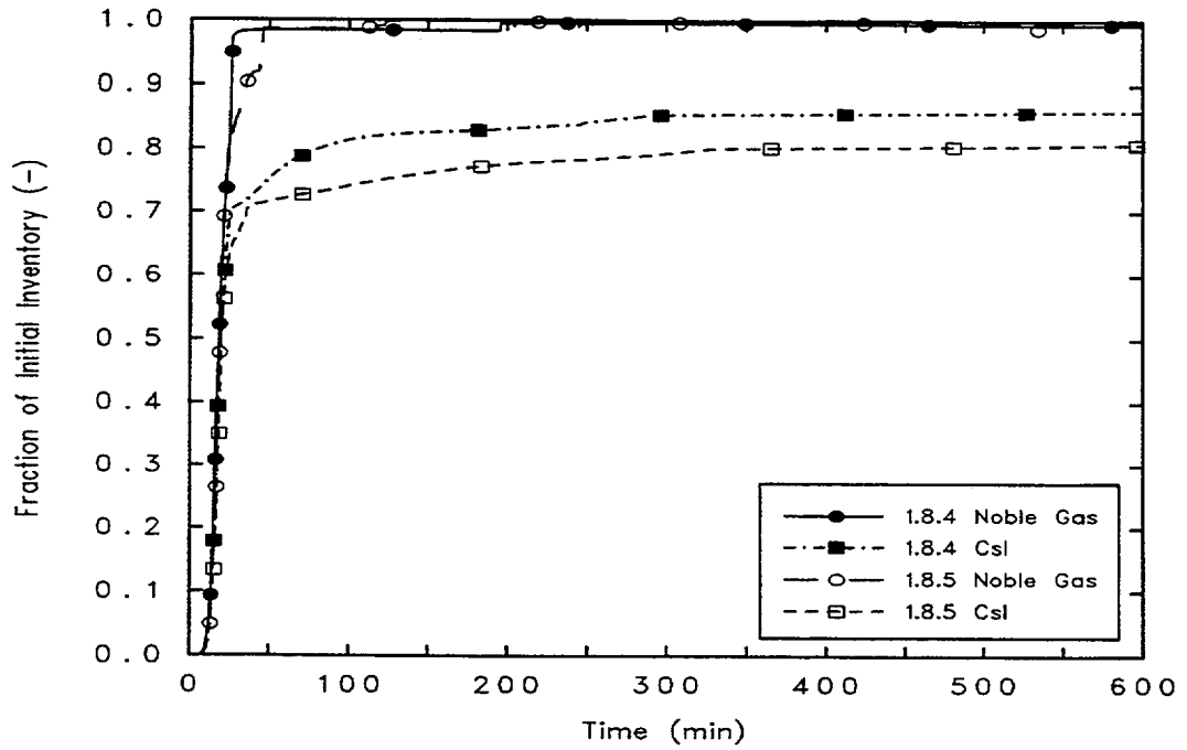
Figure 8-14. Surry LB LOCA: Noble Gas and Csl Release to Containment
