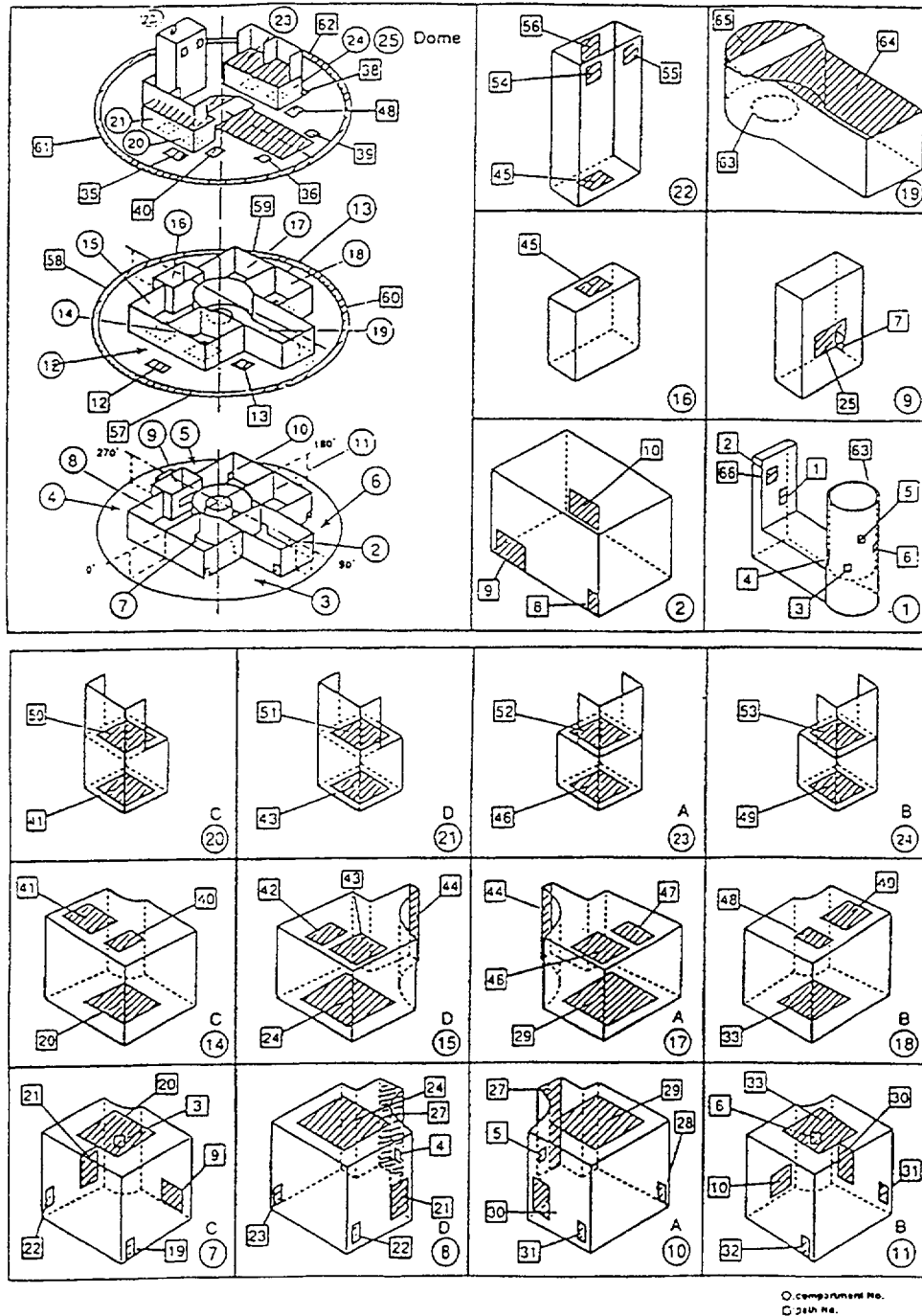
Figure 1-3. Detailed NUPEC Facility Layout [1]
