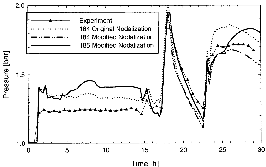
Figure 4-9. Predicted Pressure in the VANAM-M3 Test
