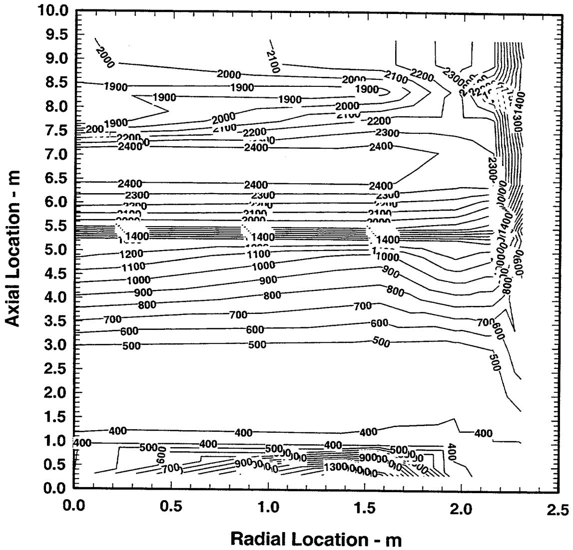
Figure 11-27. Core Temperature Profile at 1500 Seconds
