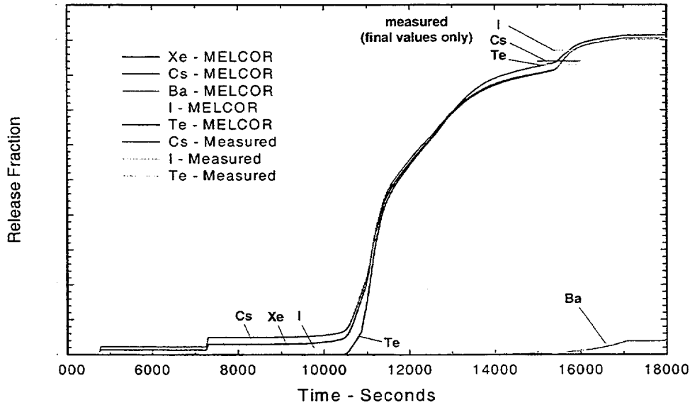
Figure 7-7. Comparison of Calculated and Measured Fission Product Releases for MELCOR 1.8.5. (Note: Data values not publicly available)
