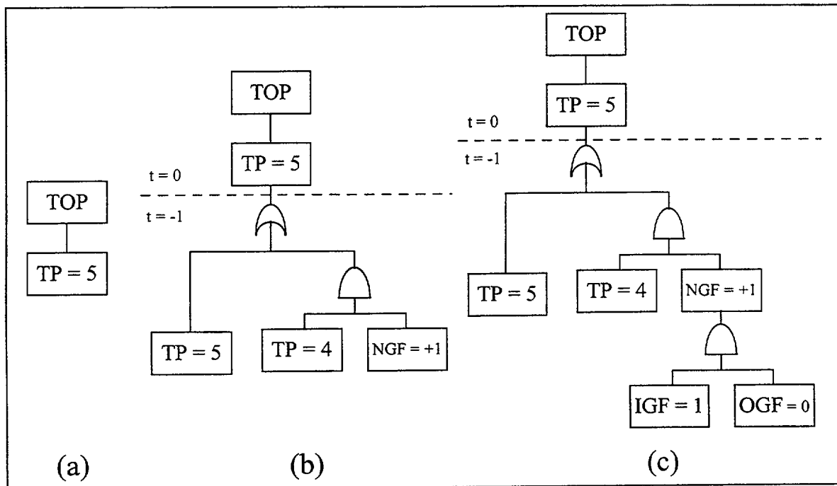
Figure 3.3: Example of timed fault tree construction
