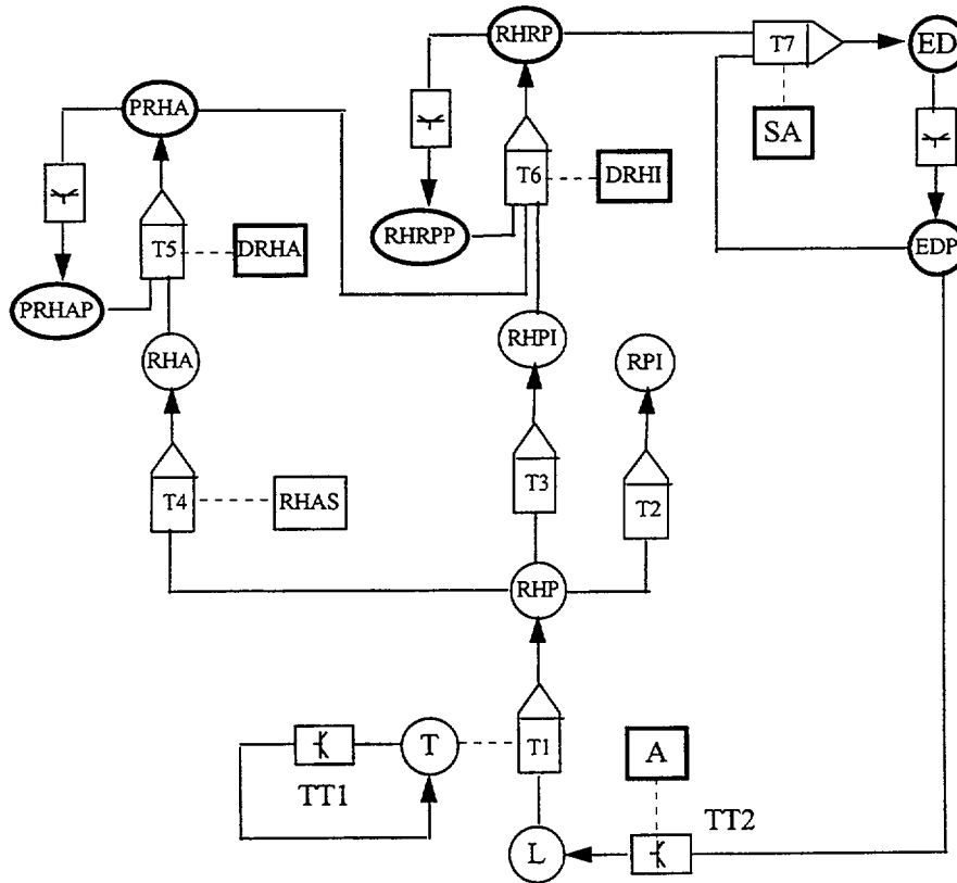
Figure 6.2: DFM model for ISLOCA example
