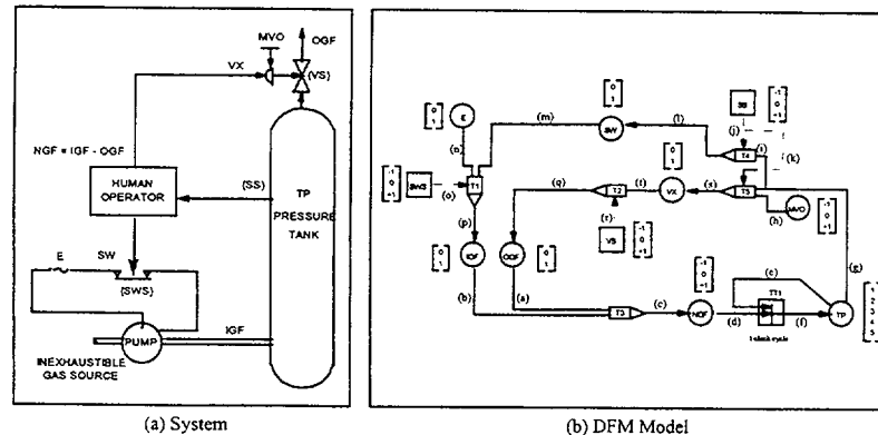
Figure 3.1: A simple system and its DFM model
