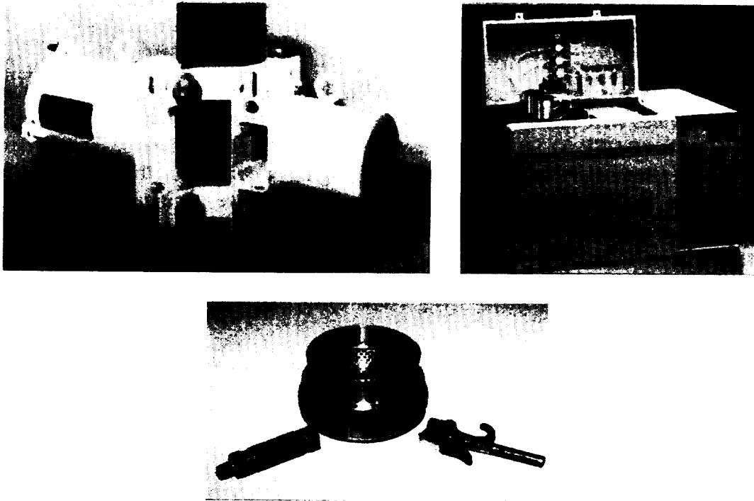
Figure 4.3 10 CFR 31.5 General License. Gas chromatographs, density gauges, and static elimination devices are products used under 10 CFR 31.5 general license.
