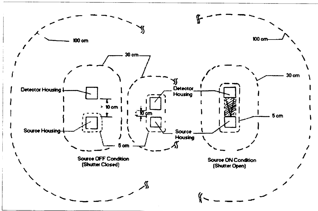
Figure 10.1 Radiation Profiles. ANSI-538 suggests radiation profiles be provided as indicated above.
