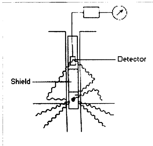
Figure 4.6 Well-Logging Operations. Sealed sources used in well-logging operations must meet the requirements of 10 CFR Part 39.
