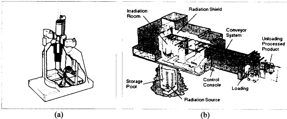
Figure 4.7 Irradiators. NRC evaluates both (a) category I (self-shielded) irradiators and, (b) sealed sources used in category IV (Panoramic, wet source storage) irradiators.
