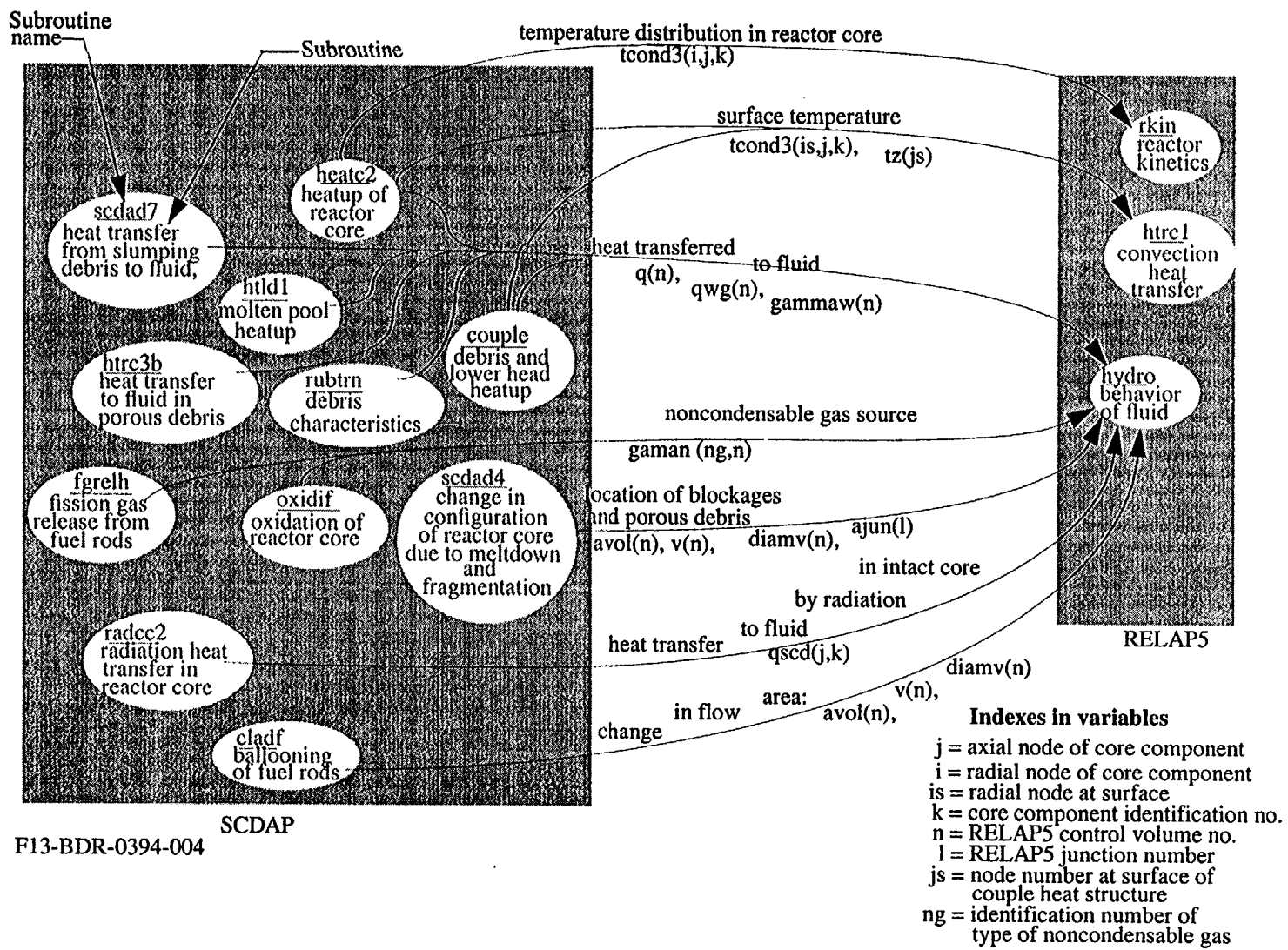
Figure 3-1. Flow of information from SCDAP to RELAP5.
