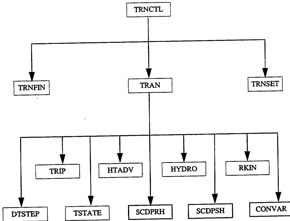
Figure 4-5. SCDAP/RELAP5 top level organization.
