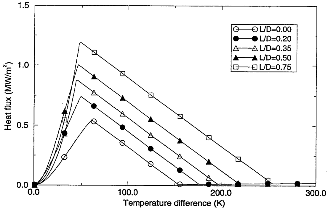
Figure 4-4. Predicted heat flux to a subcooled pool from lower head heat transfer correlations as a function of position and temperature difference. 14, 15
