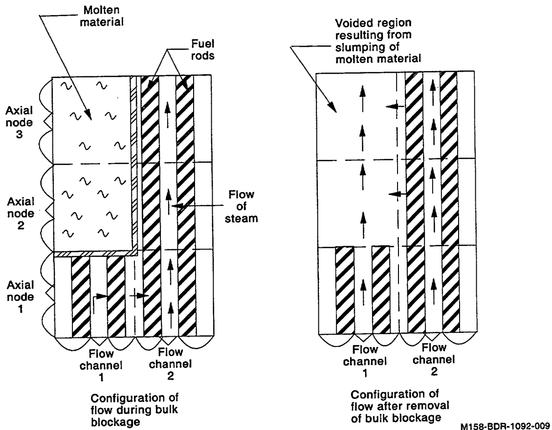
Figure 3-4. Schematic of blockage removal.
