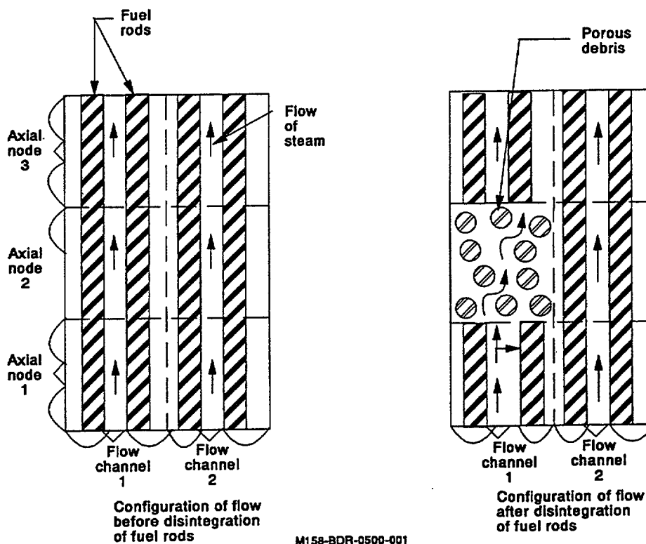
Figure 3-6. Schematic of change in configuration of flow caused by disintegration of fuel rods into porous debris.
