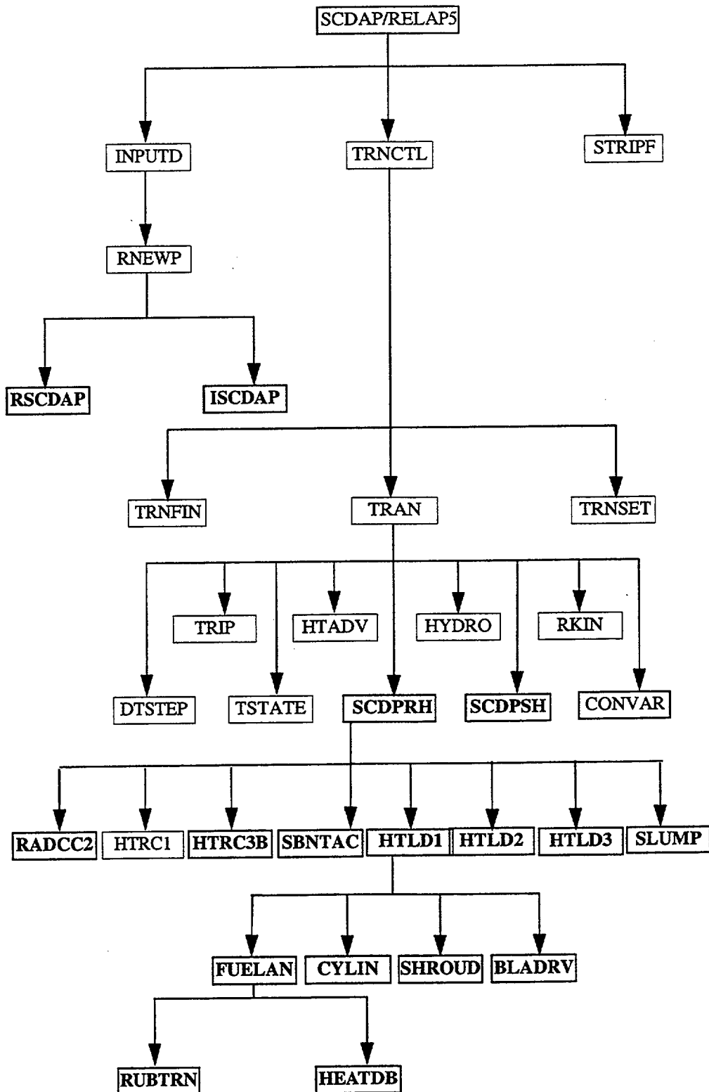
Figure 2-1. SCDAP/RELAP5 architecture with SCDAP specific routines highlighted.
