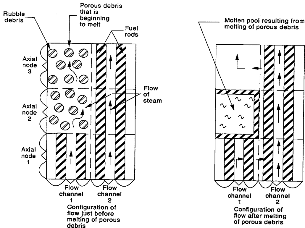
Figure 3-5. Affect of melting of porous debris on flow configuration.
