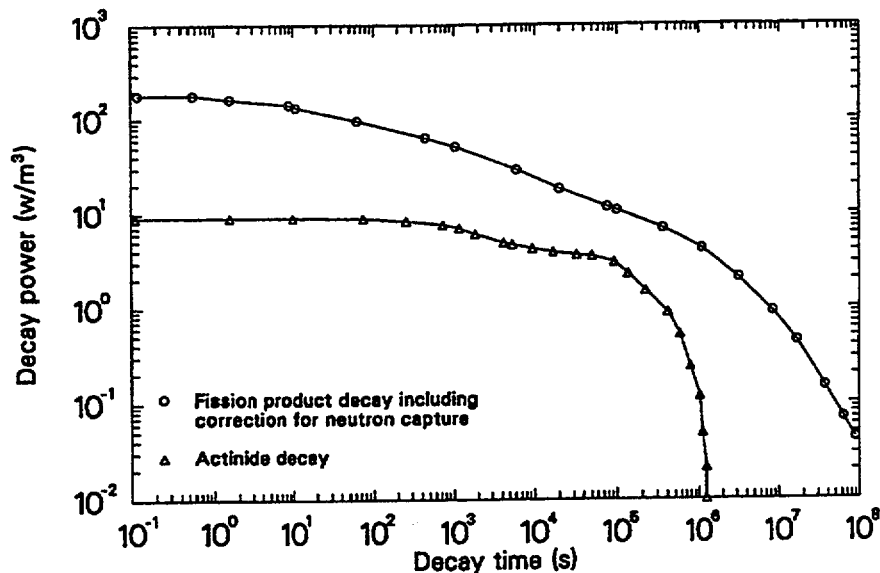
Figure 4-1. Comparison of decay heat components.
