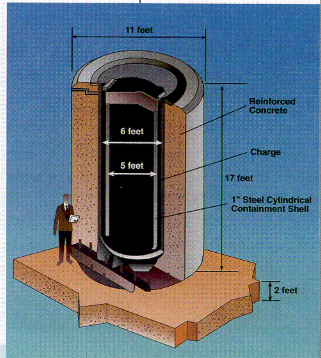
Diagram of a spent fuel storage cask
