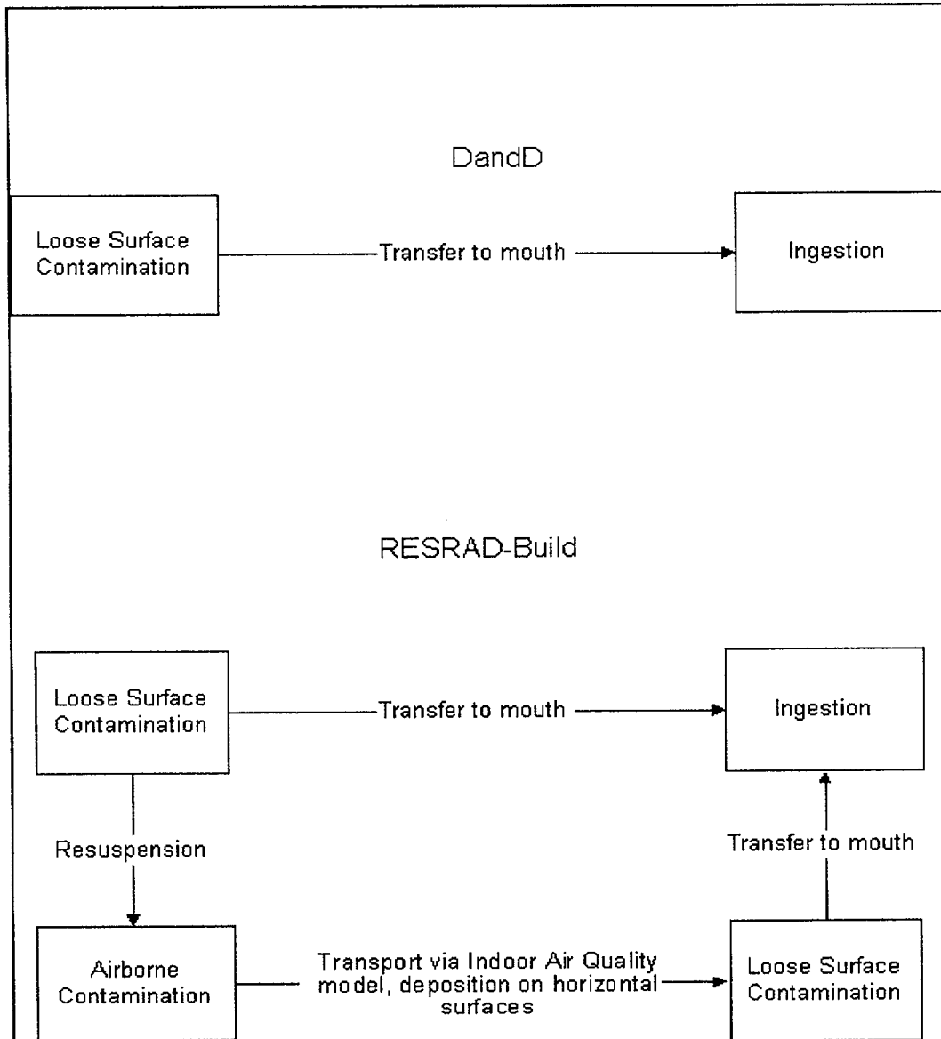
Figure 10. Ingestion models
