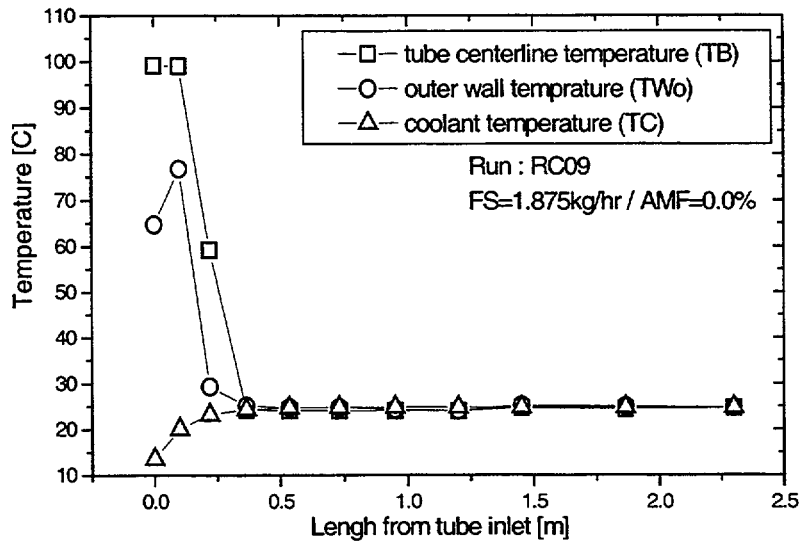
Figure 2.10 Temperature distribution in the absence of air
