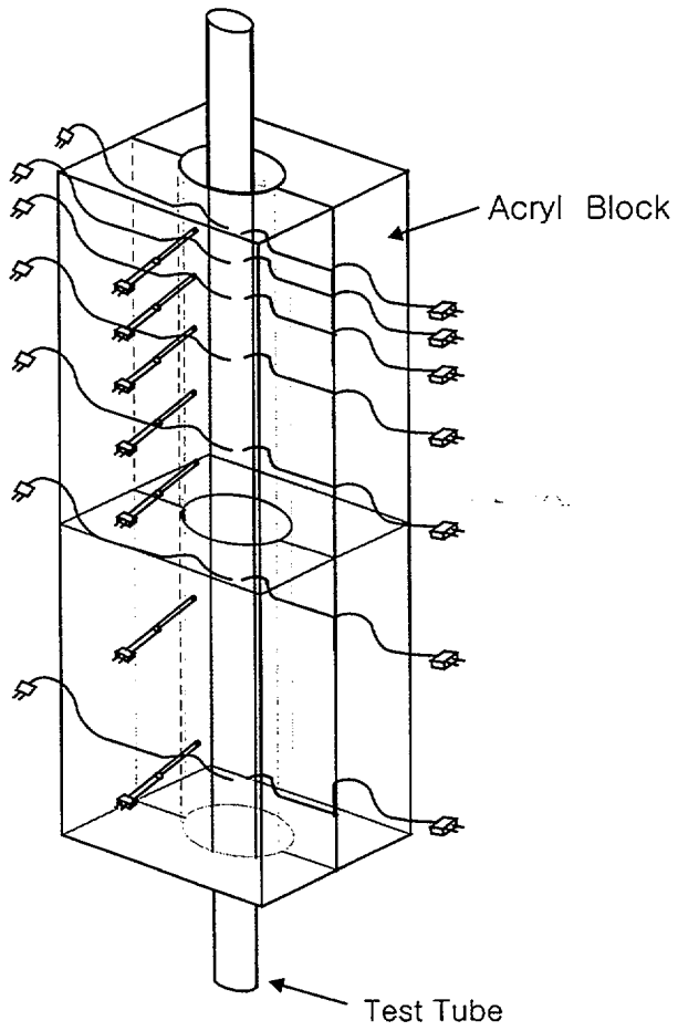
Figure 2.4 Vertical tube and coolant block
