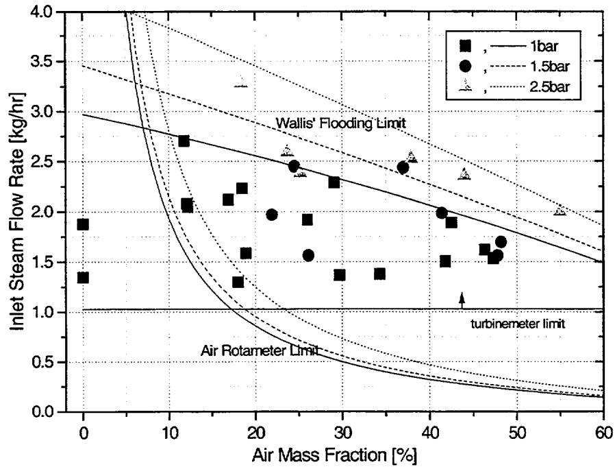
Figure 2.7 Experimental domain in terms of air mass fraction and inlet steam flow rate
