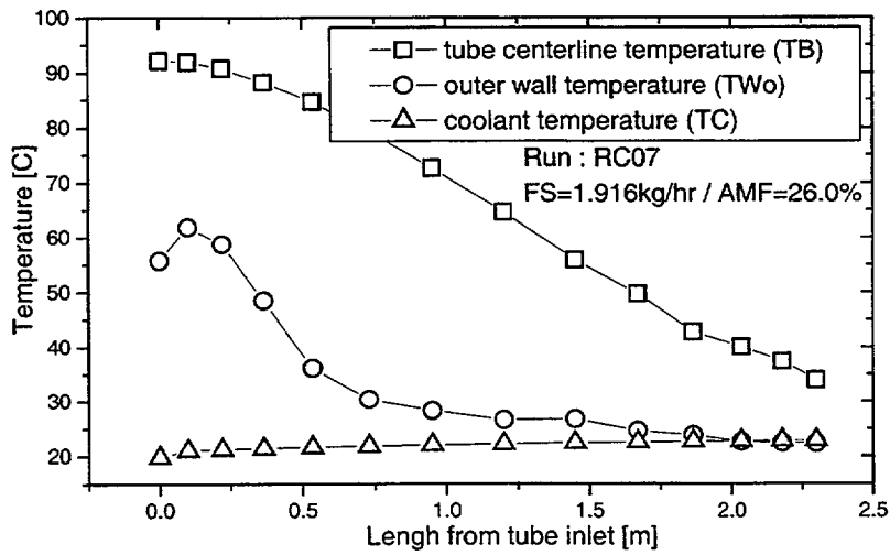
Figure 2.11 Temperature distribution in the presence of air
