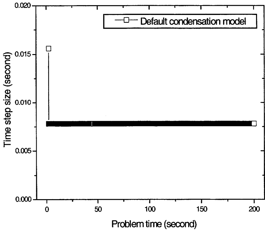
Figure 3.9 Time step sizes of the default condensation model
