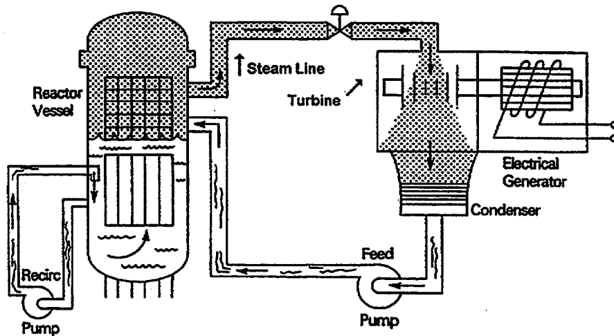
Figure 5.7 Boiling Water Reactor (BWR)
