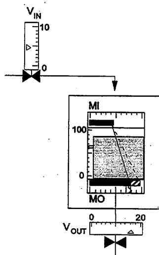
Figure 5.6 EID P+F Interface with Analytical Redundancy (Source: Reprinted with permission from Vicente, K., and Wang, J., "Taking Full Advantage of Process Constraints in Advanced Interface Design," Proceedings of the 1996 American Nuclear Society International Topical Meeting on Nuclear Power Plant Instrumentation, Control and Human-Machine Interface Technologies , pp. 405-411, 1996. Copyright 1996 by the American Nuclear Society. All rights reserved.)
