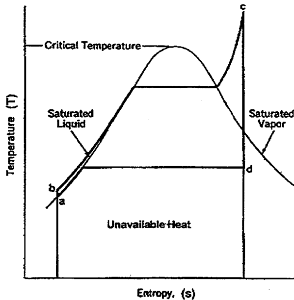
Figure 5.10 Rankine Cycle
