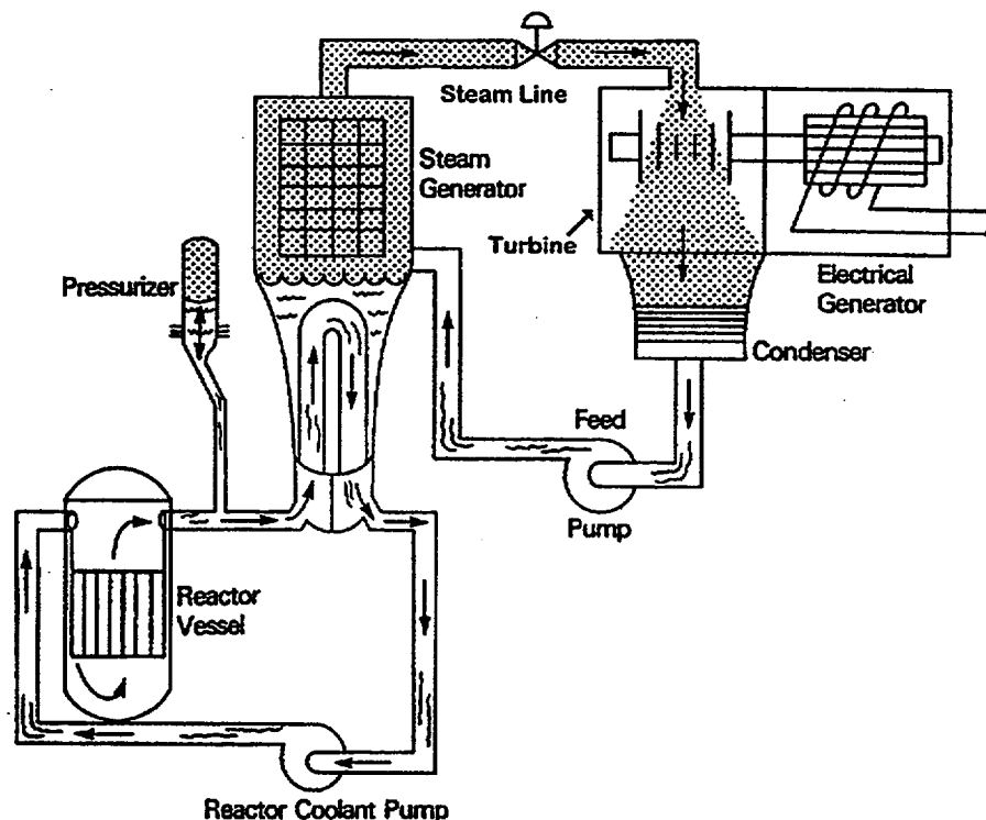
Figure 5.8 Pressurized Water Reactor (PWR)
