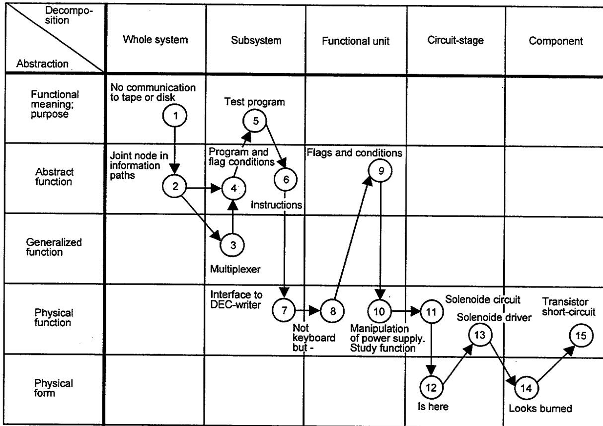
Figure 5.2 Diagnostic Strategies Used in Troubleshooting
